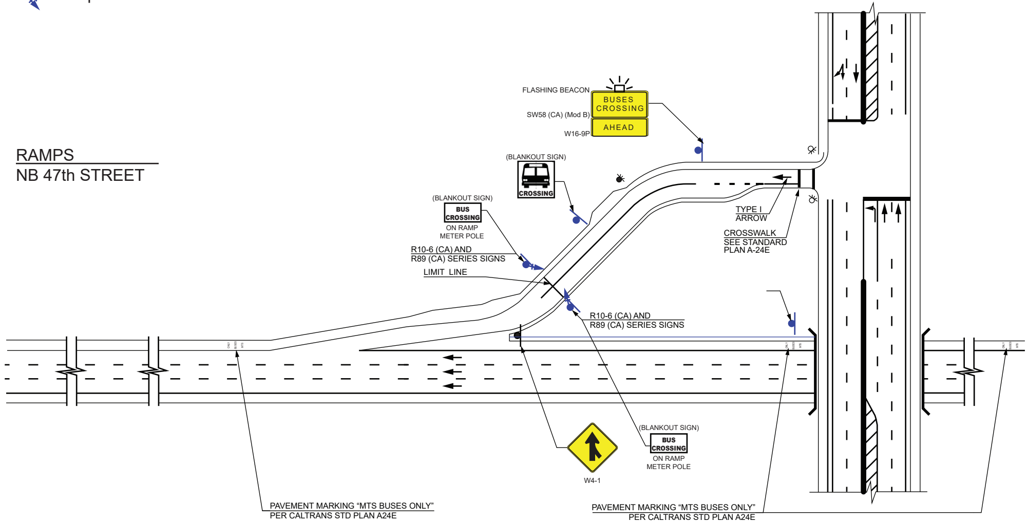
PROPOSED TYPICAL SIGNING AND PAVEMENT MARKING BASED ON FIGURE 3-2 OF CALTRANS RAMP METER DESIGN MANUAL
