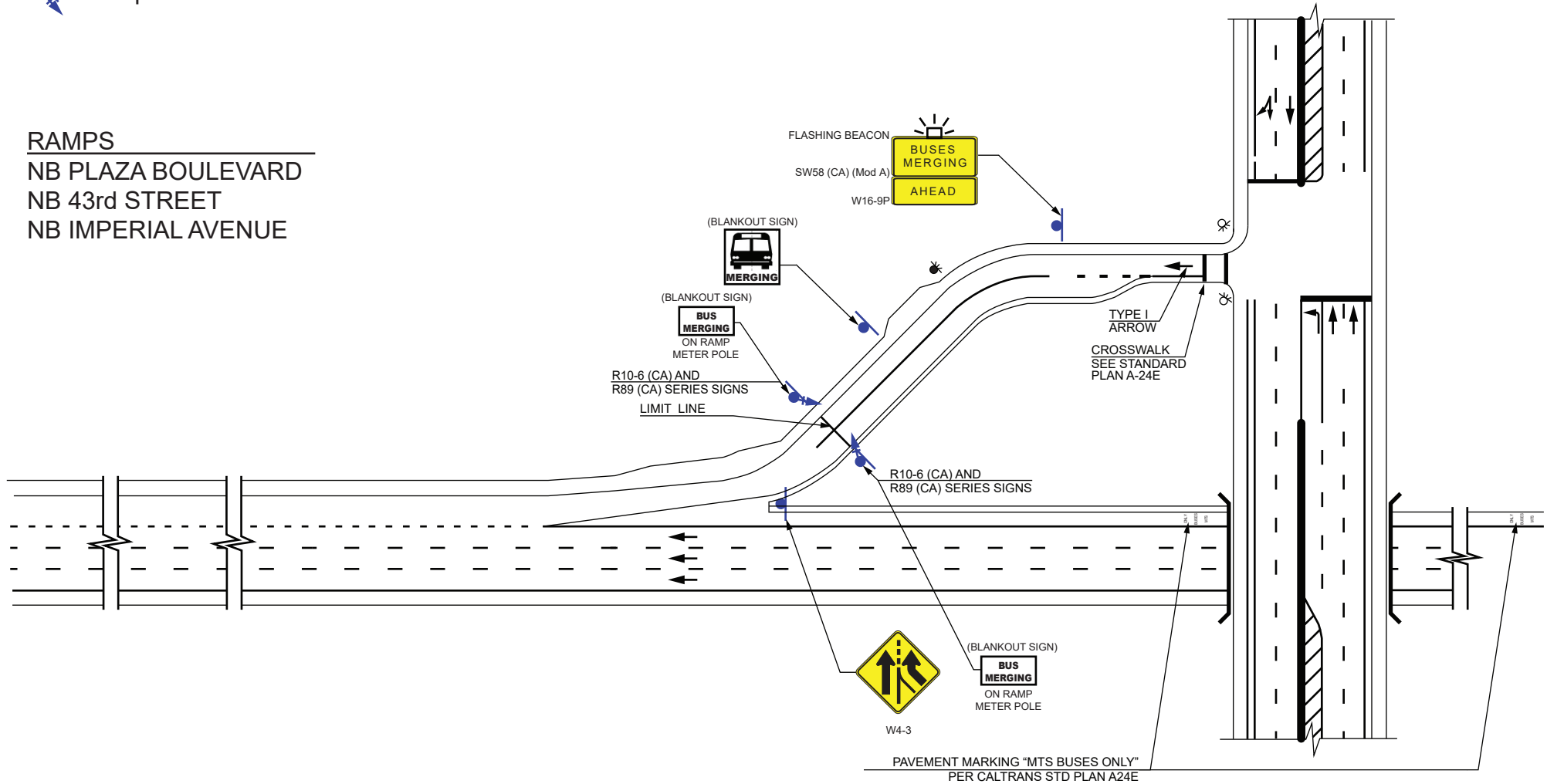
PROPOSED TYPICAL SIGNING AND PAVEMENT MARKING BASED ON FIGURE 3-2 OF CALTRANS RAMP METER DESIGN MANUAL (WITH AUXILIARY LANE)
