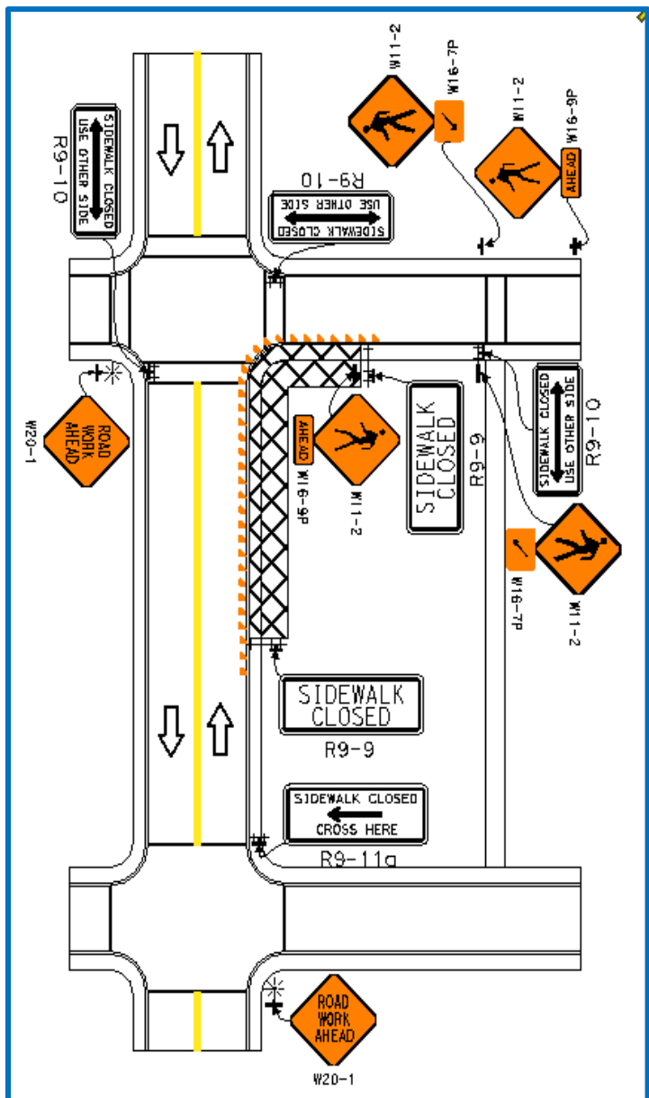
Figure 4 Crosswalk Closures and Pedestrian Detours
