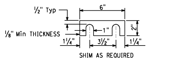
RAILING SHIM DETAILS 3" = 1'-0"
