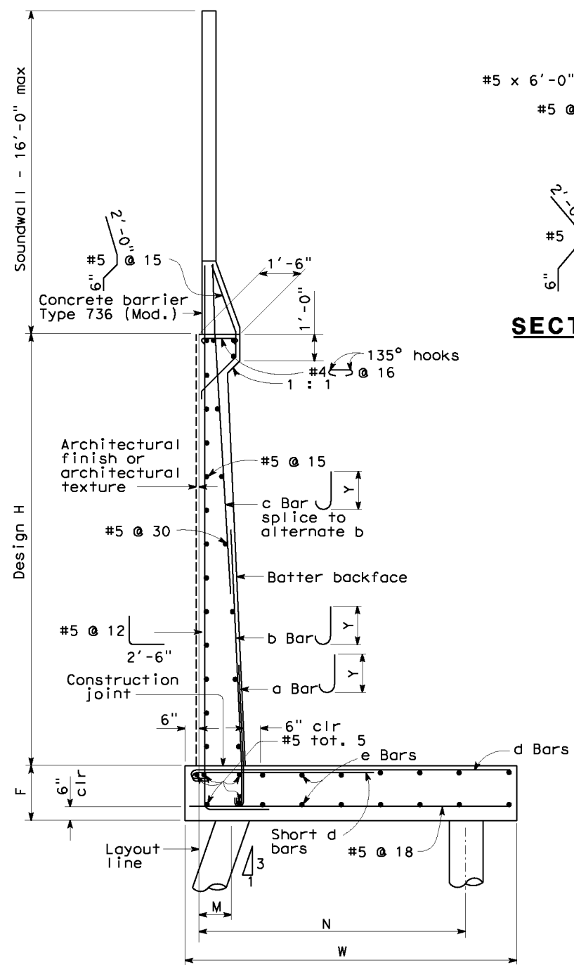
45T PILE FOOTING SECTION NO SCALE
