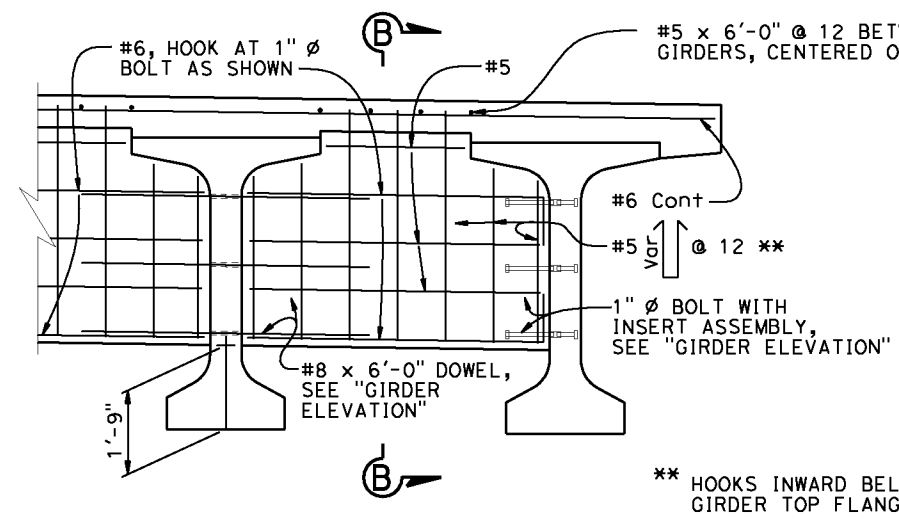
INTERMEDIATE DIAPHRAGM
