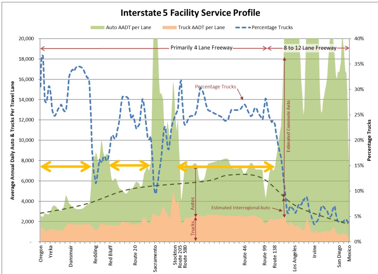
Figure 17: Interstate 5 Facility Service Profile
