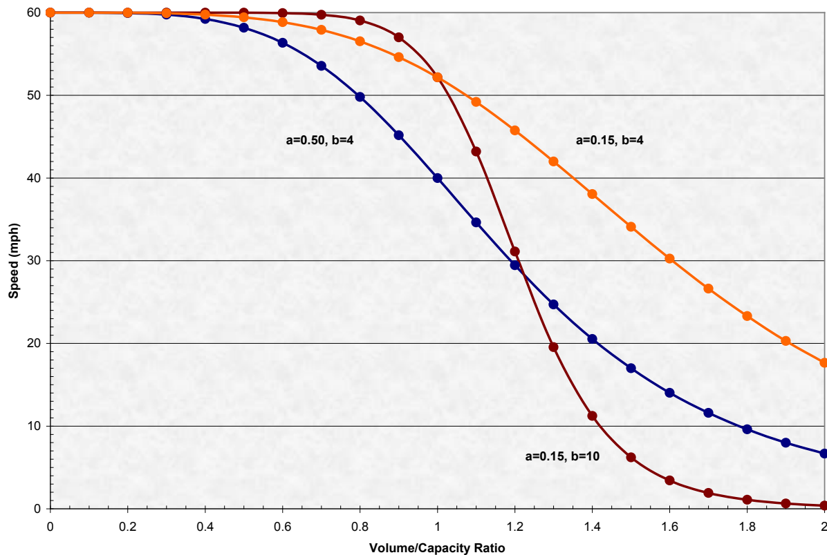
Exhibit III-8: Plot of BPR Curve and Several Variations
