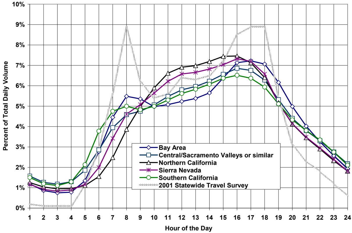
Exhibit III-16: Percent Daily “Rural” Freeway Traffic by Hour by Region
