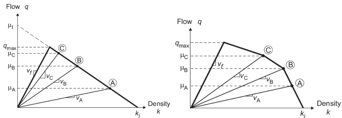
Exhibit VII-6: Two Approaches to Modeling Flow-Density Relationships - Triangular and Piecewise-Linear Concave
