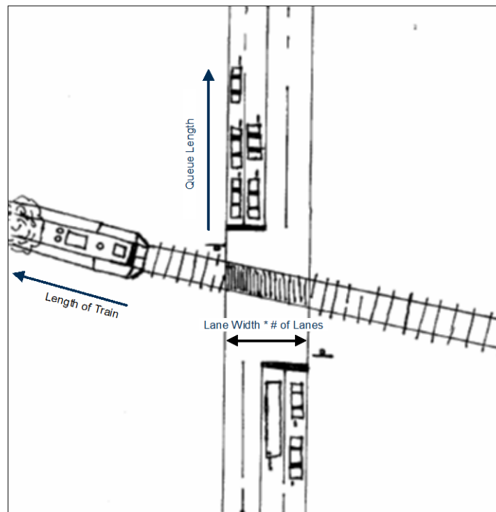
Exhibit VI-1: Typical At-Grade Rail-Highway Crossing
