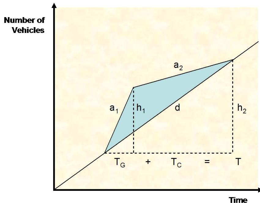
Exhibit VII-7: Input-Output Diagram for Highway Queuing Analysis
