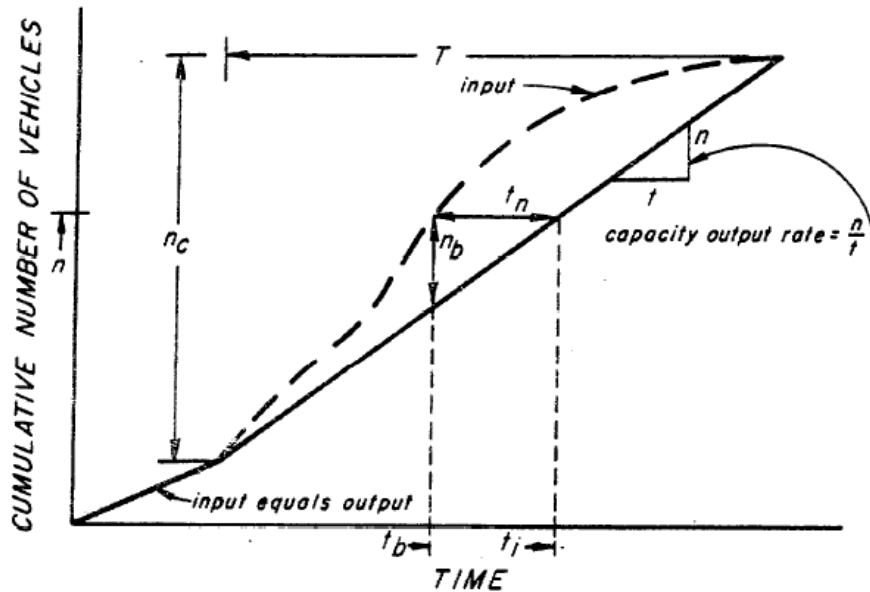
Exhibit VII-4: Queuing Delay for Roadway Grades
