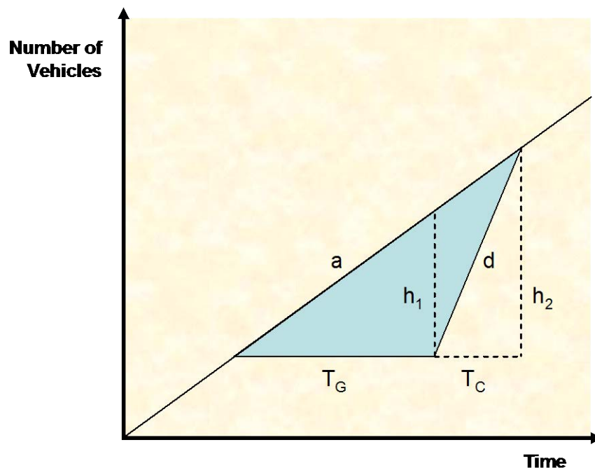
Exhibit VI-5: Input-Output Diagram for Grade Crossing Queuing Analysis
