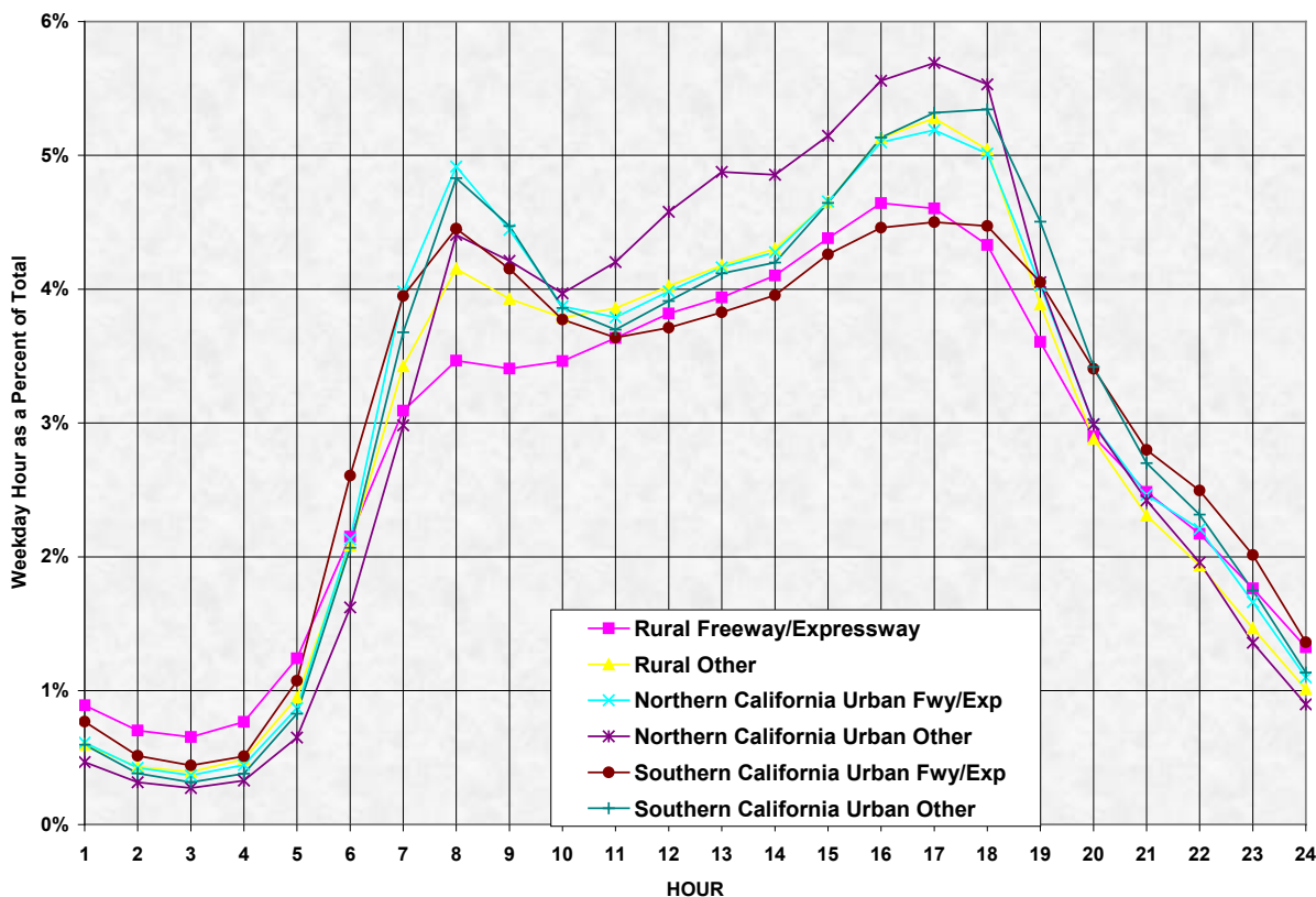
Exhibit III-19: Hourly Weekday Traffic as a Percent of Traffic for a Typical Day
