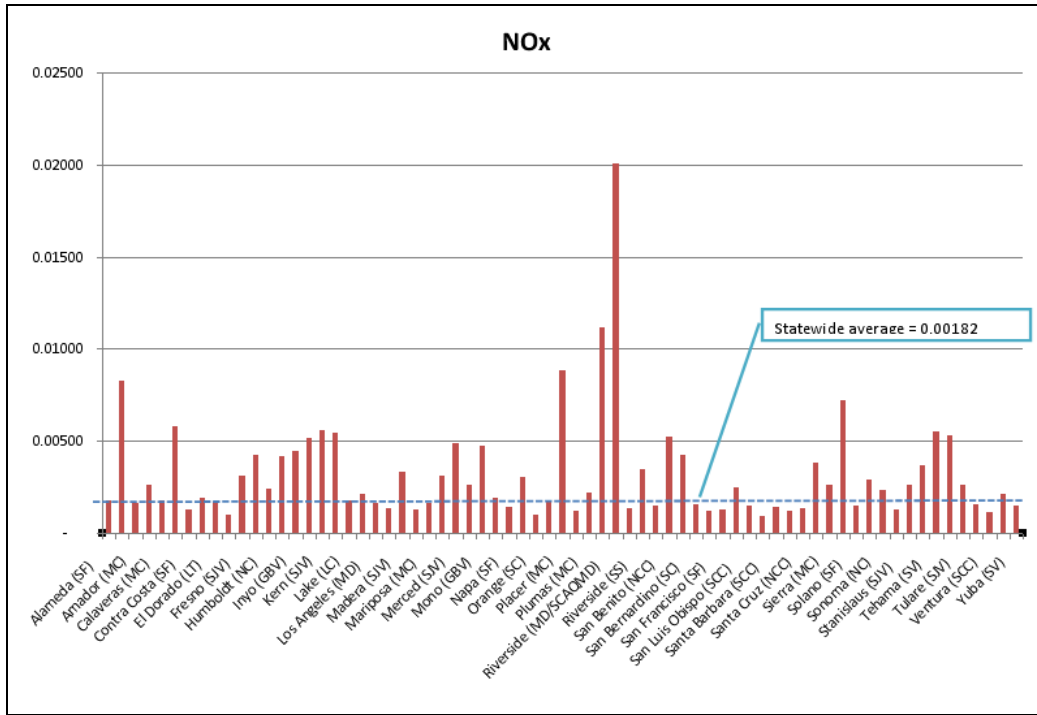
Exhibit III-37: NOx Emissions per Mile
