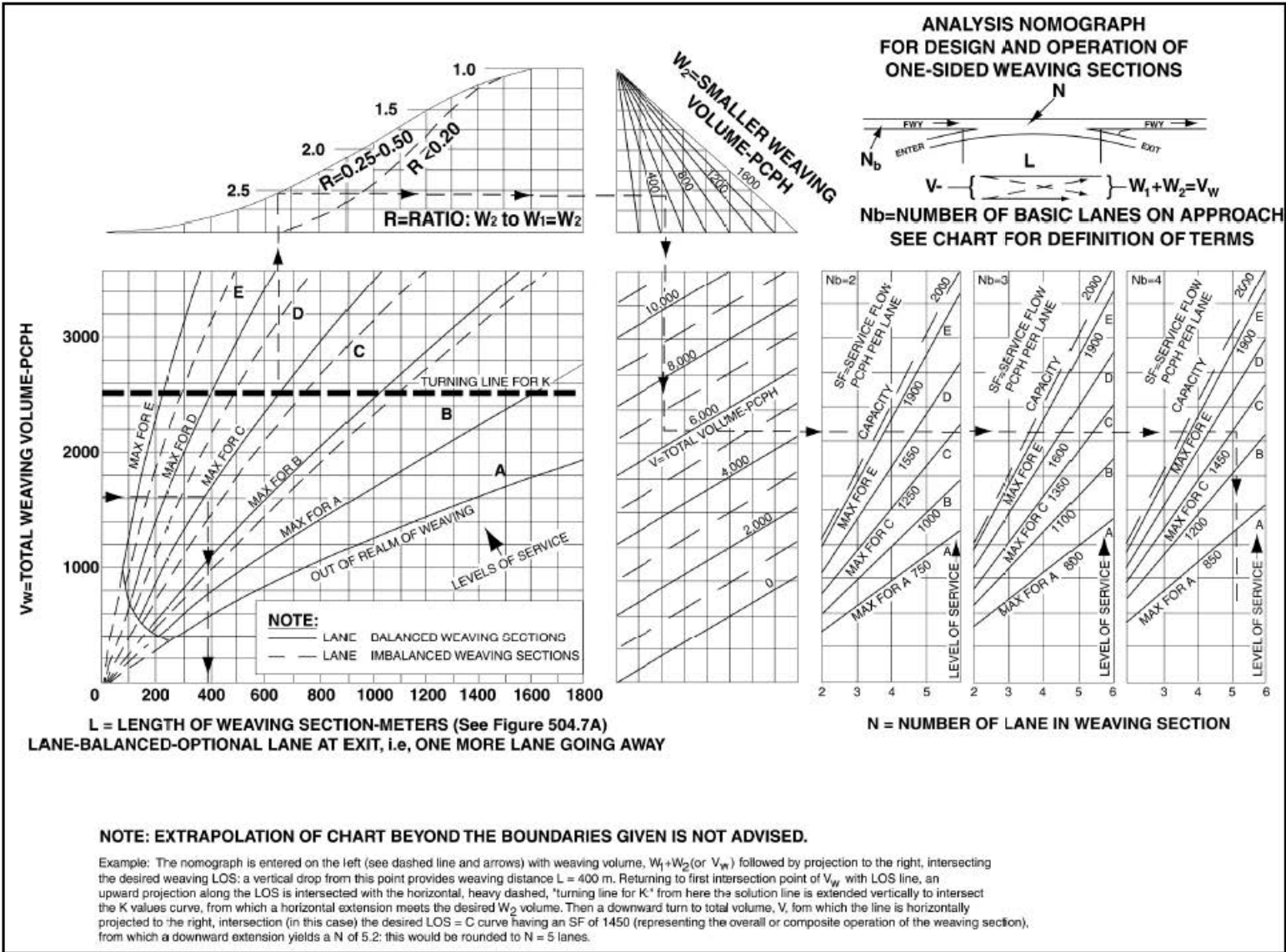
Leisch Design Curve for Freeway and Collector Weaving
