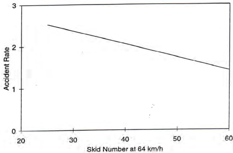
Exhibit VI-9 Linear Relationship Between Accident Rate and Skid Resistance (at a constant speed)
