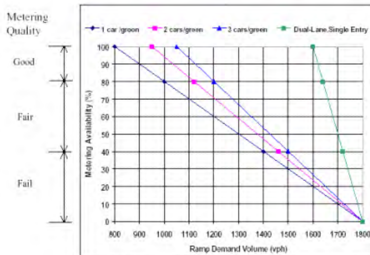
Exhibit II-8 Impact of Ramp Demand on the Quality of Ramp Metering
