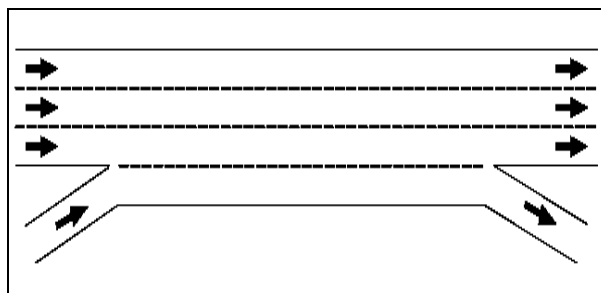
Exhibit V-1 Example of a Simple Ramp-Weave Area
