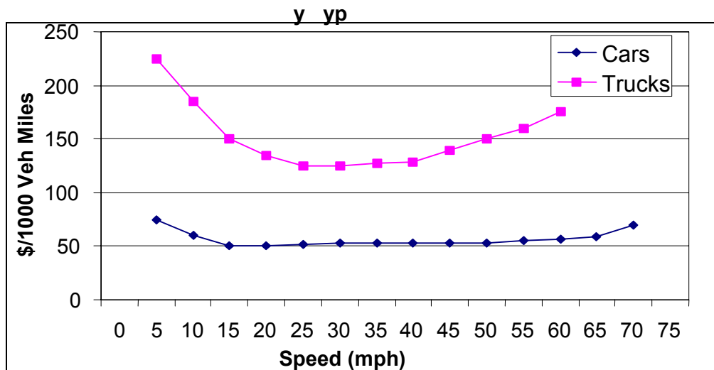
Exhibit VI-14 VOC/Uniform Speed Relationship by Type of Vehicle
