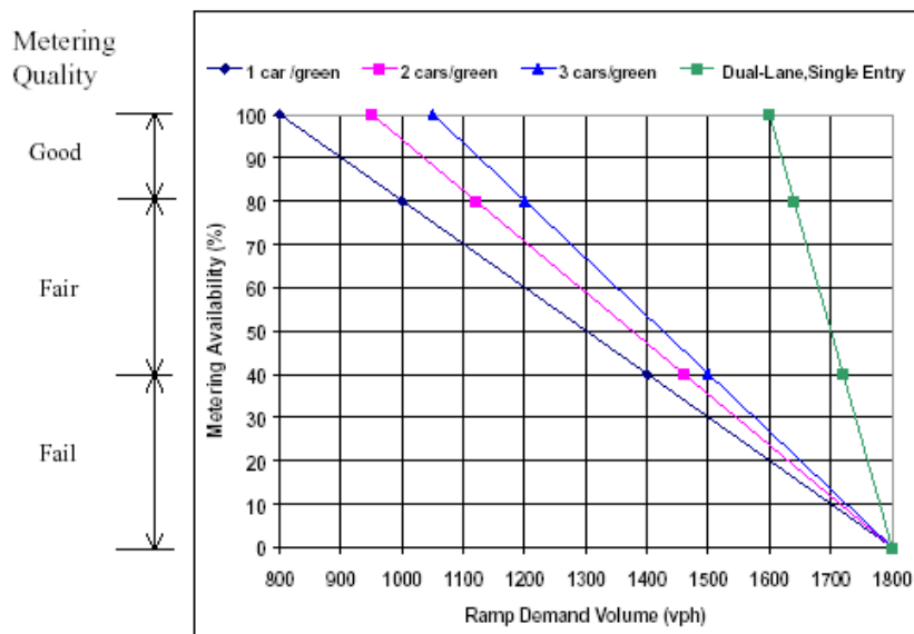
Exhibit V-17 Impact of Ramp Demand on the Quality of Ramp Metering
