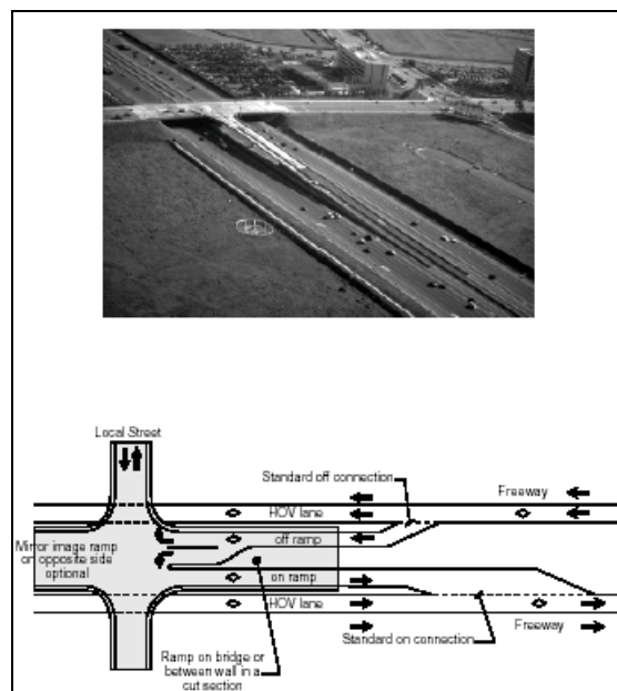
Exhibit V-4 Example of an HOV Drop Ramp
