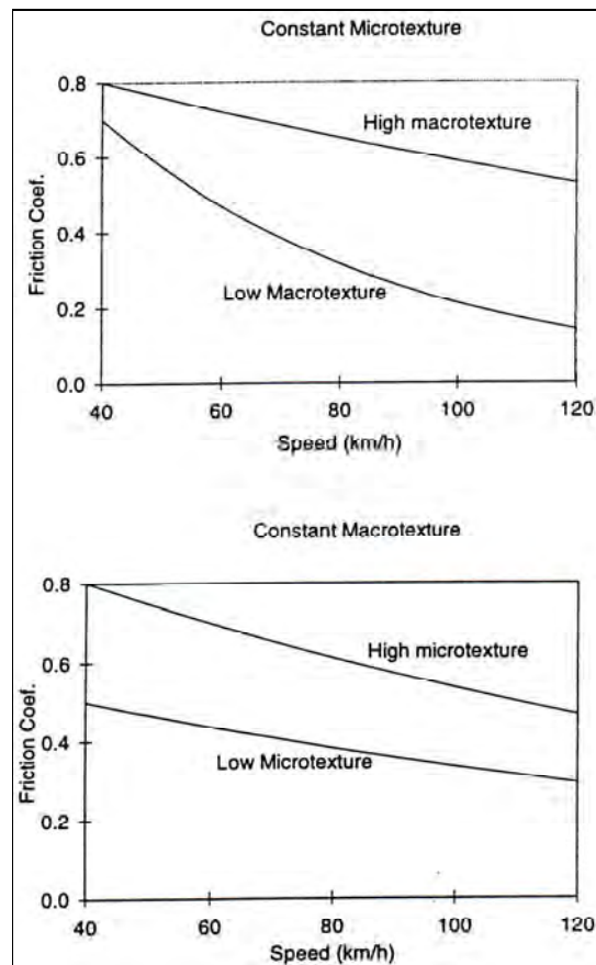
Exhibit VI-8 Effects of Microtexture on Skid Resistance
