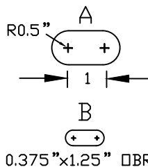
HOLE SLOT DETAIL
