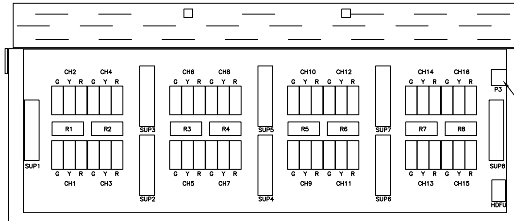
REAR (INSIDE) VIEW
