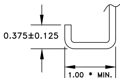
SECTION A-A CABINET HOUSING 1C FLANGE AROUND DOOR OPENING
