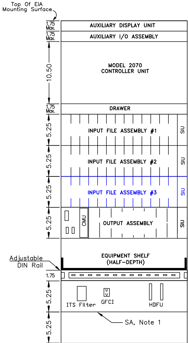
FRONT VIEW (Rack 1)
