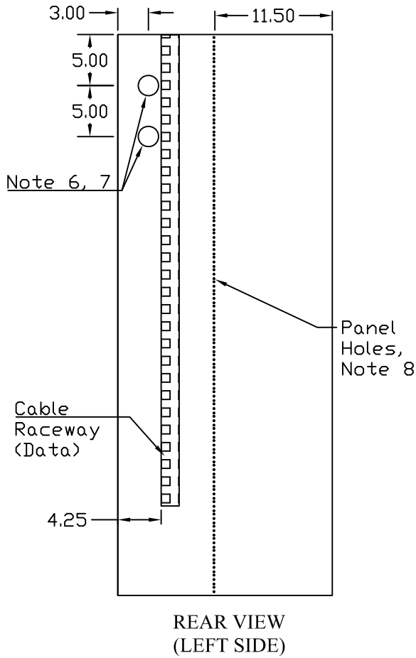
COMMUNICATIONS PANEL #1
