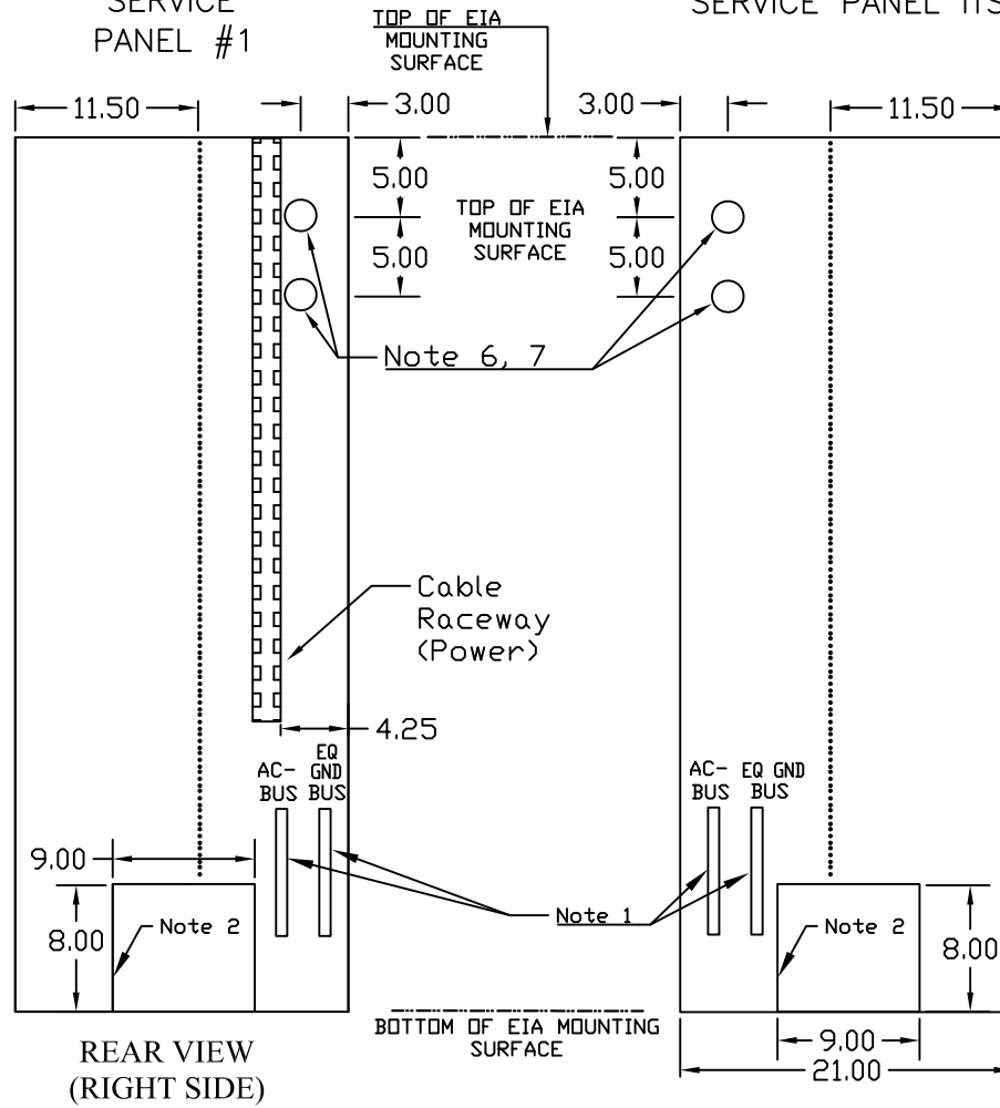
SERVICE PANEL ITS
