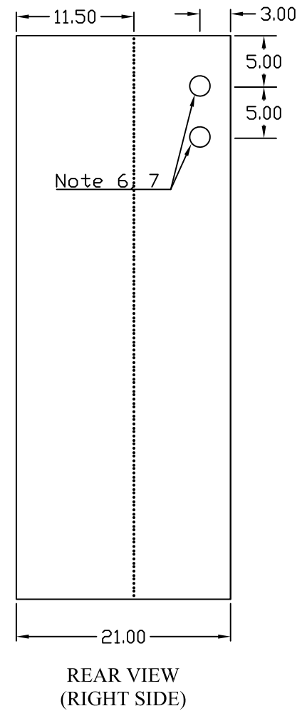
ITS PANEL
