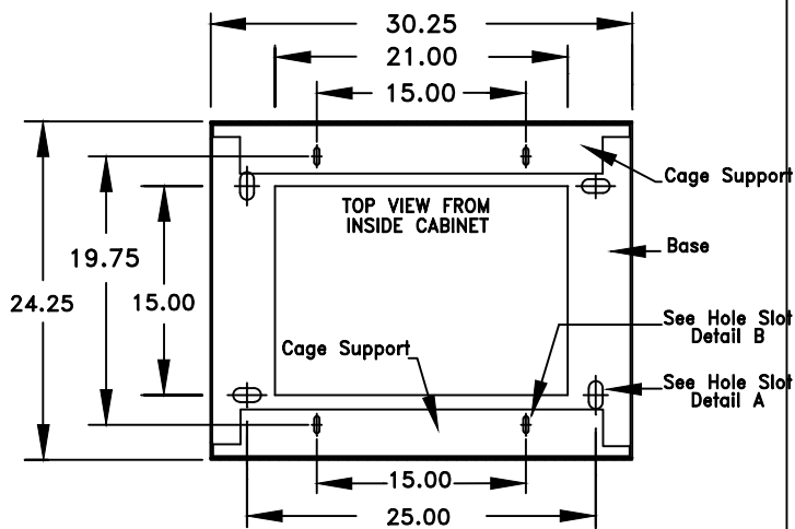
CABINET HOUSING 1C BOTTOM DETAIL
