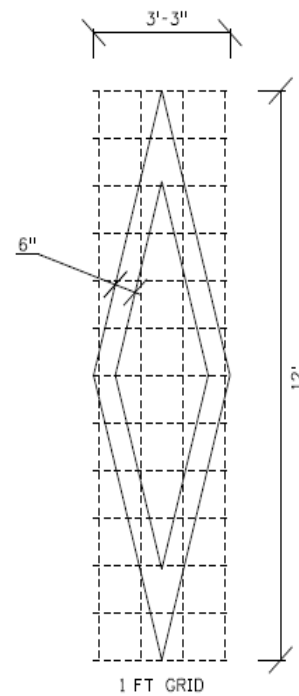
HOV PREFERENTIAL LANE SYMBOL (SEE STANDARD PLANS A24-C)
