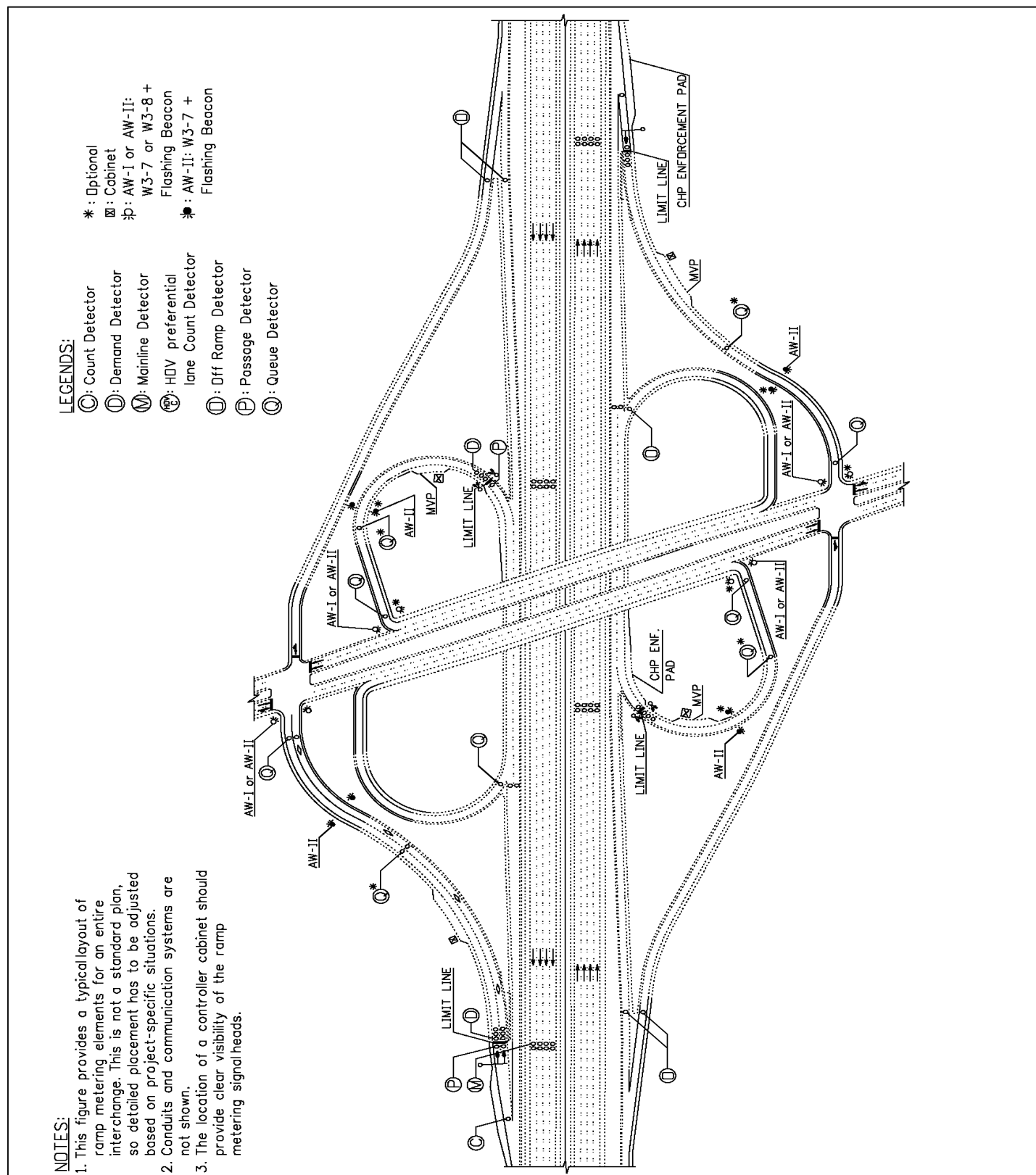
Figure 2-2. Typical Layout of Ramp Metering Elements at a Full-Cloverleaf Interchange
