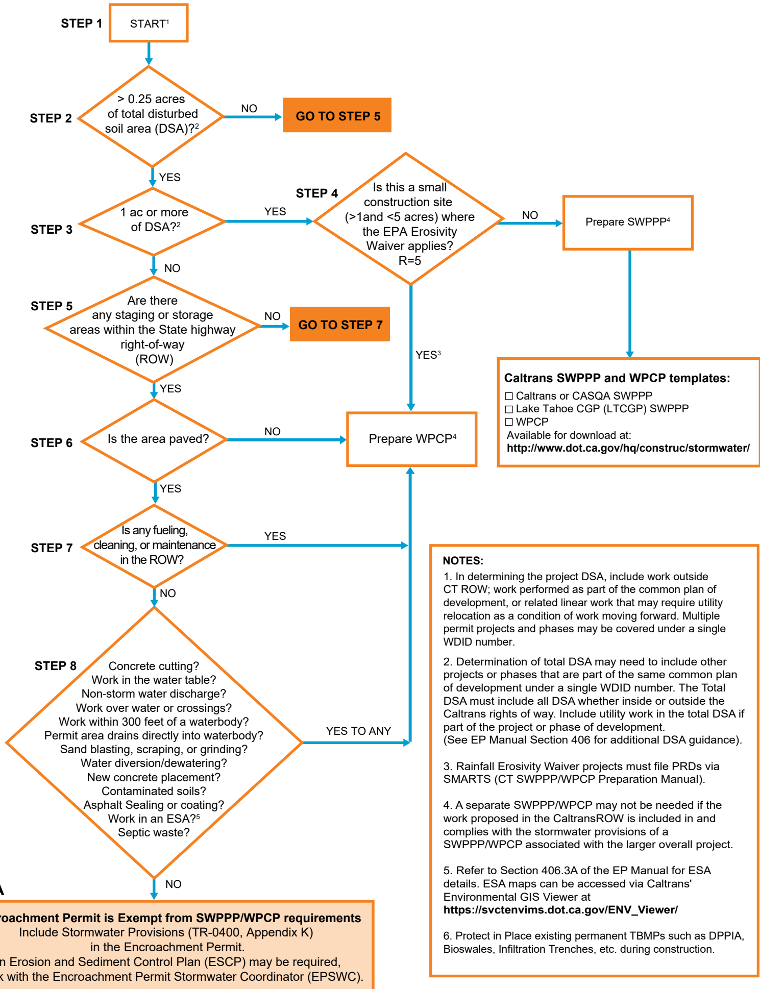
Figure 1. Construction-Related Stormwater Document Determination Flowchart
