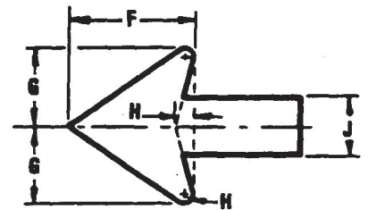
ARROW DETAIL
