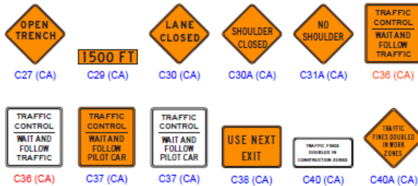
Figure 6F-101(CA). California Temporary Traffic Control Zone Signs (Sheet 1 of 2)
