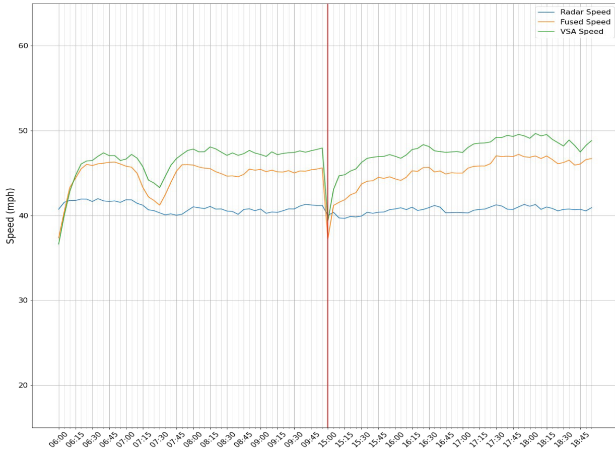
Figure 12. Speed comparison at VSA sign 2 (downstream of Laguna Blvd WB onramp)
