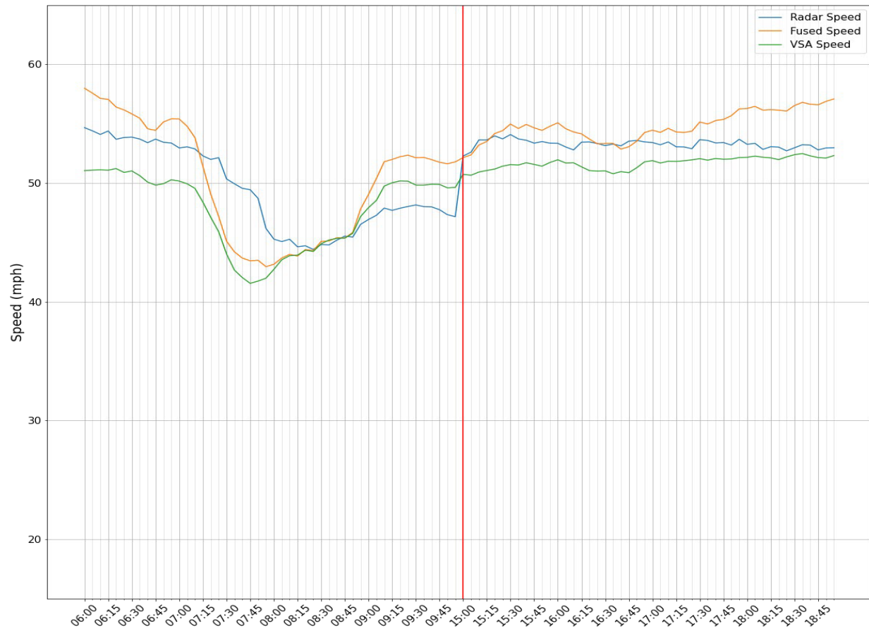
Figure 17. Speed comparison at VSA sign 6 (downstream of Mack Road WB onramp, 2 nd sign)
