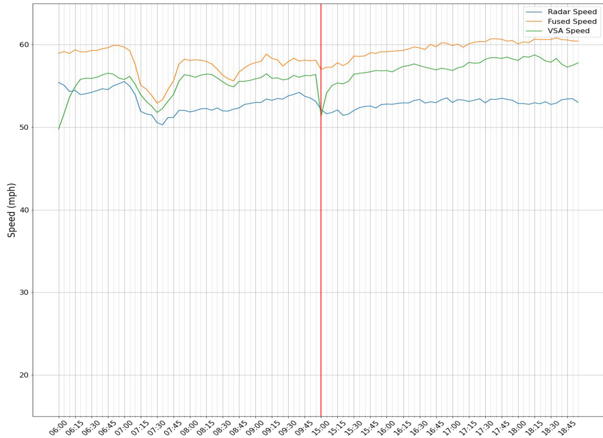
Figure 14. Speed comparison at VSA sign 3 (downstream of Sheldon WB onramp)
