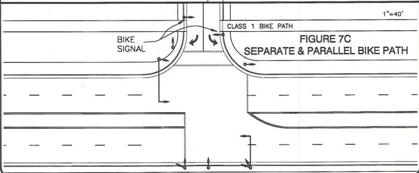
FIGURE 7 - ALTERNATIVE LOCATIONS FOR BICYCLE SIGNALS
