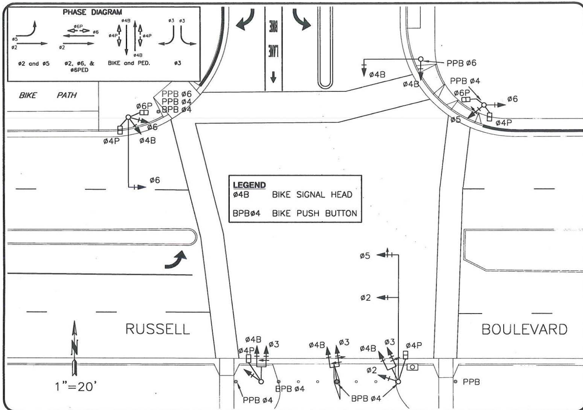
FIGURE 5 - SIGNAL INDICATIONS AND PHASING - AFTER MODIFICATIONS RUSSELL BLVD. AND SYCAMORE LANE
