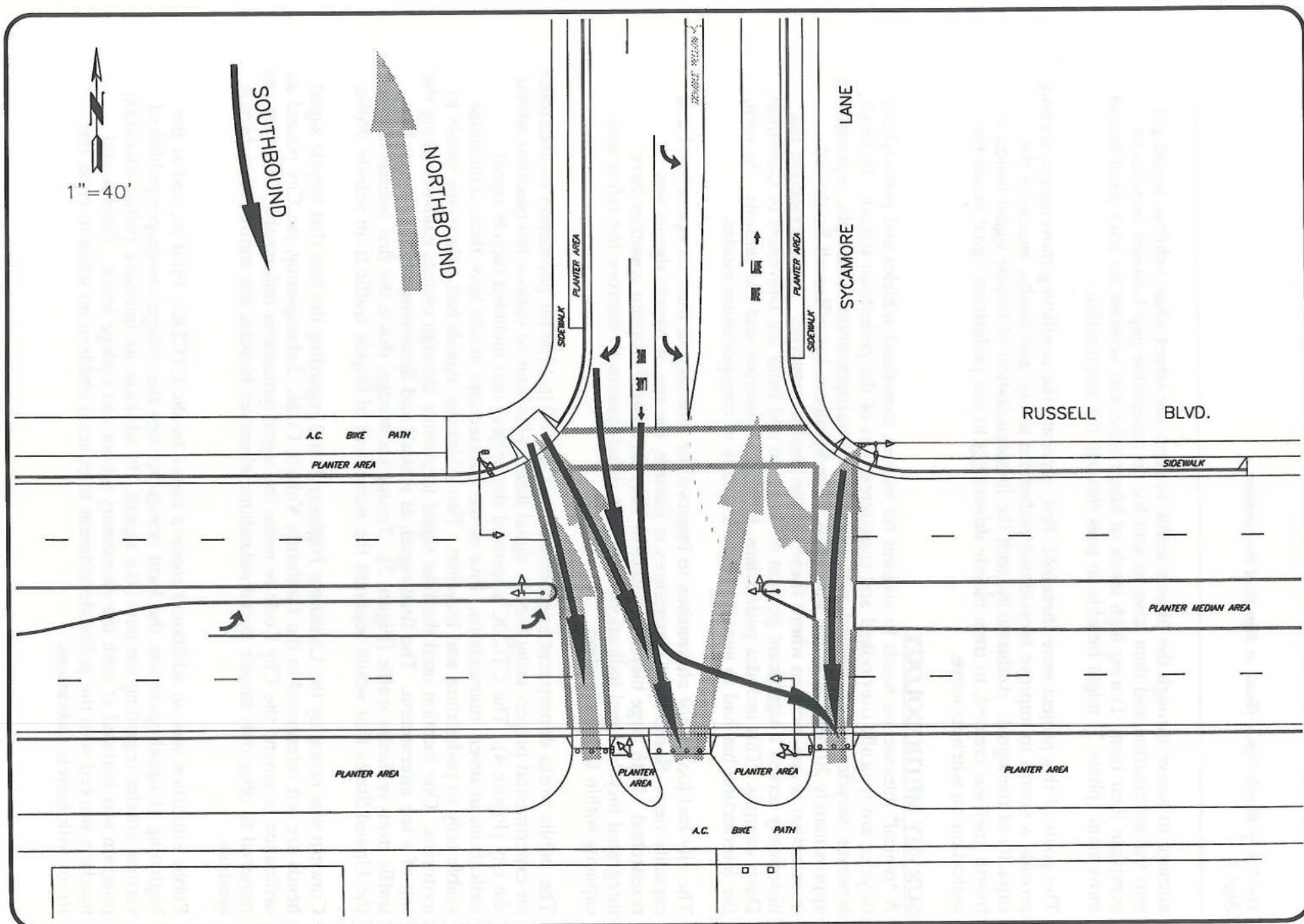
FIGURE 3 - BICYCLE MOVEMENTS PRIOR TO MODIFICATIONS RUSSELL BLVD. & SYCAMORE LANE
