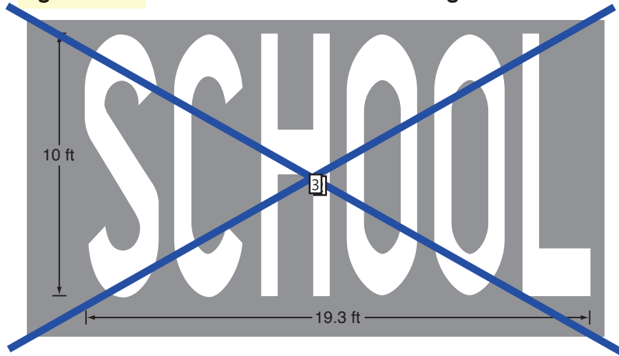
Figure 7C-1. Two-Lane Pavement Marking of “SCHOOL”
