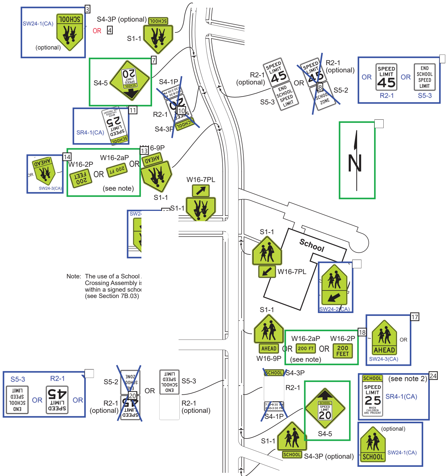
Figure B-2. Example of Signing for a School Zone with a School Speed Limit and a School Crossing
