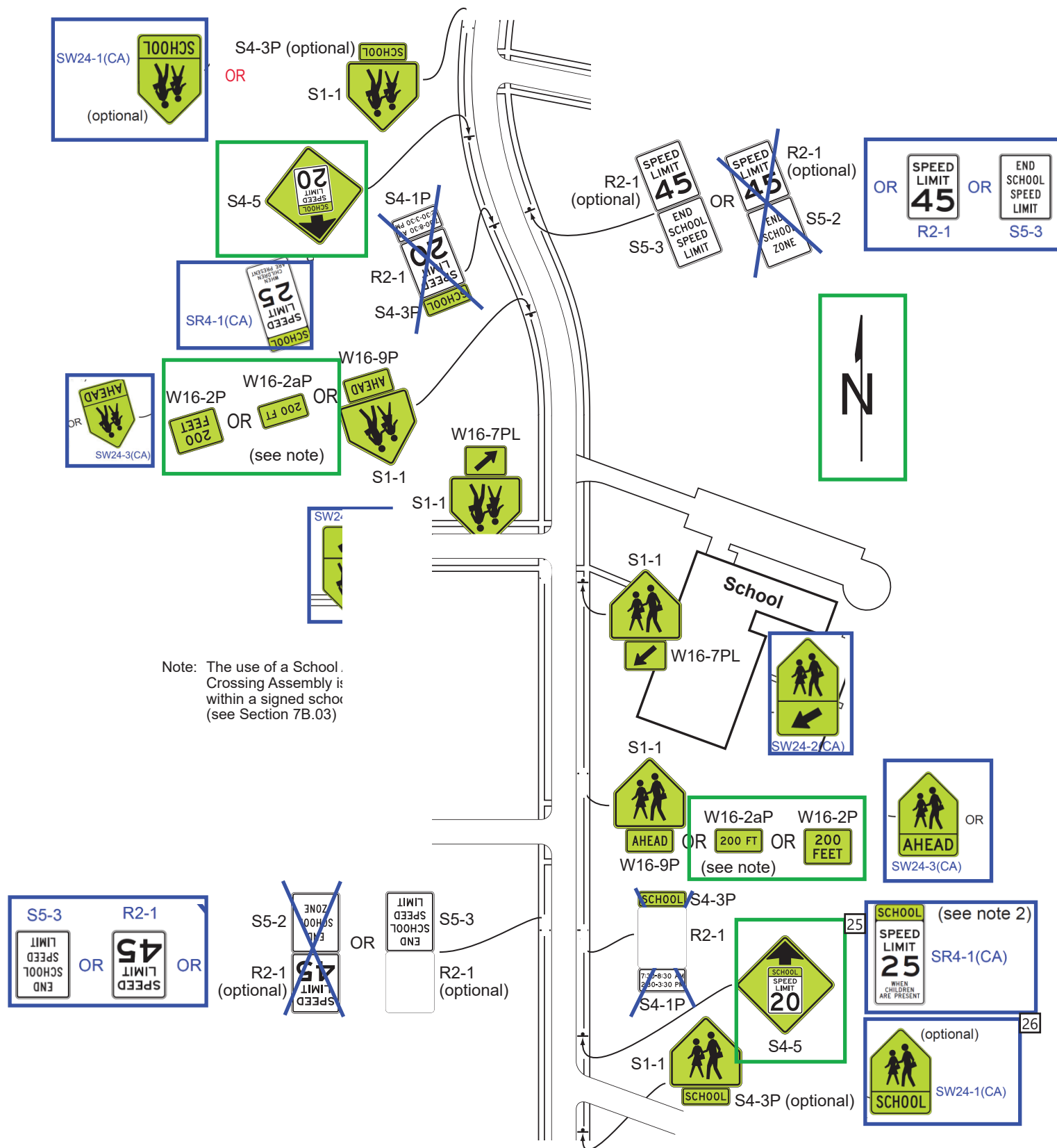
Figure 7B-2. Example of Signing for a School Zone with a School Speed Limit and a School Crossing
