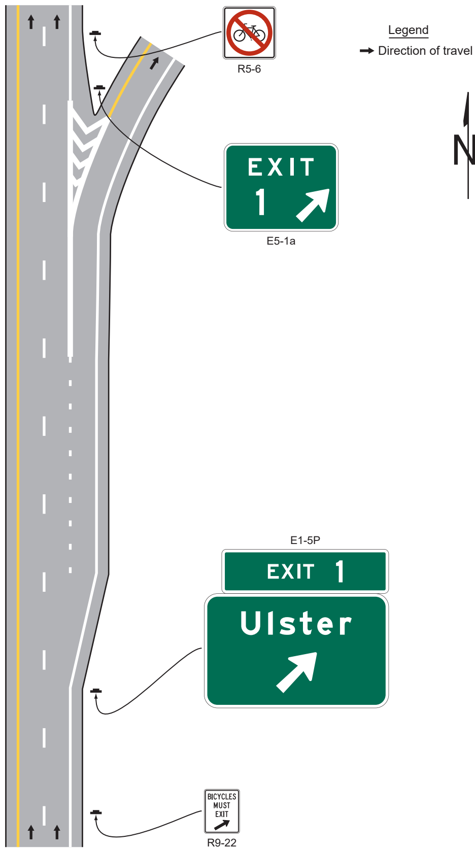
Figure 9B-4. Signing for Termination of Bicycle Access on Freeways and Expressways
