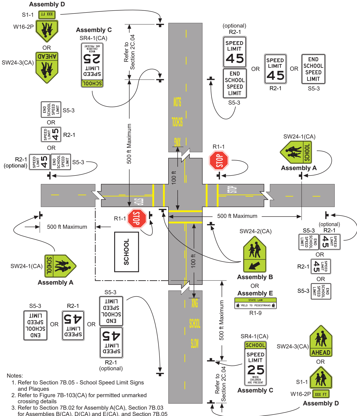
Figure 7B-2(CA). Example of Signing for a School Zone with a School Speed Limit and a School Crossing
