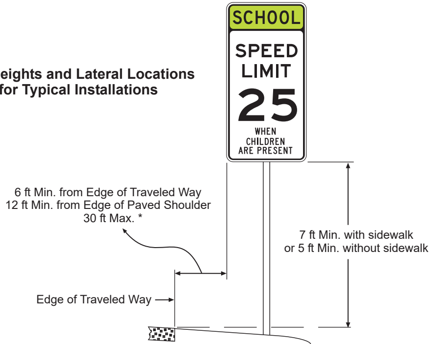
Figure 7B-1(CA). Signs in School Areas and at School Crossings
