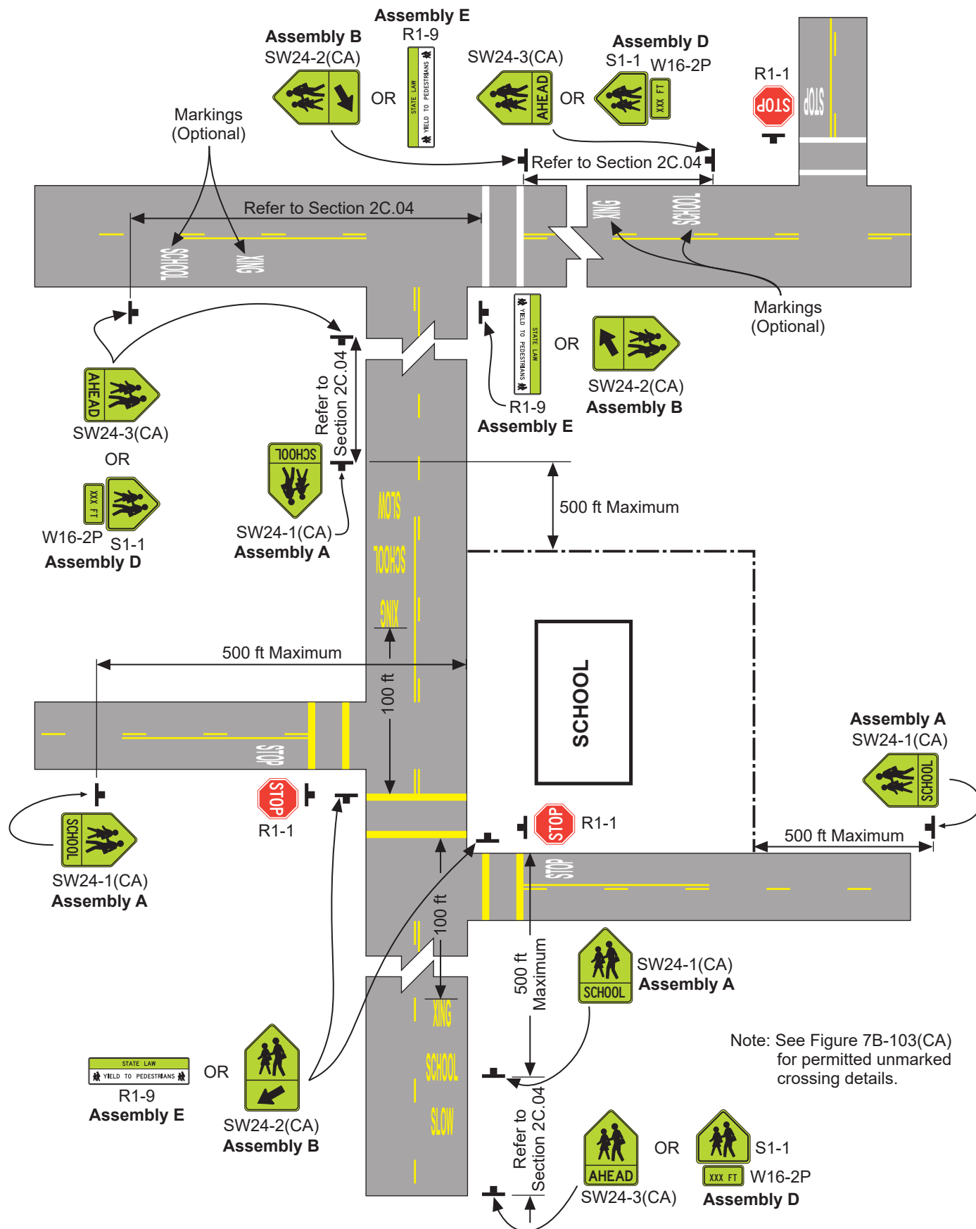
Figure 7B-104(CA). Example of Signing for School Crosswalk Warning Assembly
