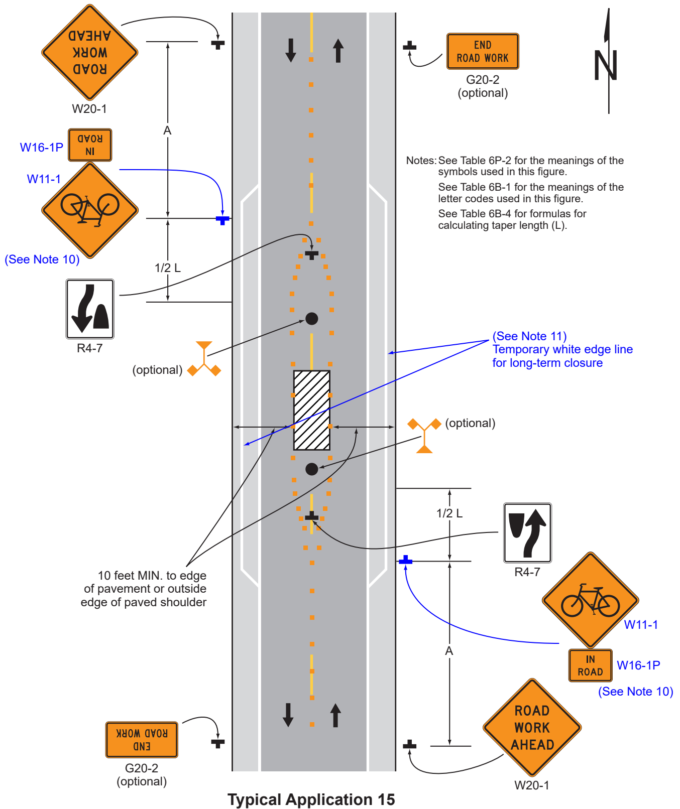
Figure 6P-15. Work in the Center of a Road with Low Traffic Volumes (TA-15)
