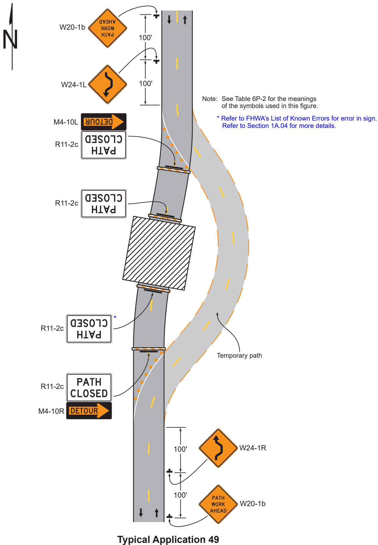
Figure 6P-49. Shared-Use Path Closure with a Diversion (TA-49)
