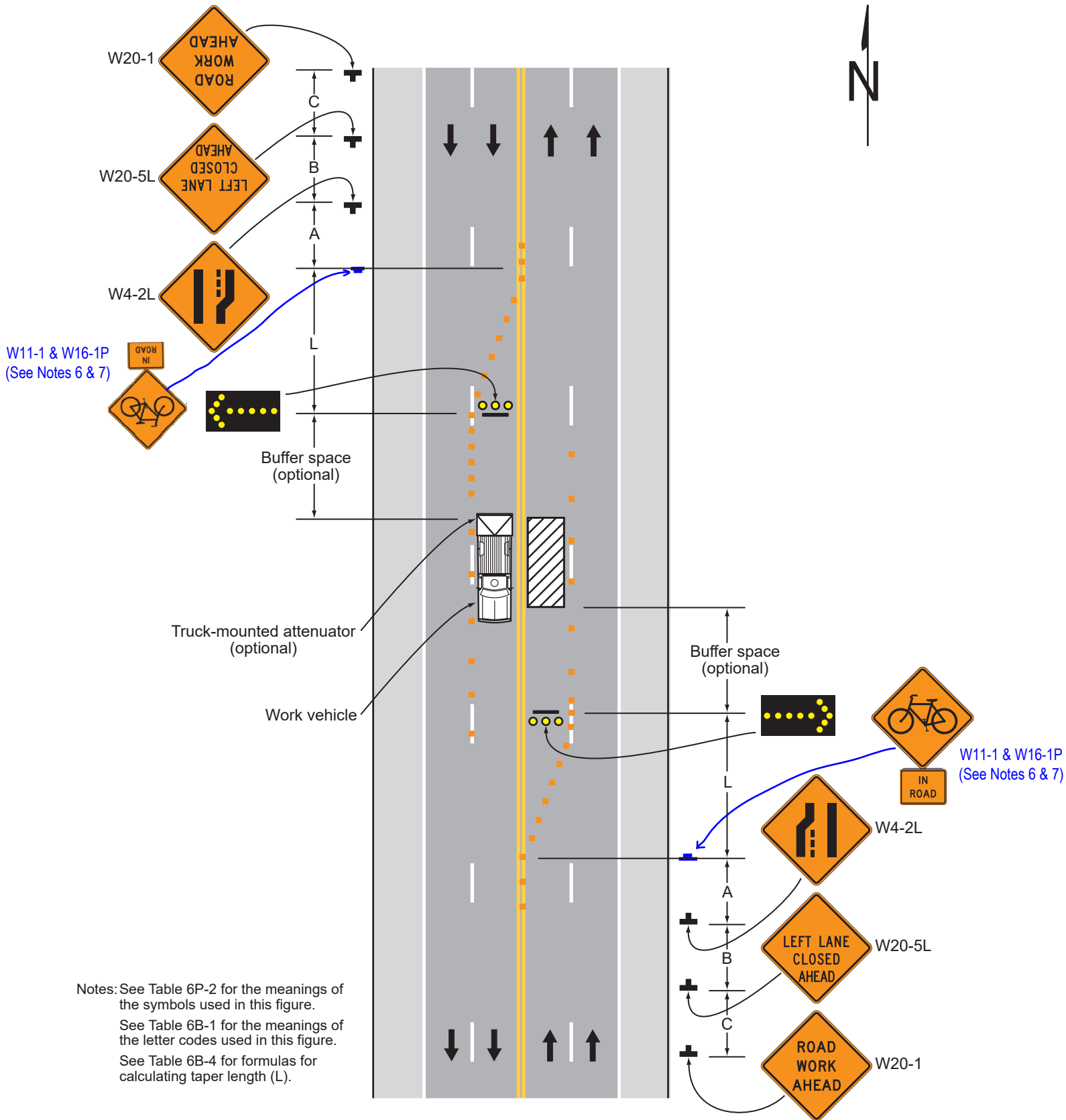
Typical Application 30
