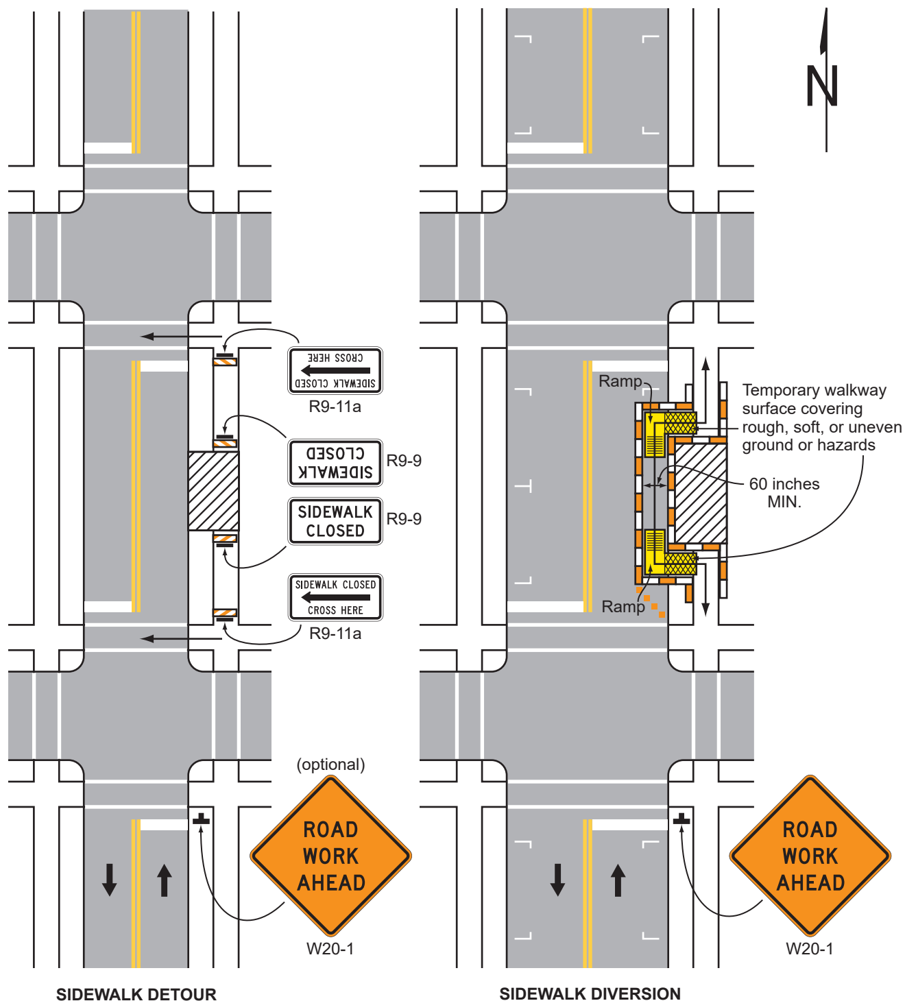
Figure 6P-28. Sidewalk Detour or Diversion (TA-28)
