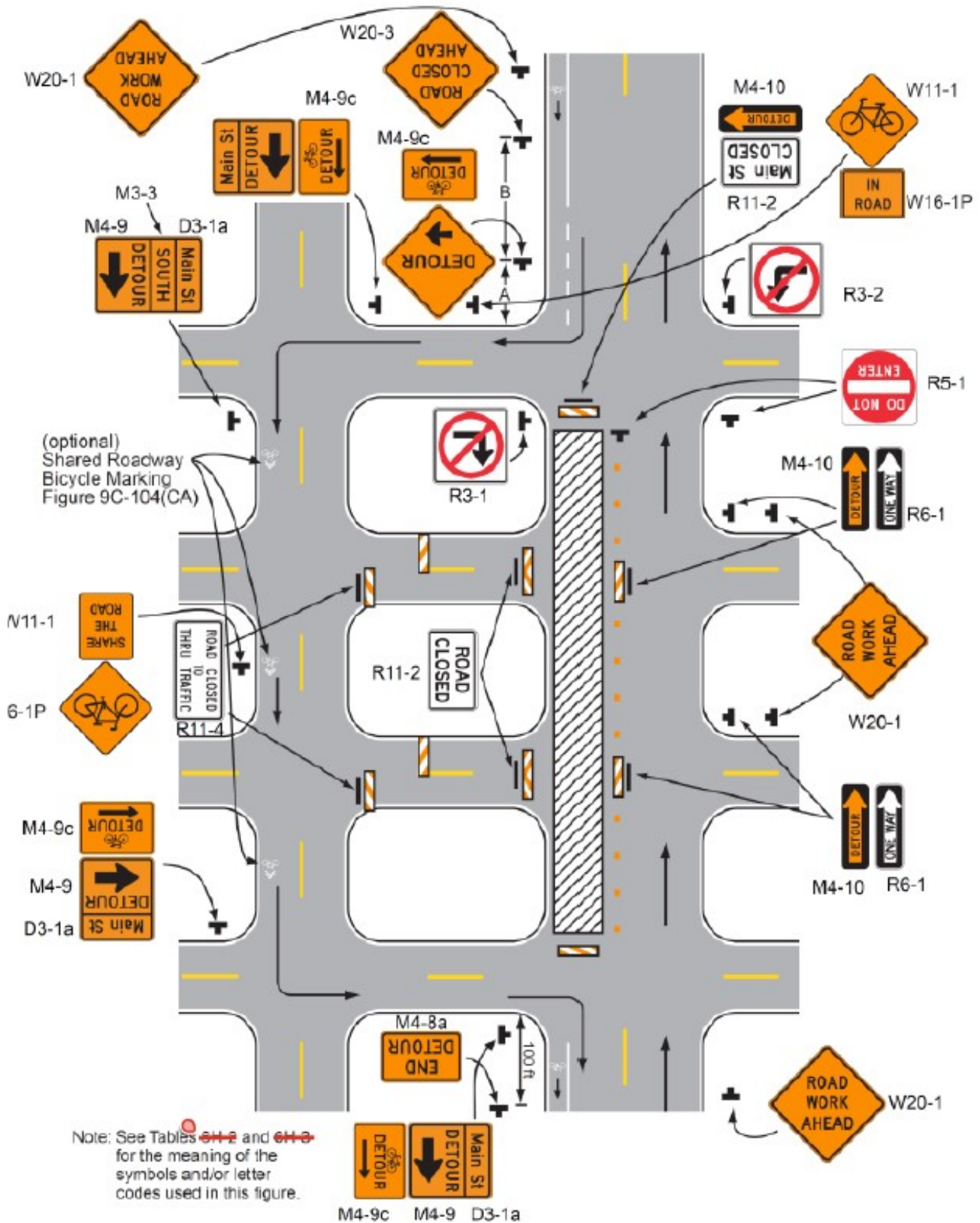
Figure 6P-19(CA) Detour One Travel Direction (TA-19(CA))
