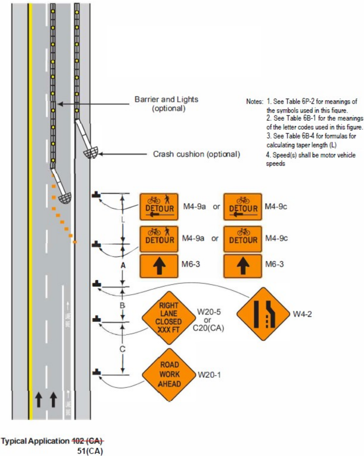
Figure 6P-51(CA). Paved Shoulder Closure with a Bicycle Diversion onto a Temporary Path. (TA-51(CA))
