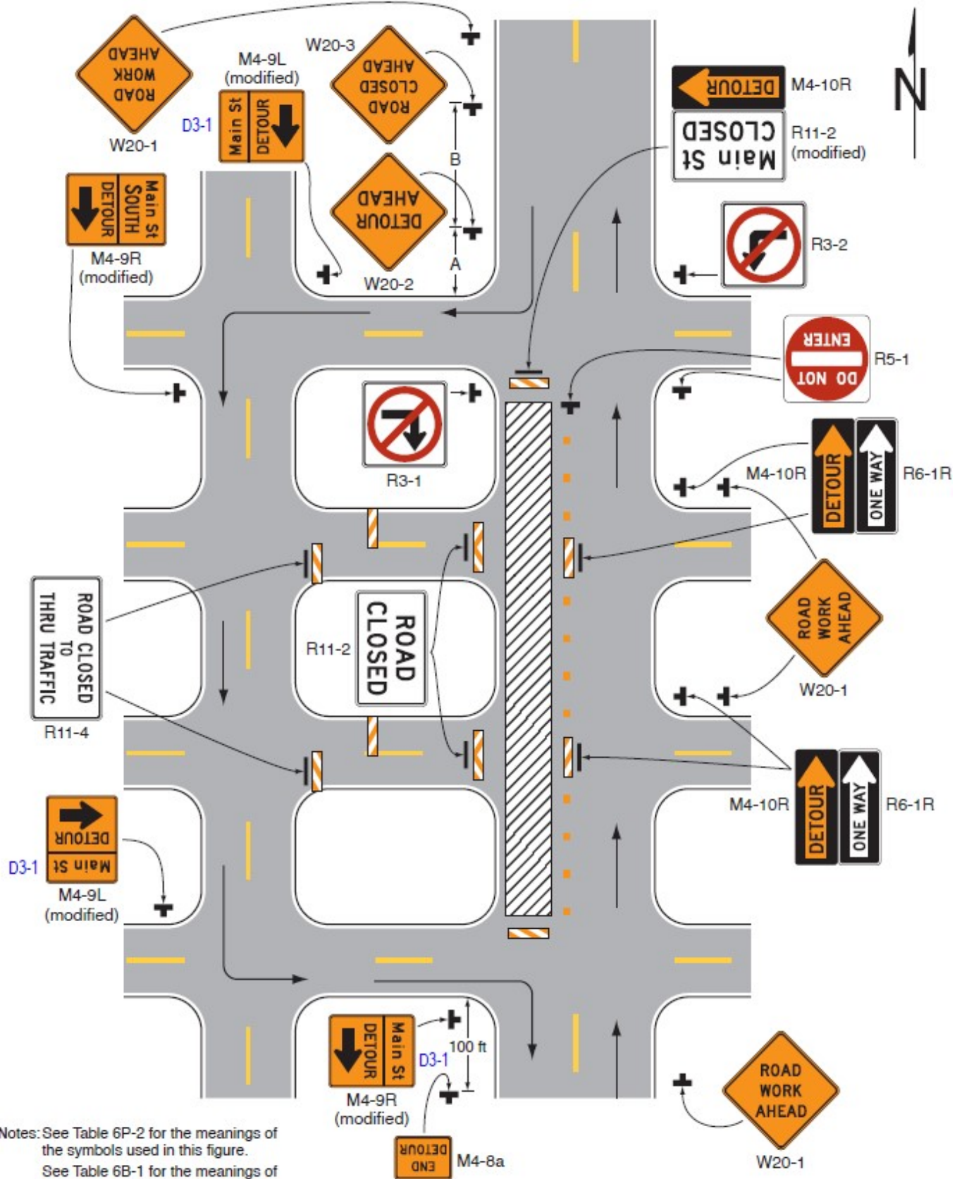
Typical Application 19
