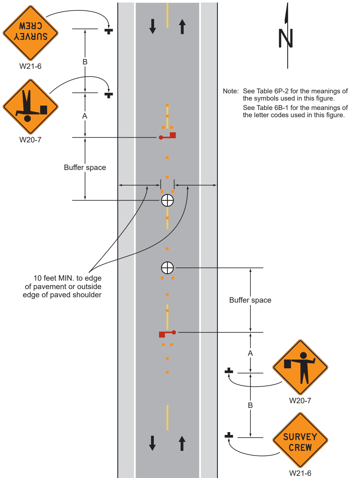
Typical Application 16
