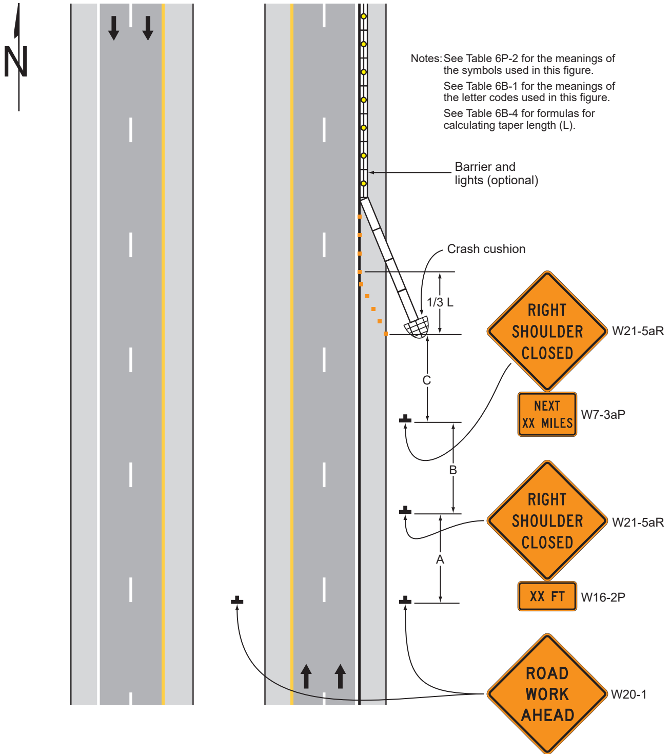
Figure 6P-5. Shoulder Closure on a Freeway (TA-5)
