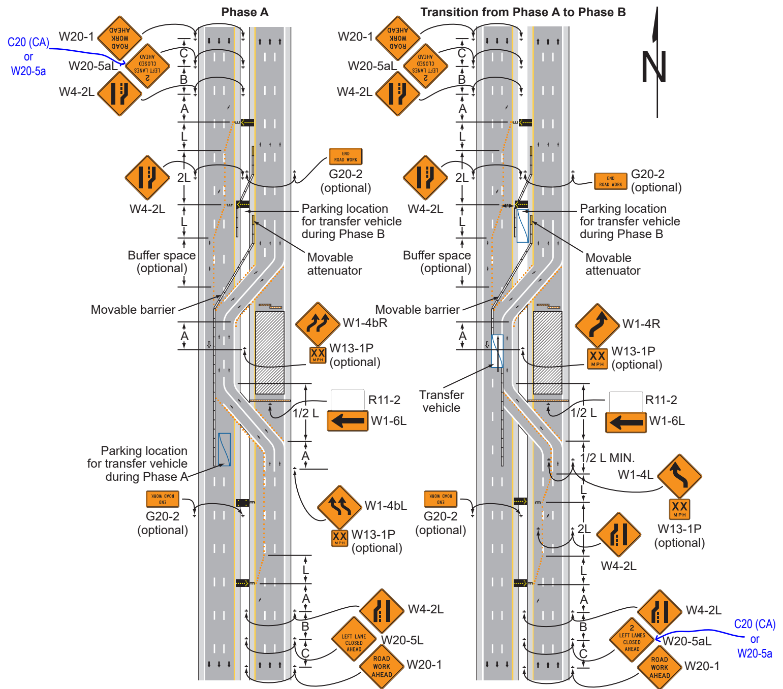
Figure 6P-45. Temporary Reversible Lane Using Movable Barriers (TA-45)
