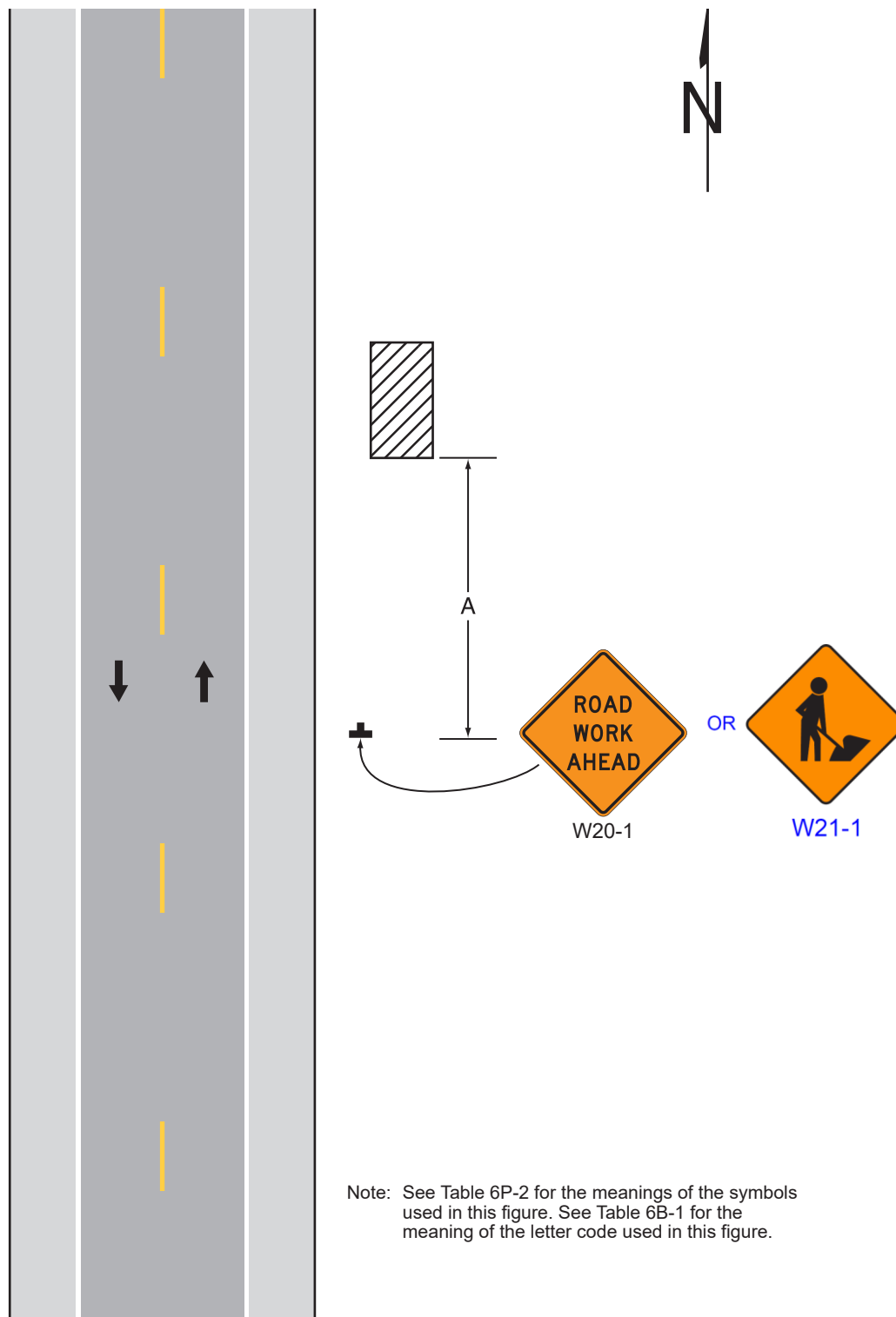
Typical Application 1
