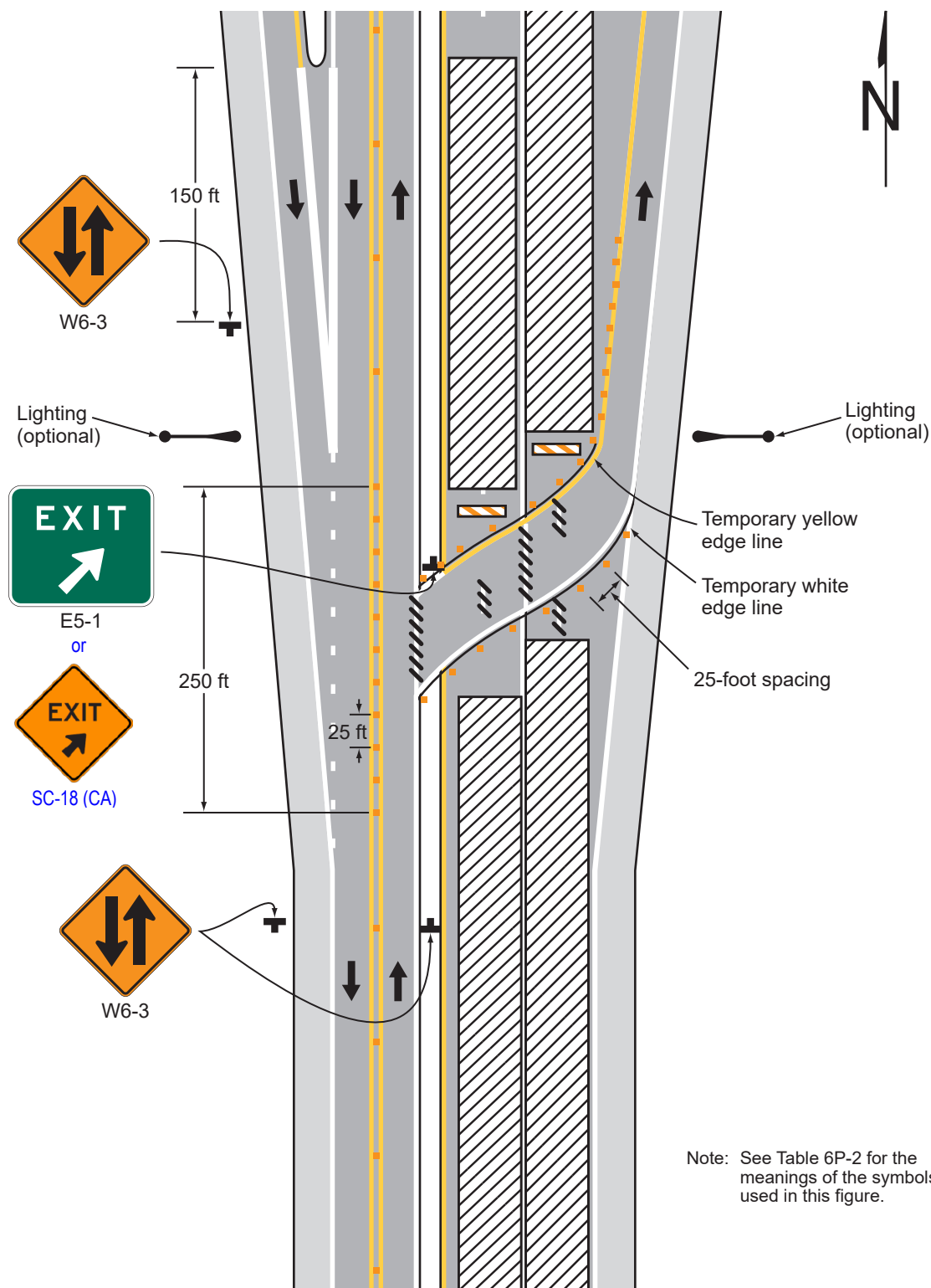
Typical Application 41
