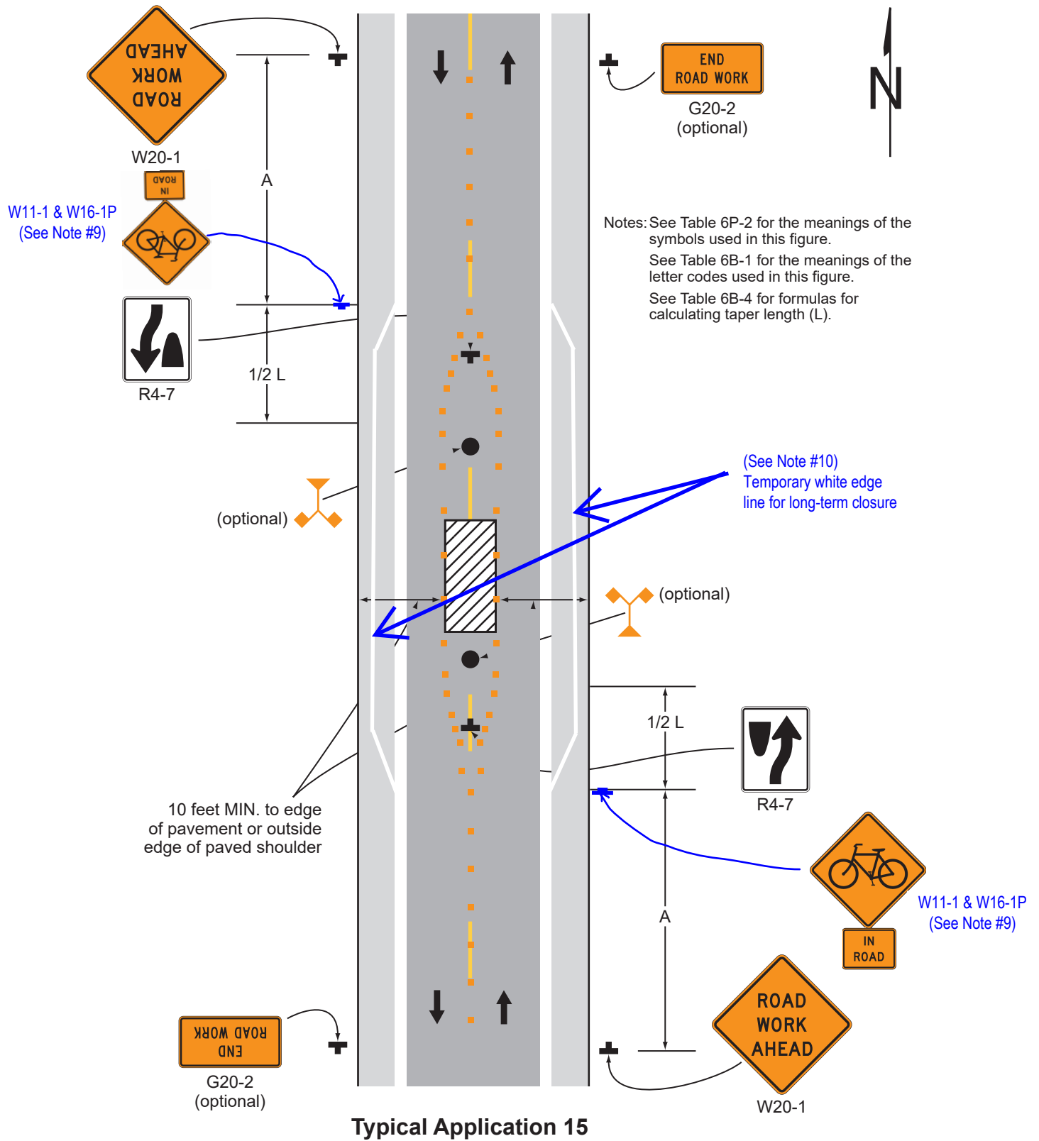
Figure 6P-15. Work in the Center of a Road with Low Traffic Volumes (TA-15)
