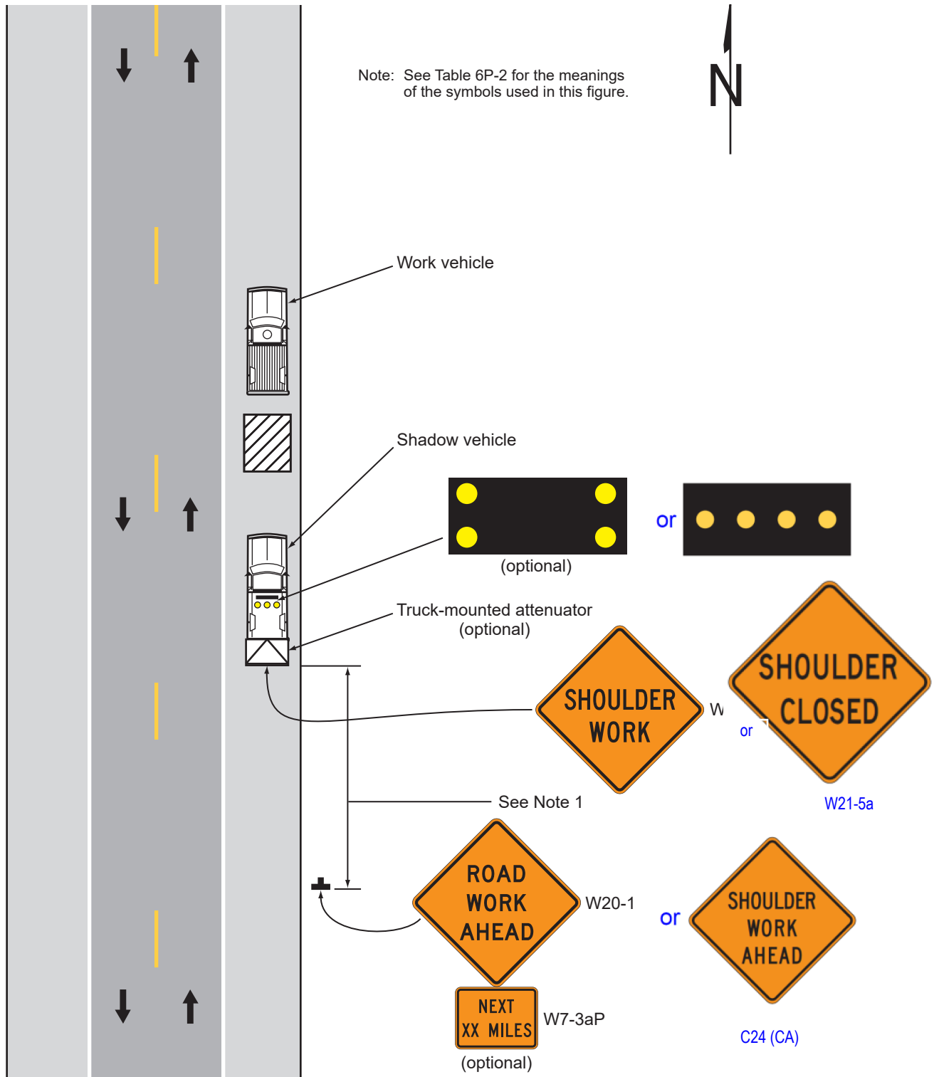
Typical Application 4
