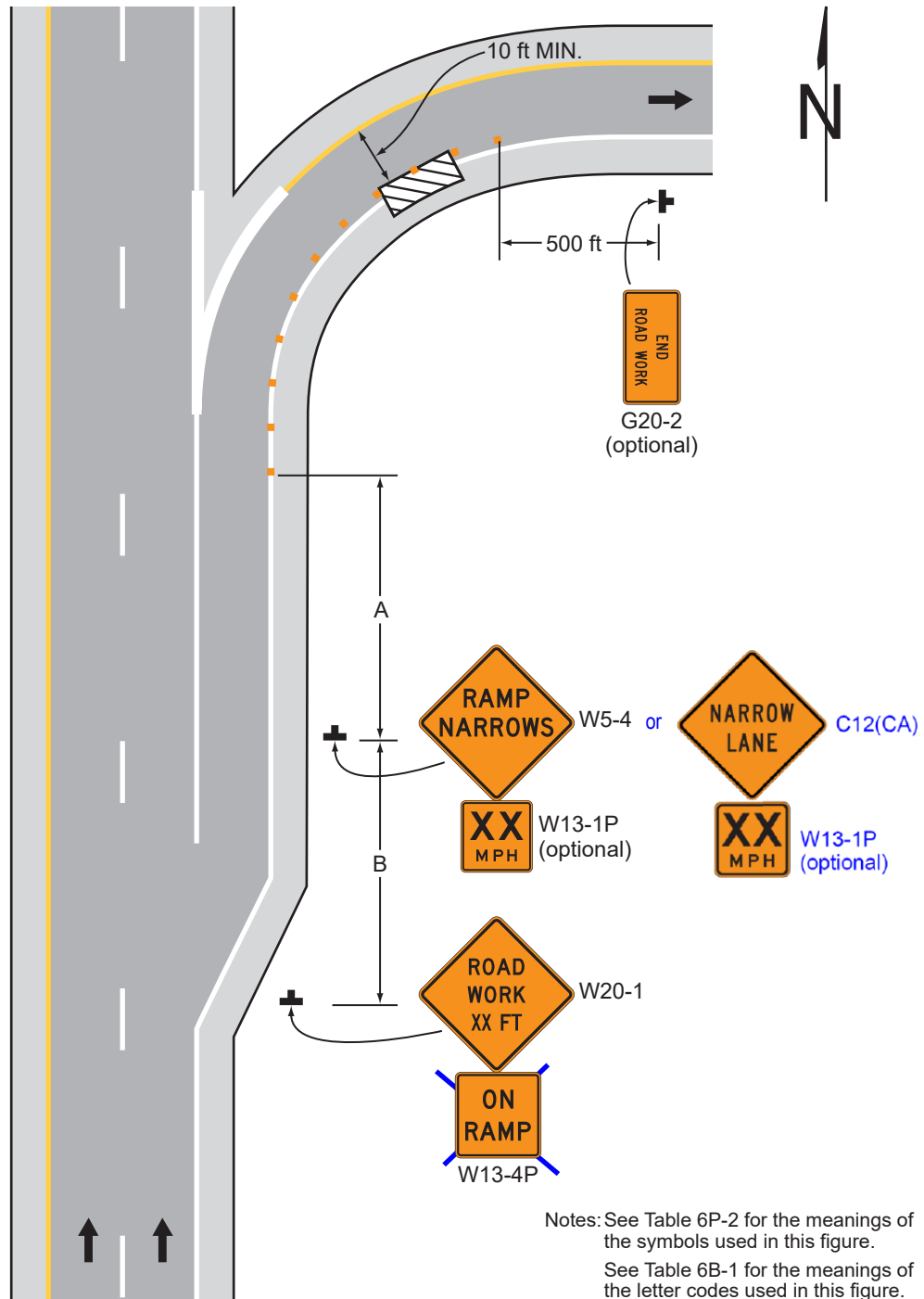
Typical Application 43
