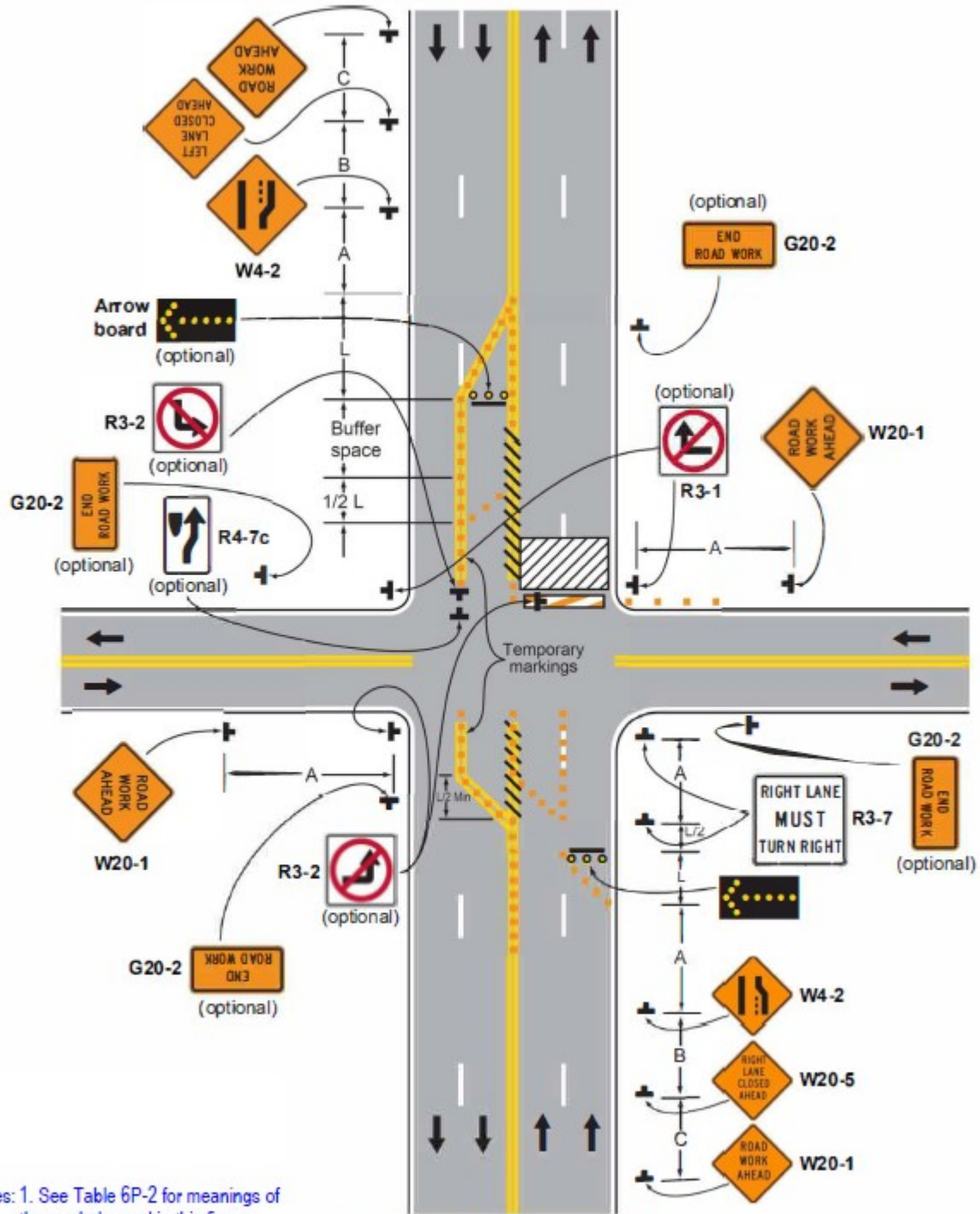
Typical Application 24(CA)
