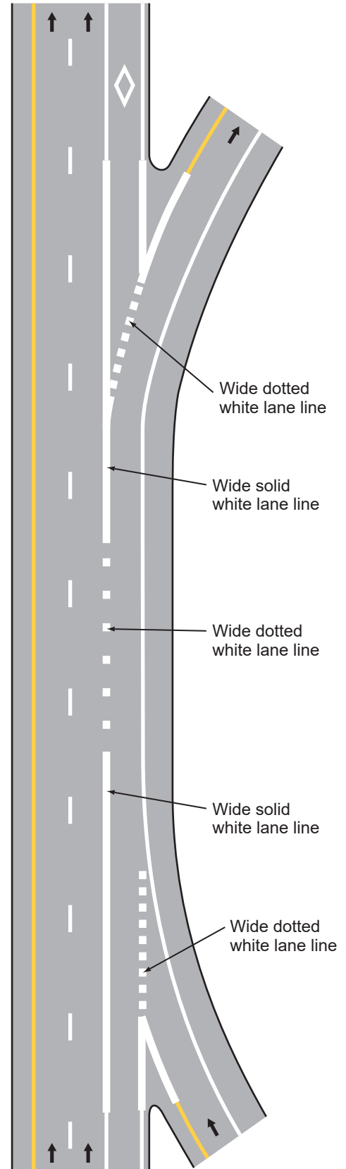
Figure 3E-5. Markings for Part-Time Travel on Shoulder and Application of Pavement Word Markings (Sheet 2 of 3)
