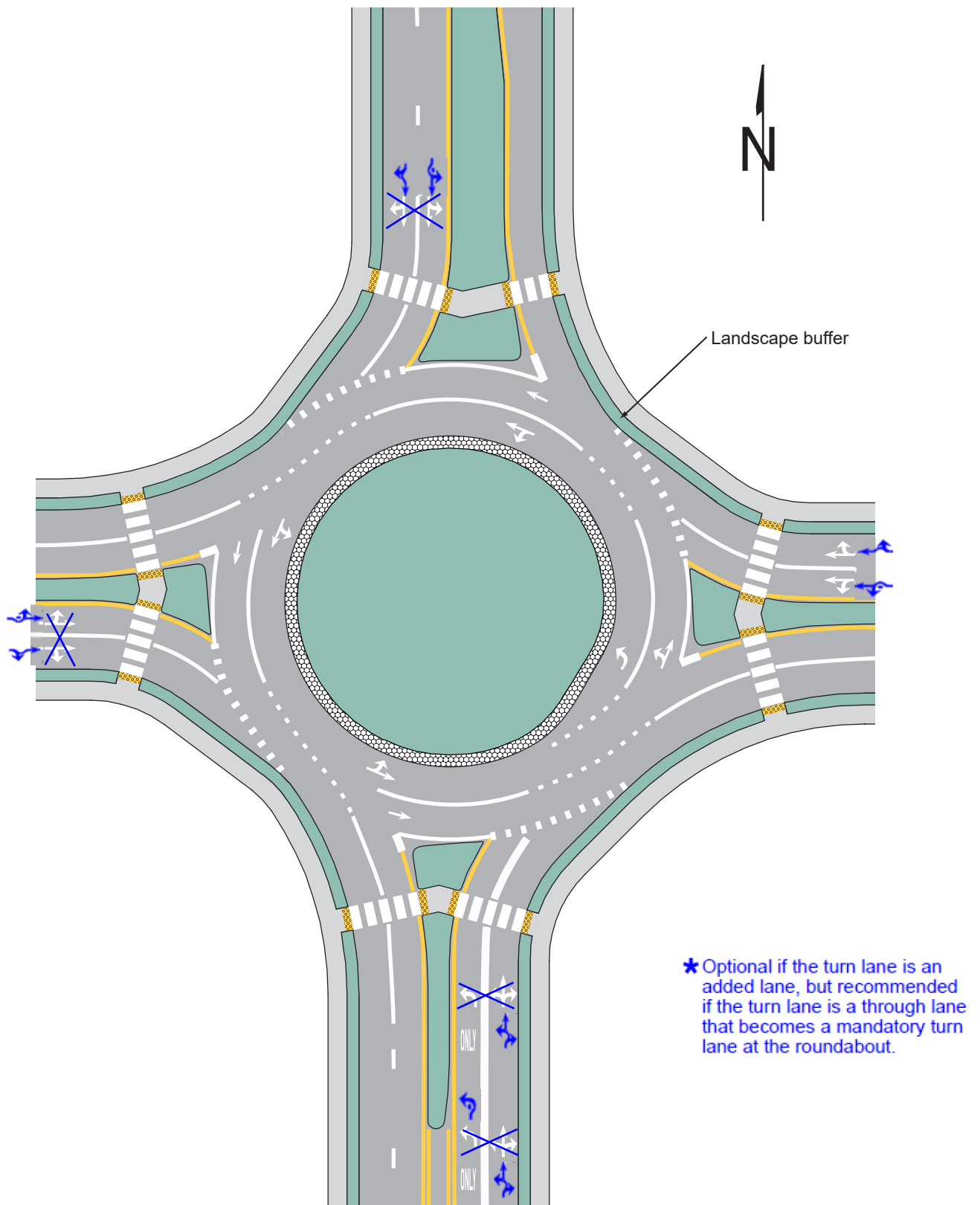
Figure 3D-6. Example of Markings for a Two-Lane Roundabout with a Double Left Turn
