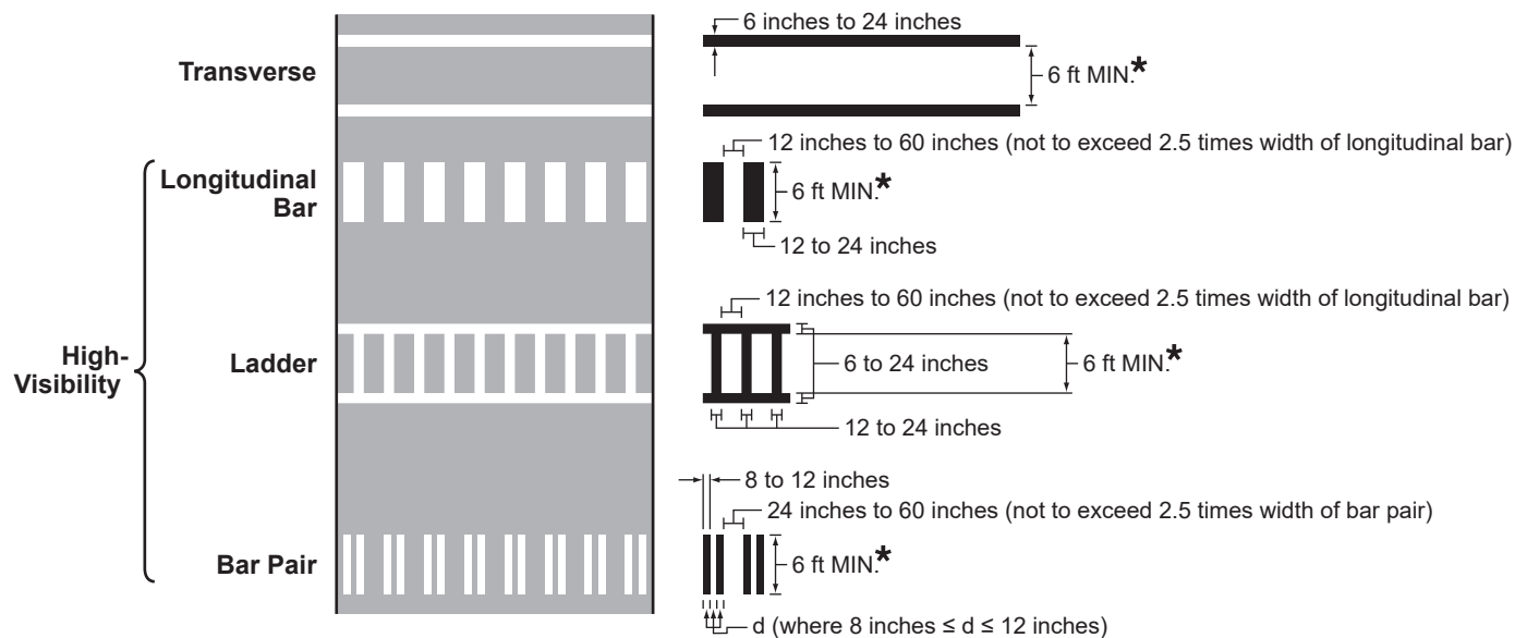
Figure 3C-1. Crosswalk Markings
