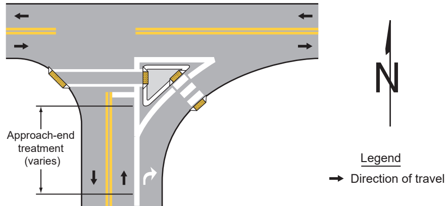
Figure 3J-1. Example of Markings for an Approach-End Treatment to an Island
