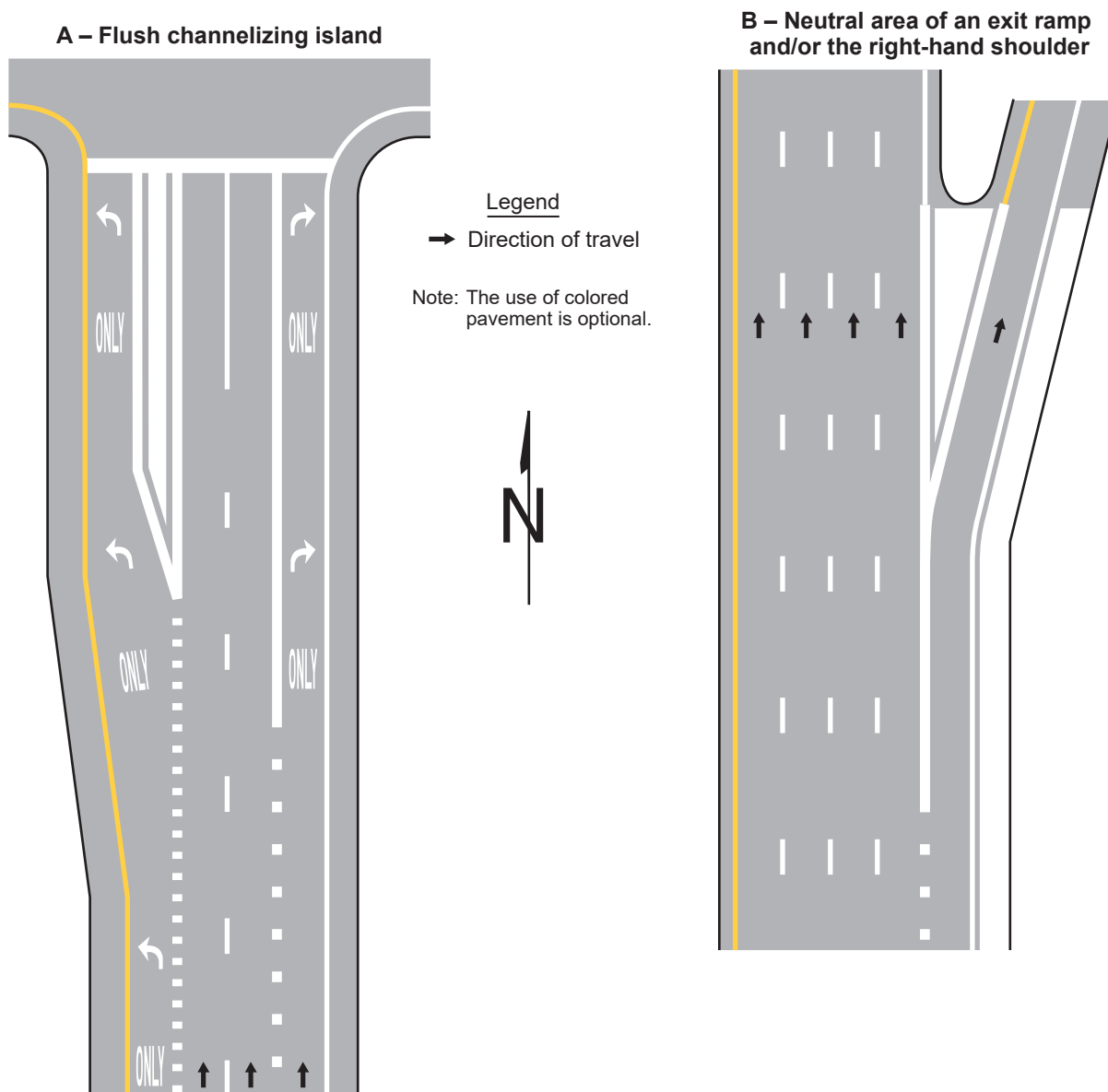
Figure 3H-3. Examples of White-Colored Pavement Applications
