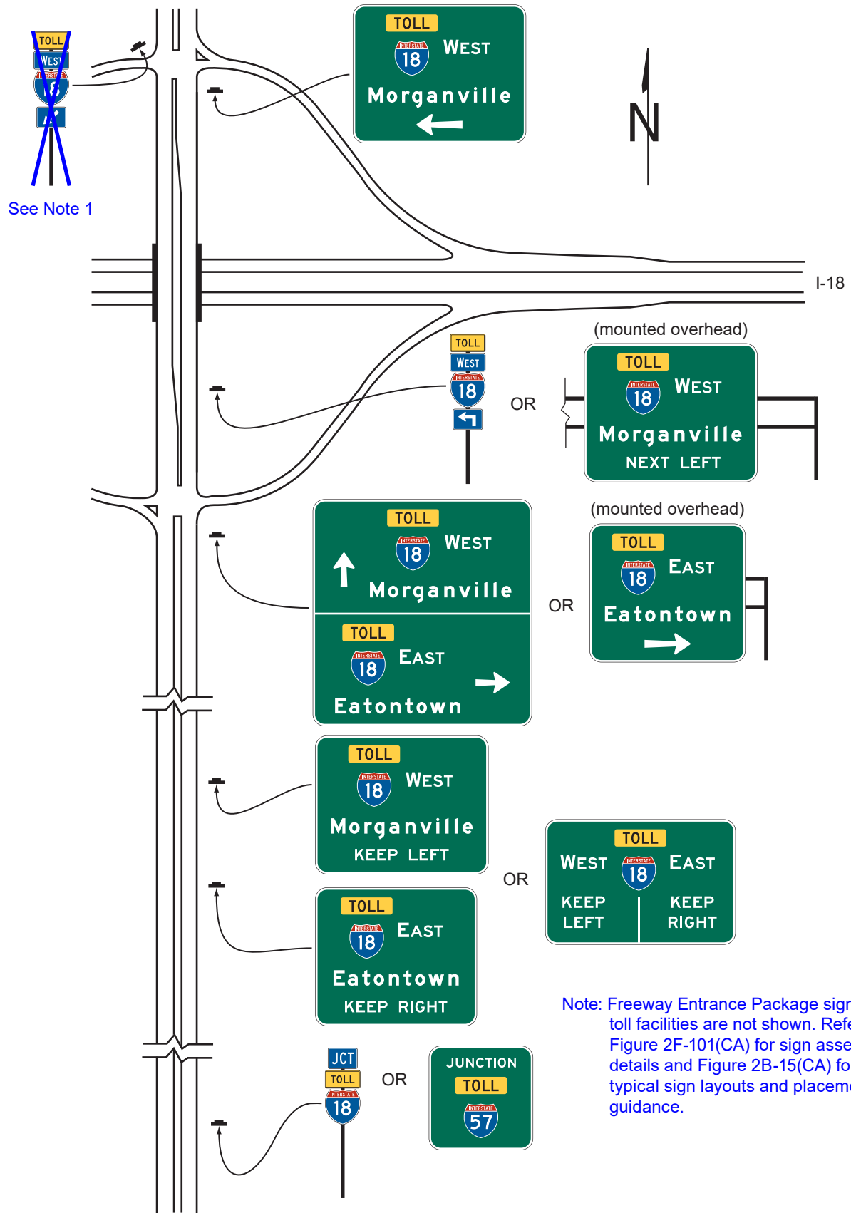
Figure 2F-7. Examples of Multi-Lane Crossroad Signing for a Diamond Interchange
