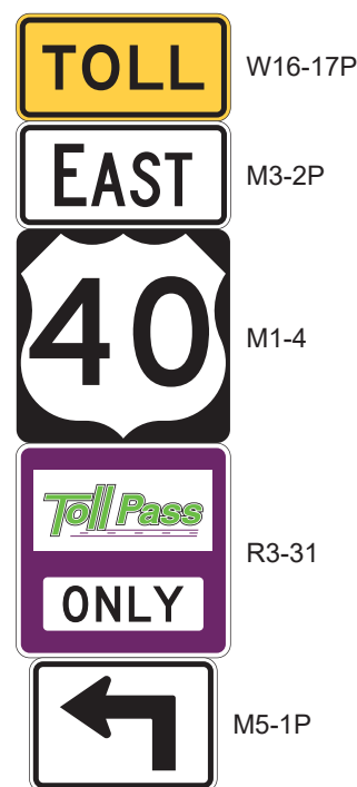
Figure 2F-3. ETC Account-Only Auxiliary Signs for Use in Route Sign Assemblies
