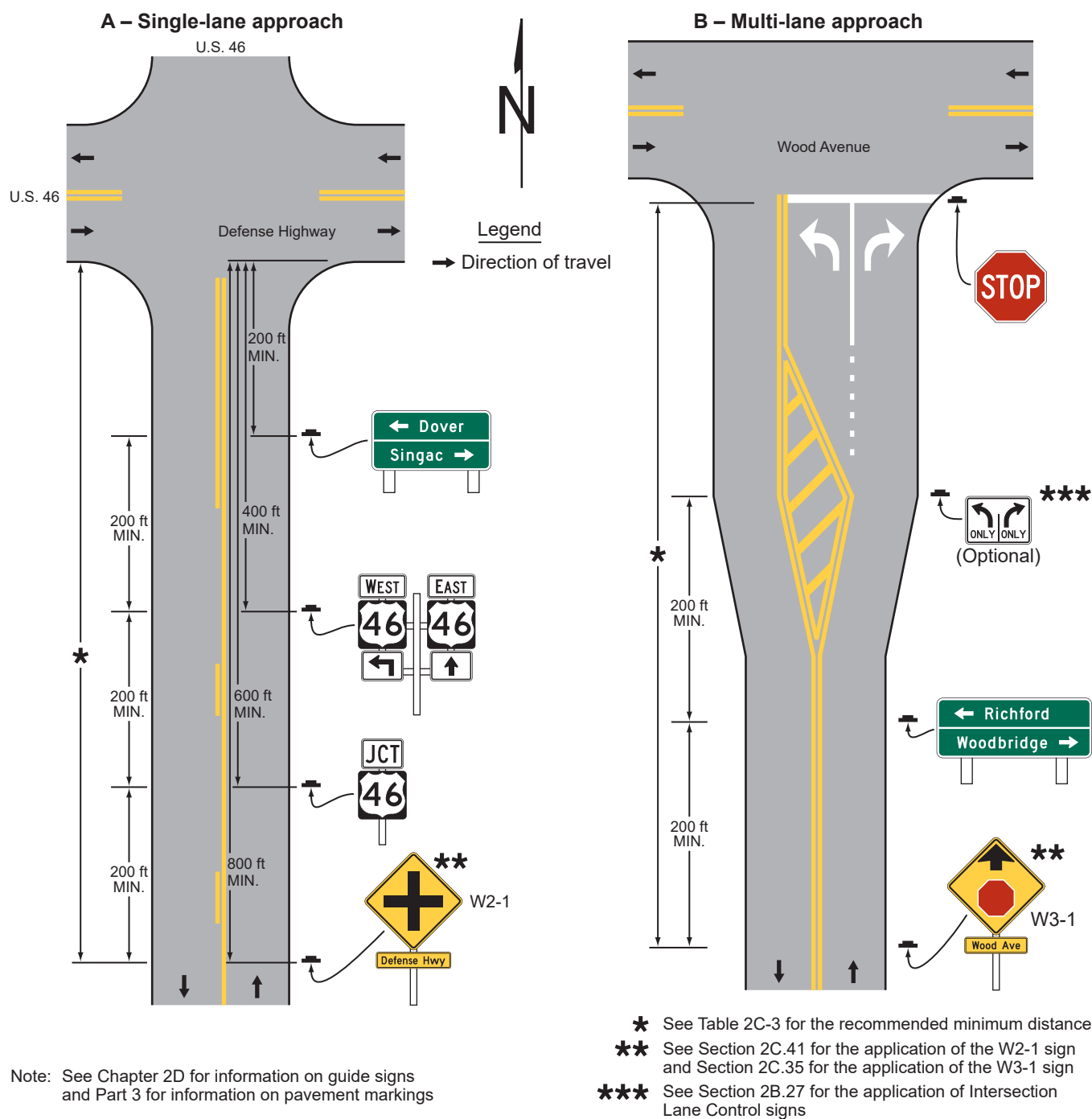
Figure 2A-4. Relative Locations of Regulatory, Warning, and Guide Signs on an Intersection Approach (Sheet 1 of 4)
