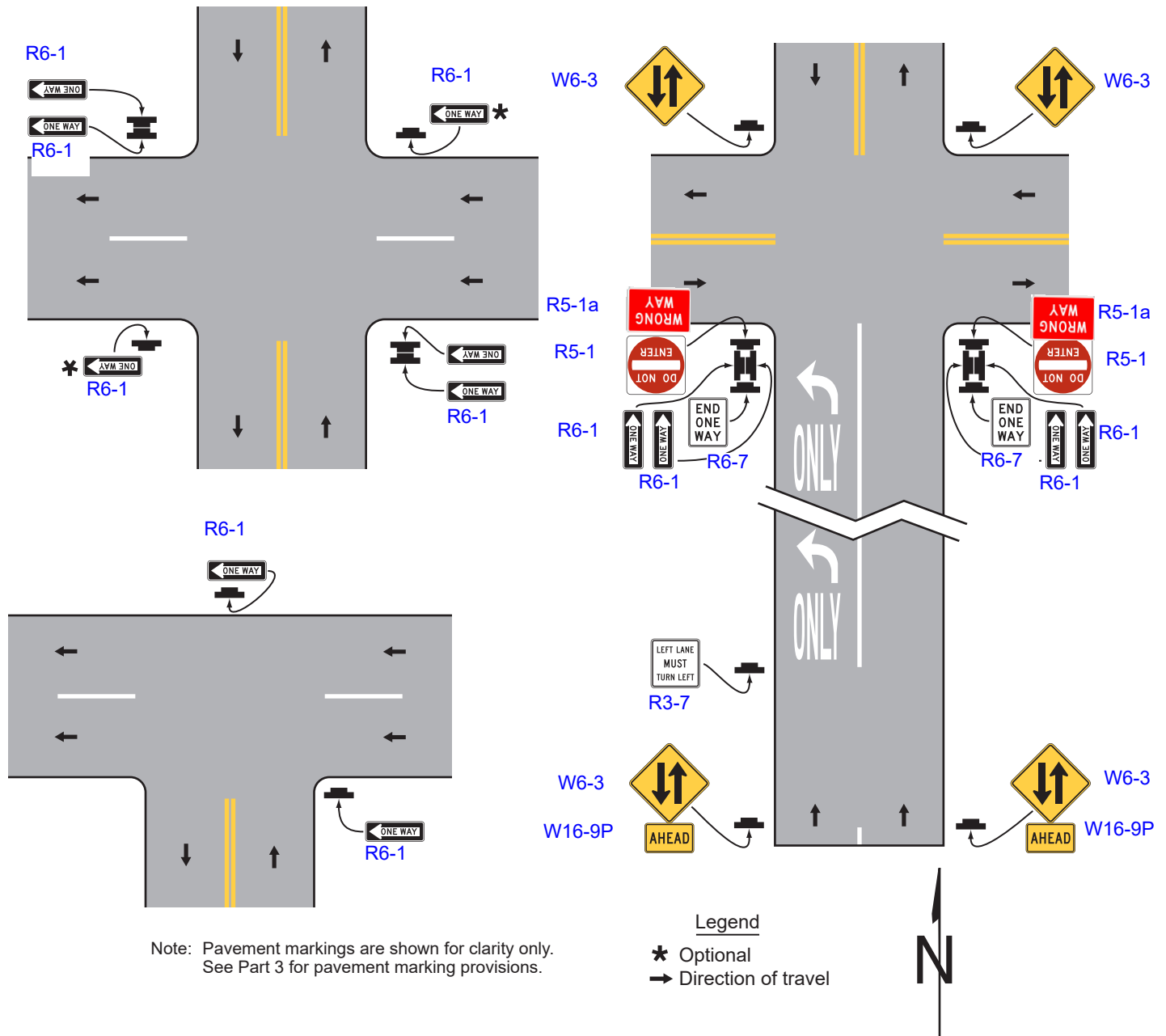
Figure 2B-18. Locations of ONE WAY Signs
