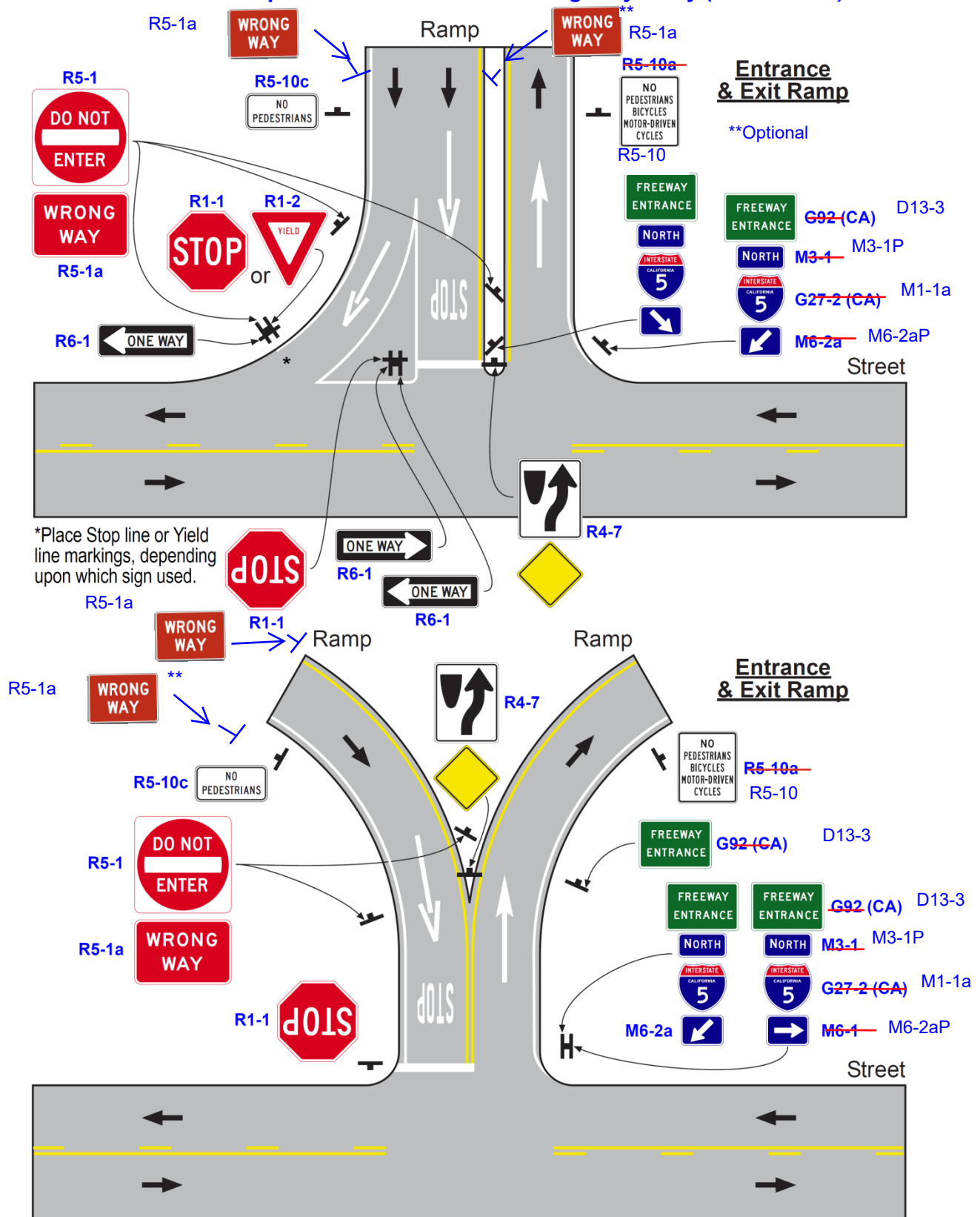
Figure 2B-18 (CA) . Example of Application of Regulatory Signing and Pavement Markings at an Exit Ramp Termination to Deter Wrong-Way Entry (Sheet 3 of 5)
