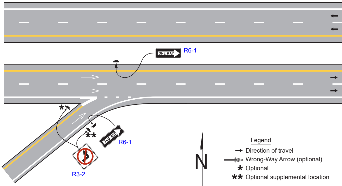
Figure 2B-16. Example of Application of Regulatory Signing and Pavement Markings at an Entrance Ramp Terminal
