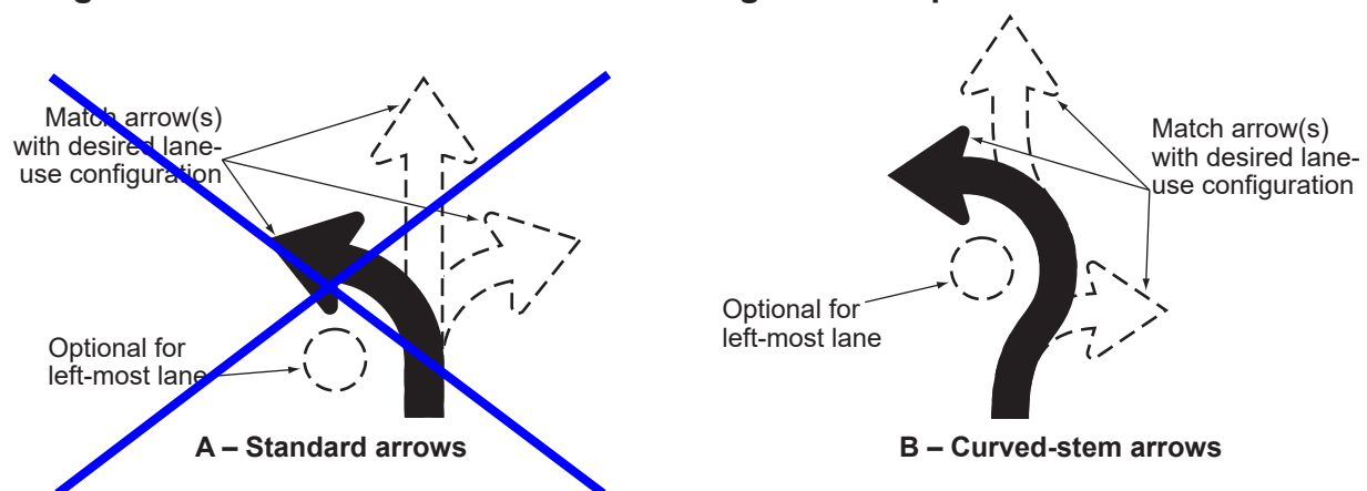
Figure 2B-5. Intersection Lane Control Sign Arrow Options for Roundabouts
