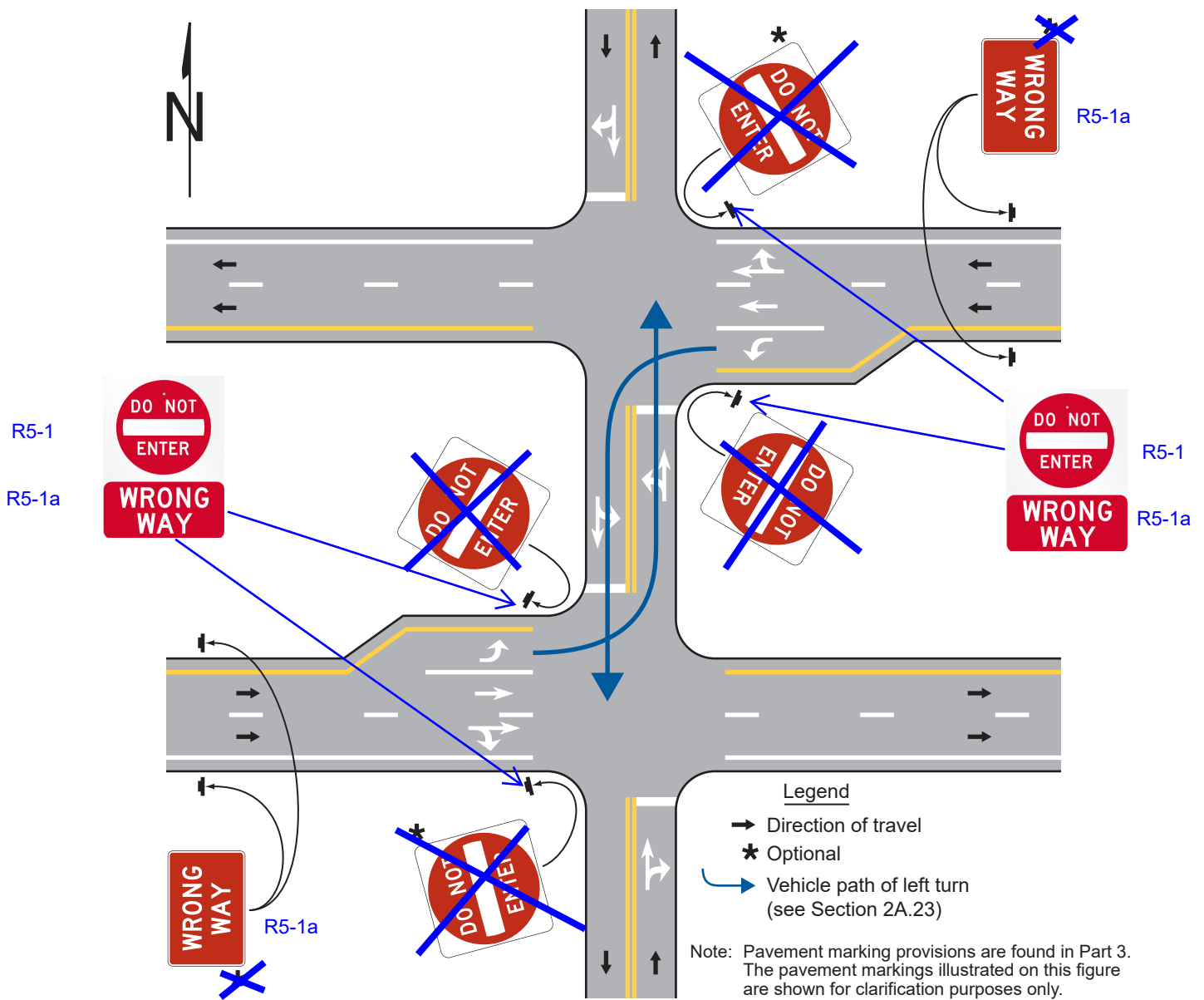
Figure 2B-14. Locations of DO NOT ENTER and WRONG WAY Signing for Divided Highway Crossings that Function as Two Separate Intersections
