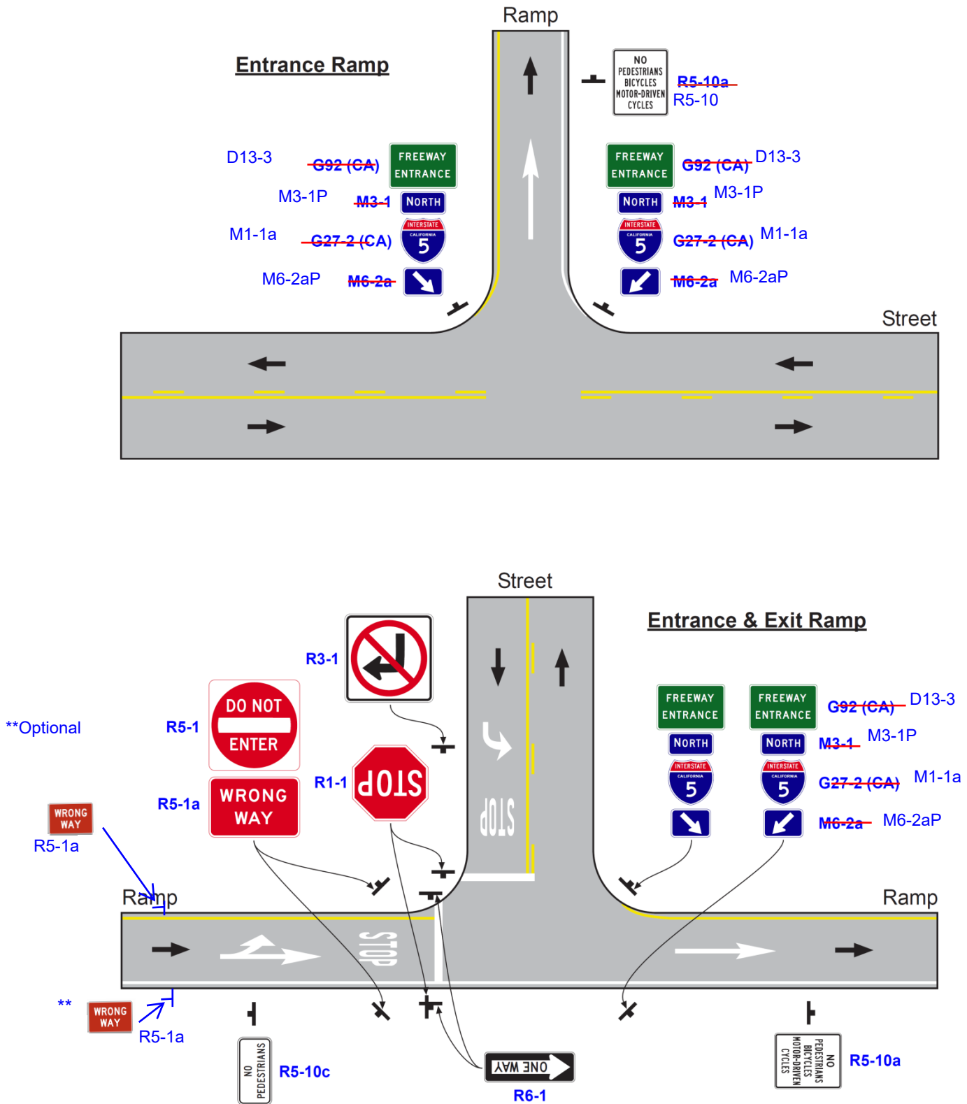
Figure 2B-18 (CA). Example of Application of Regulatory Signing and Pavement Markings at an Exit Ramp Termination to Deter Wrong-Way Entry (Sheet 2 of 5)
