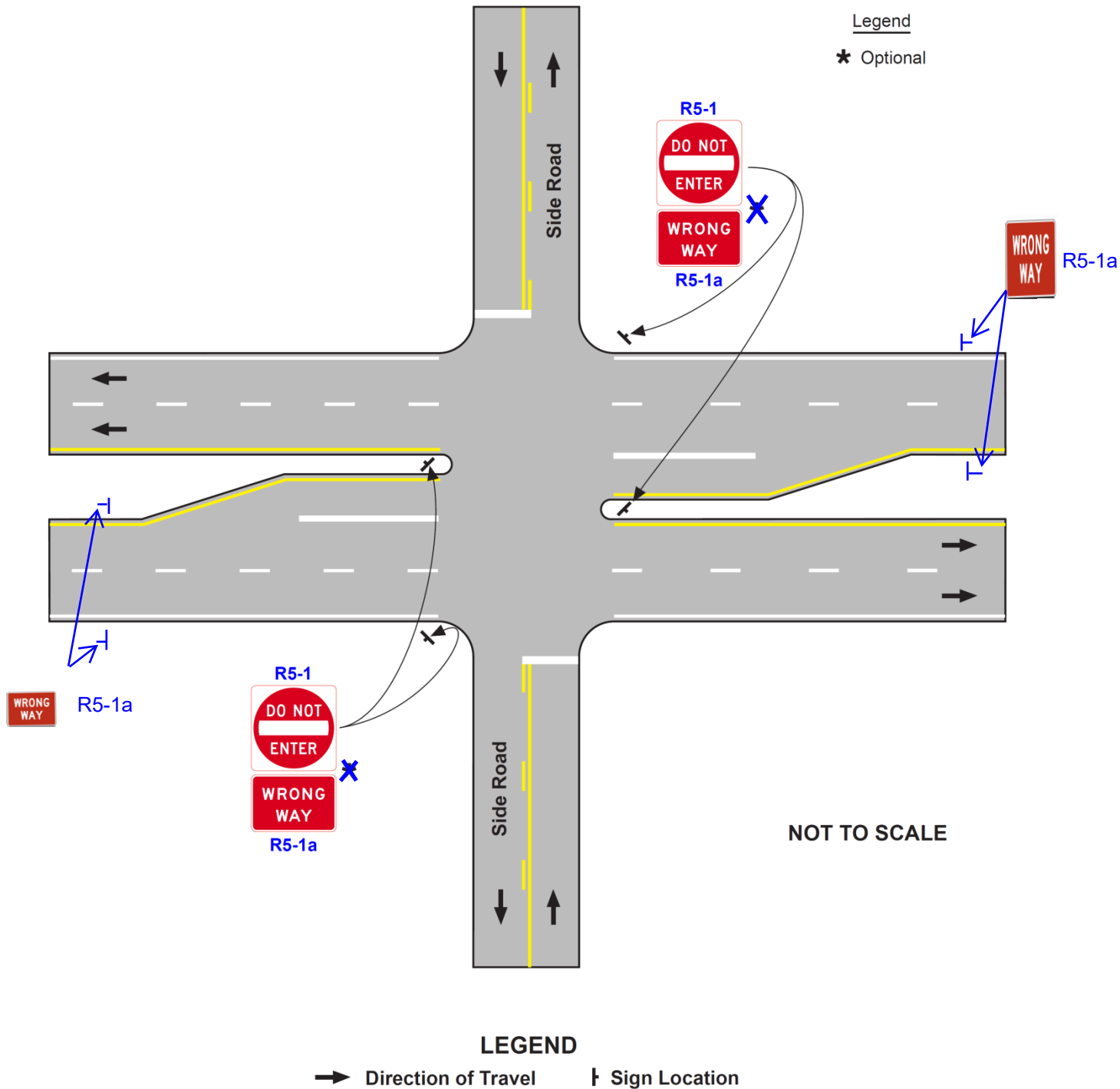
Figure 2B-14(CA). Locations of DO NOT ENTER and WRONG WAY Signing for Divided Highway Crossings that Function as a Single Intersection
