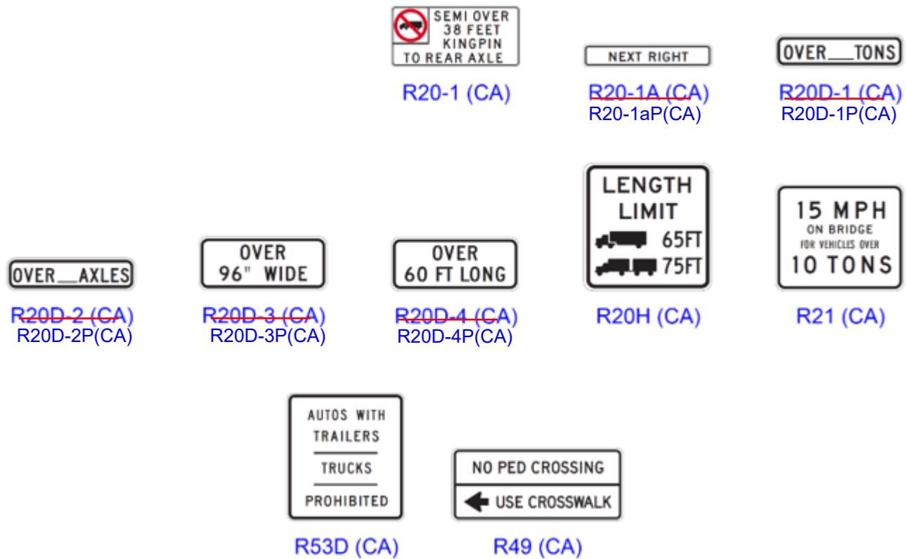
Figure 2B-11 (CA). Selective Exclusion Signs Figure 2B-12(CA). Selective Exclusion Signs and Plaques
