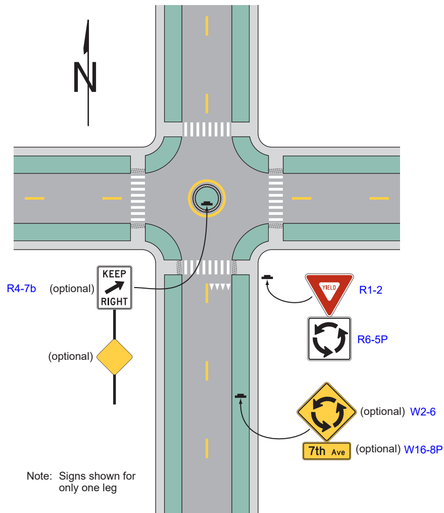
Figure 2B-24. Example of Regulatory and Warning Signs for a Neighborhood Traffic Circle
