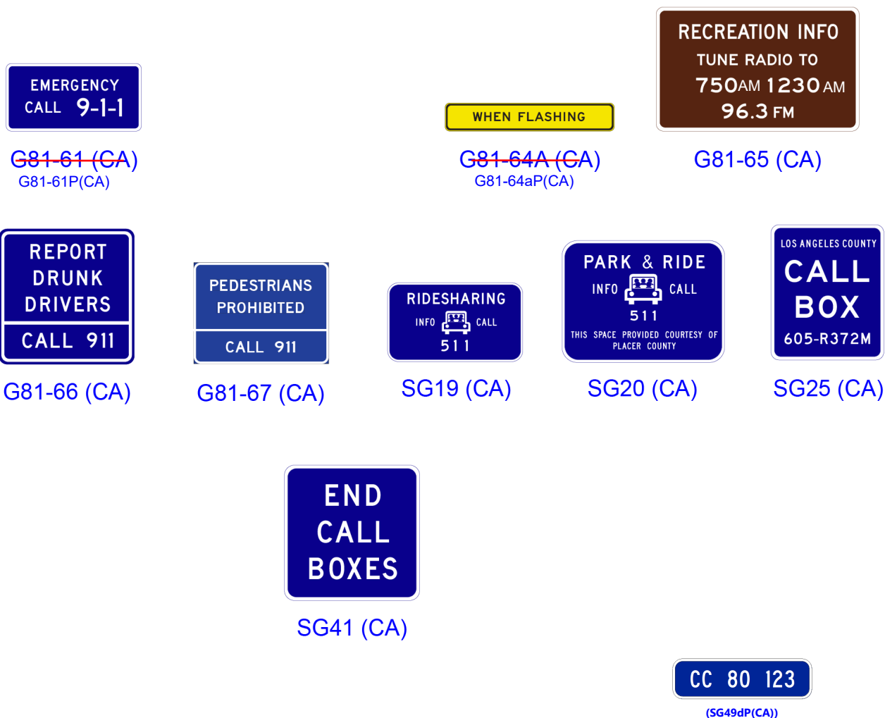
Figure 2I-8(CA). California Radio, Telephone, and Carpool Information Signs
