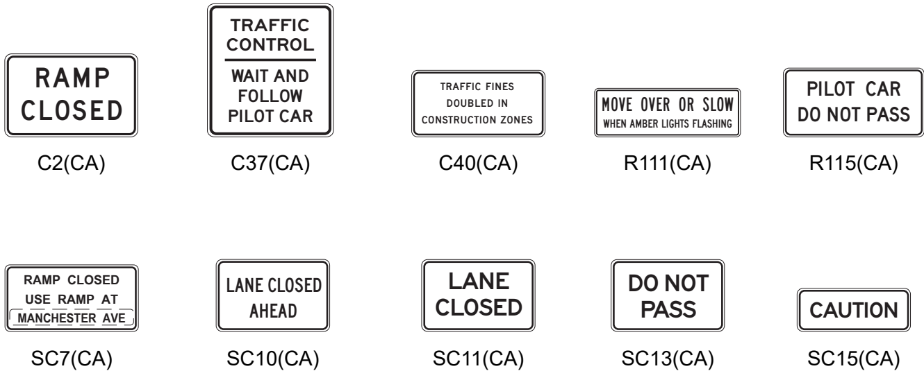
Figure 6G-101(CA). California Regulatory Signs and Plaques in Temporary Traffic Control Zones
