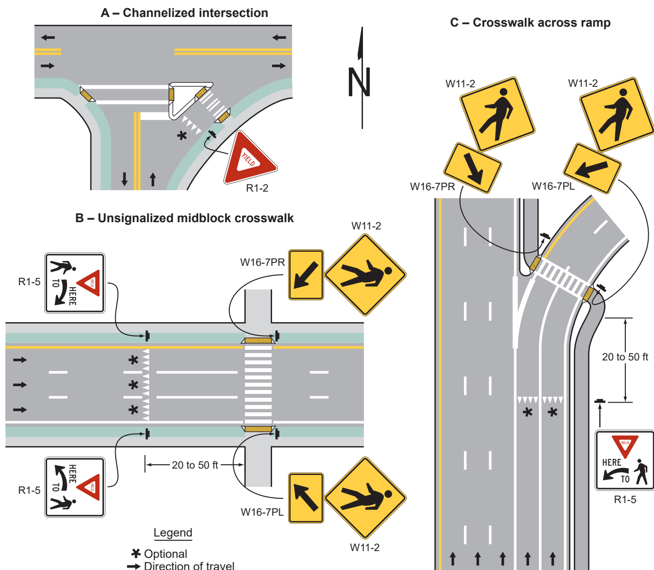
Figure 3B-16. Examples of Yield Line Applications
