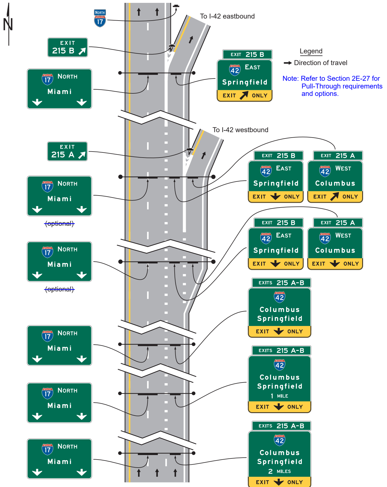
B – Example of signing for successive exit ramps with a dropped lane at the second exit
