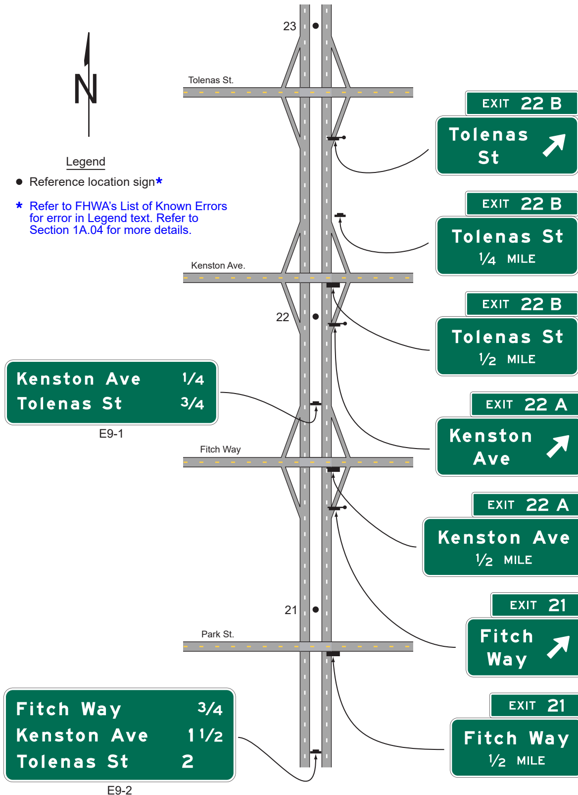
Figure 2E-11. Example of Using a Series of Interchange Sequence Signs for Closely-Spaced Interchanges
