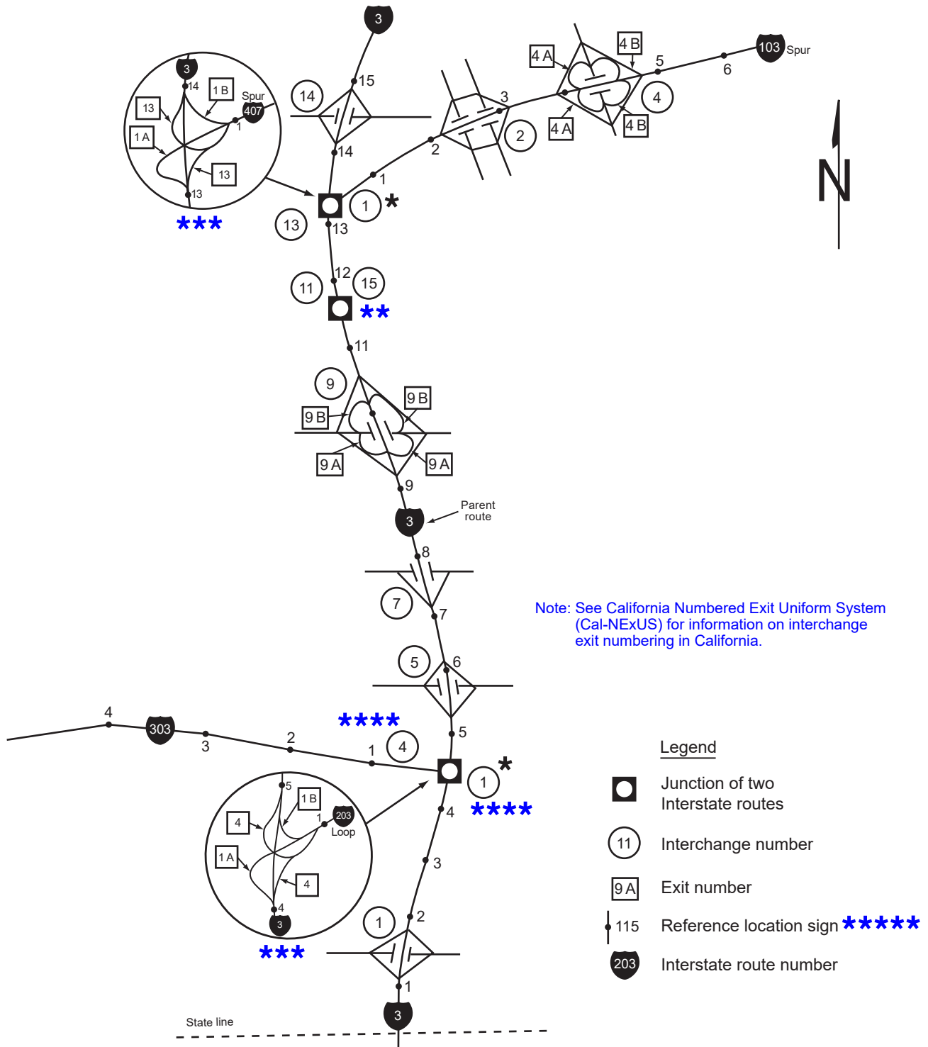
Figure 2E-7. Example of Interchange Numbering for Mainline and Spur Routes
