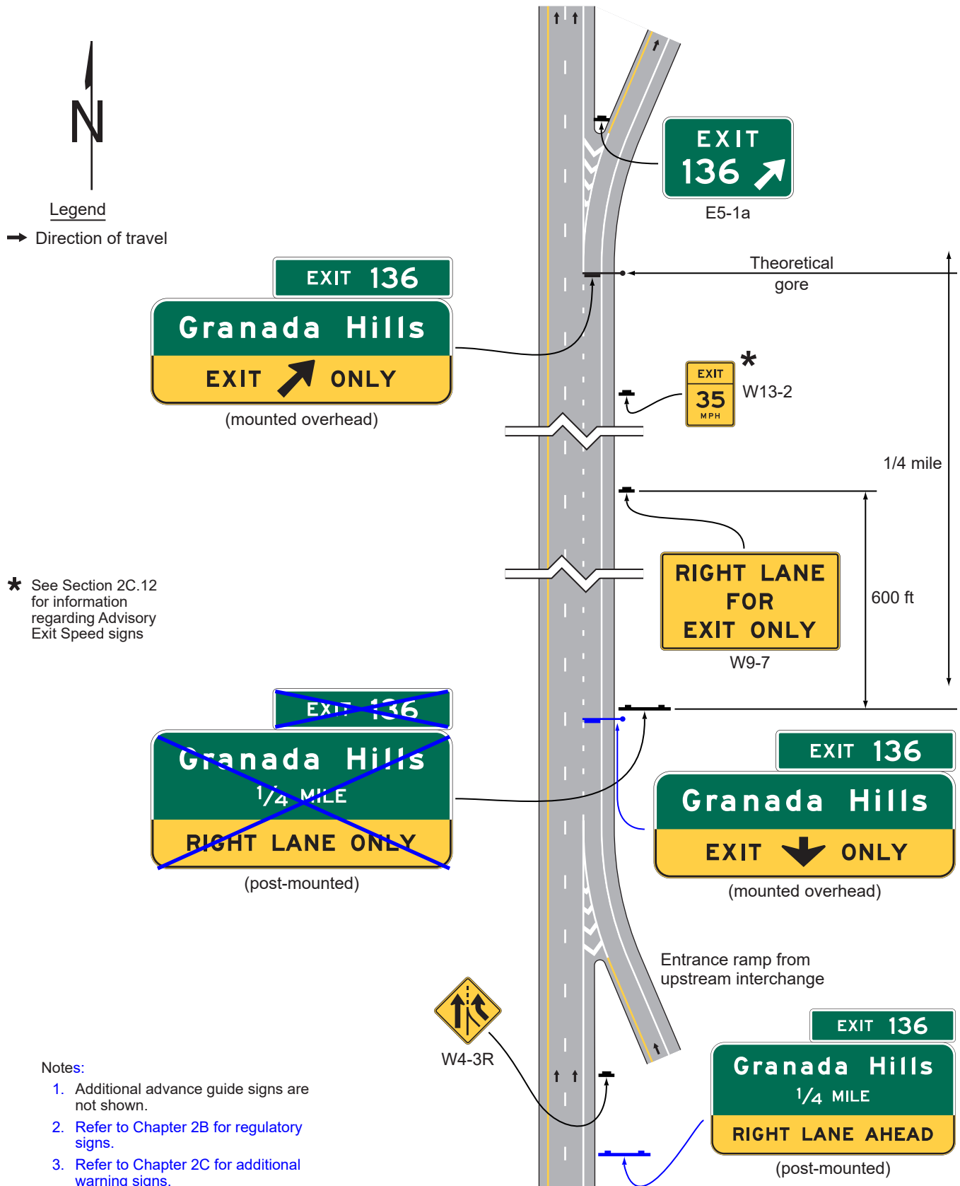
Figure 2E-21. Example of Post-Mounted Advance Guide and Supplemental Warning Signs for a Dropped Auxiliary Lane between Separate Interchange Ramps
