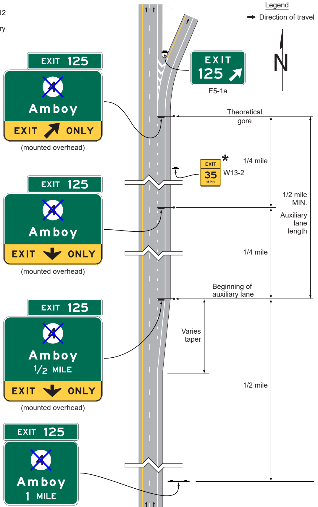
Figure 2E-22. Example of Guide Signs for an Auxiliary Lane of at Least One-Half Mile in Length
