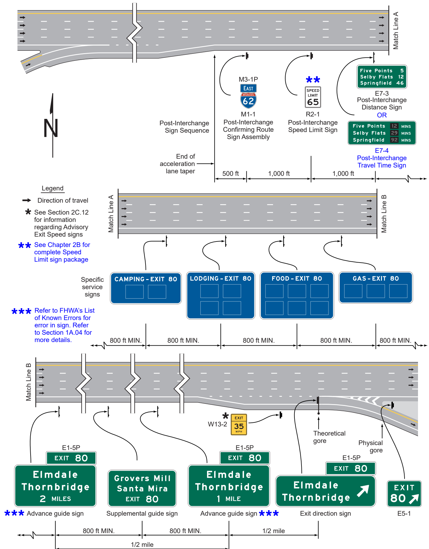
Figure 2E-2. Typical Sequence of Interchange Guide Signs
