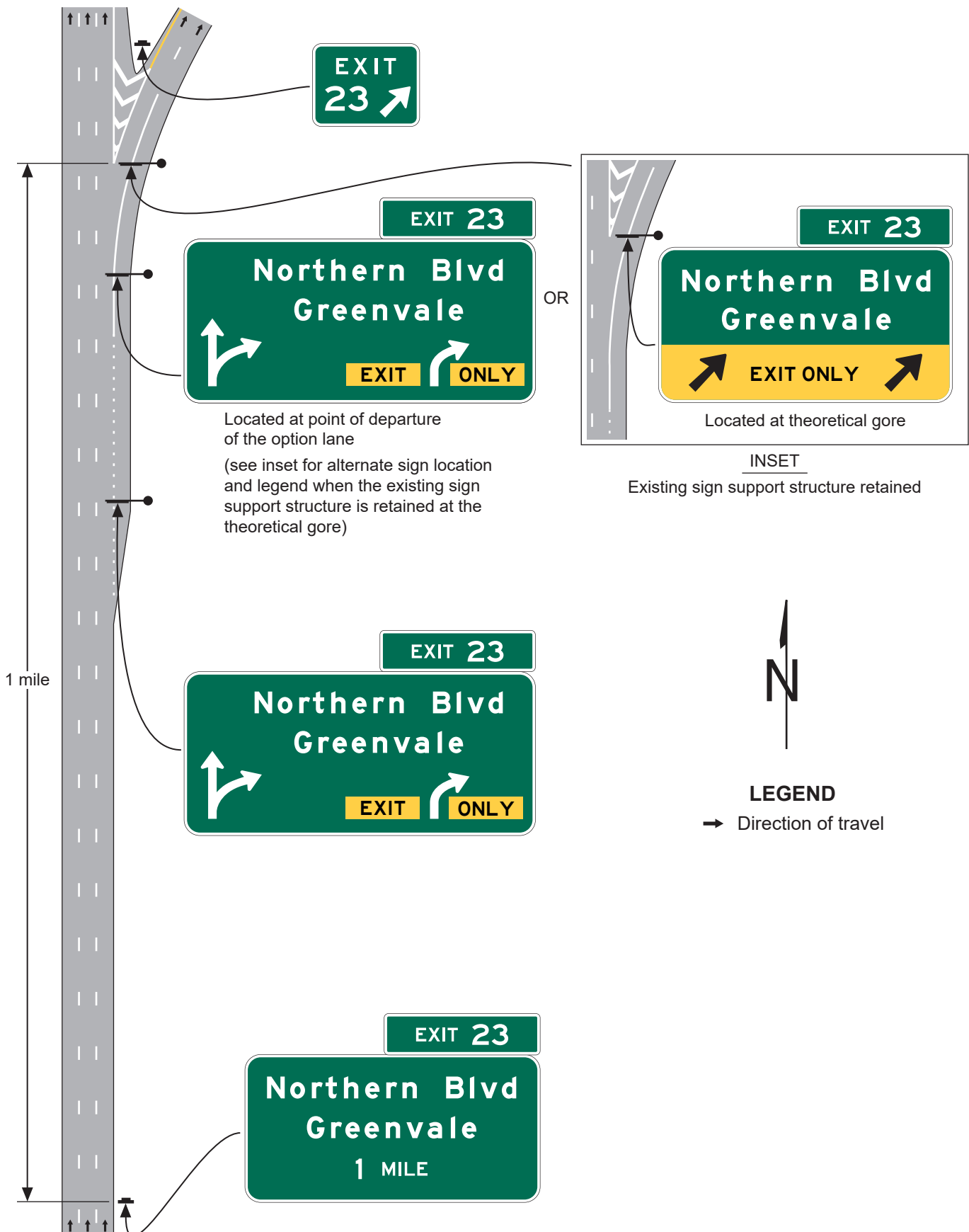
Figure 2E-45(CA). California Example of Signing for a Two-Lane Intermediate or Minor Interchange Exit with Option and Auxiliary Lanes using Partial-Width Overhead Arrow-per-Lane Signs
