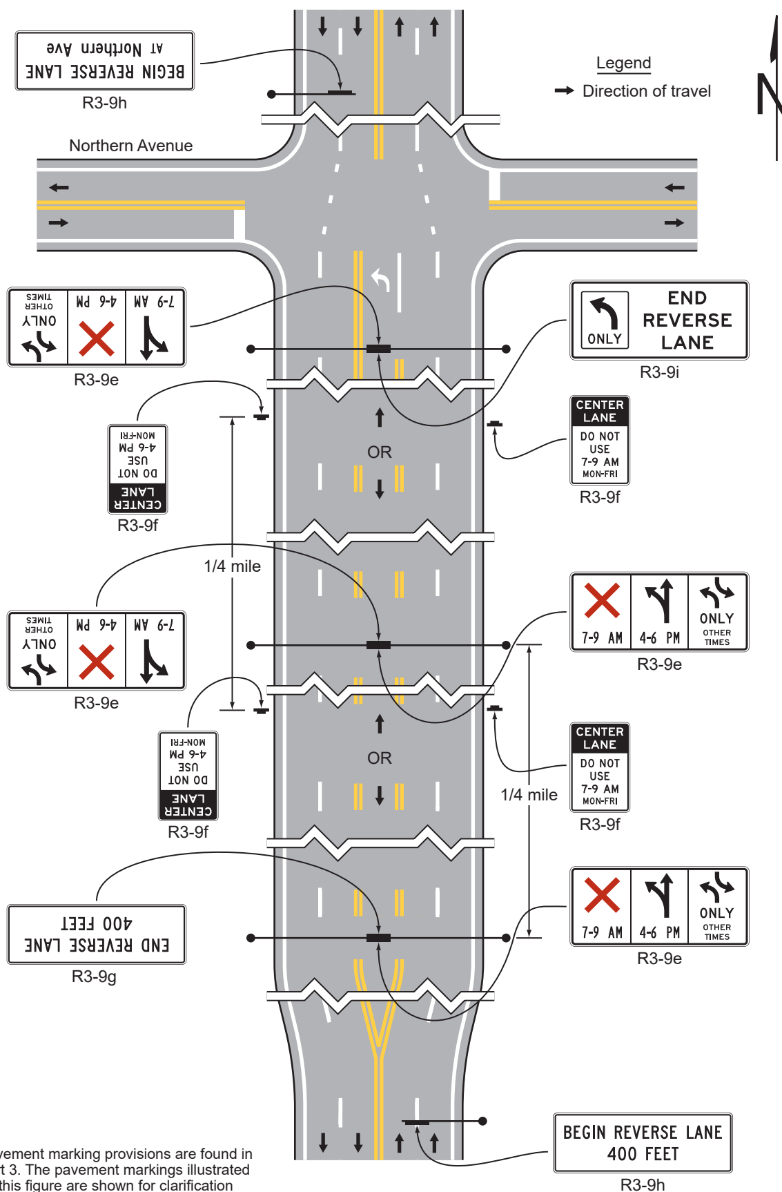
Figure 2B-7. Location of Reversible Two-Way Left-Turn Signs
