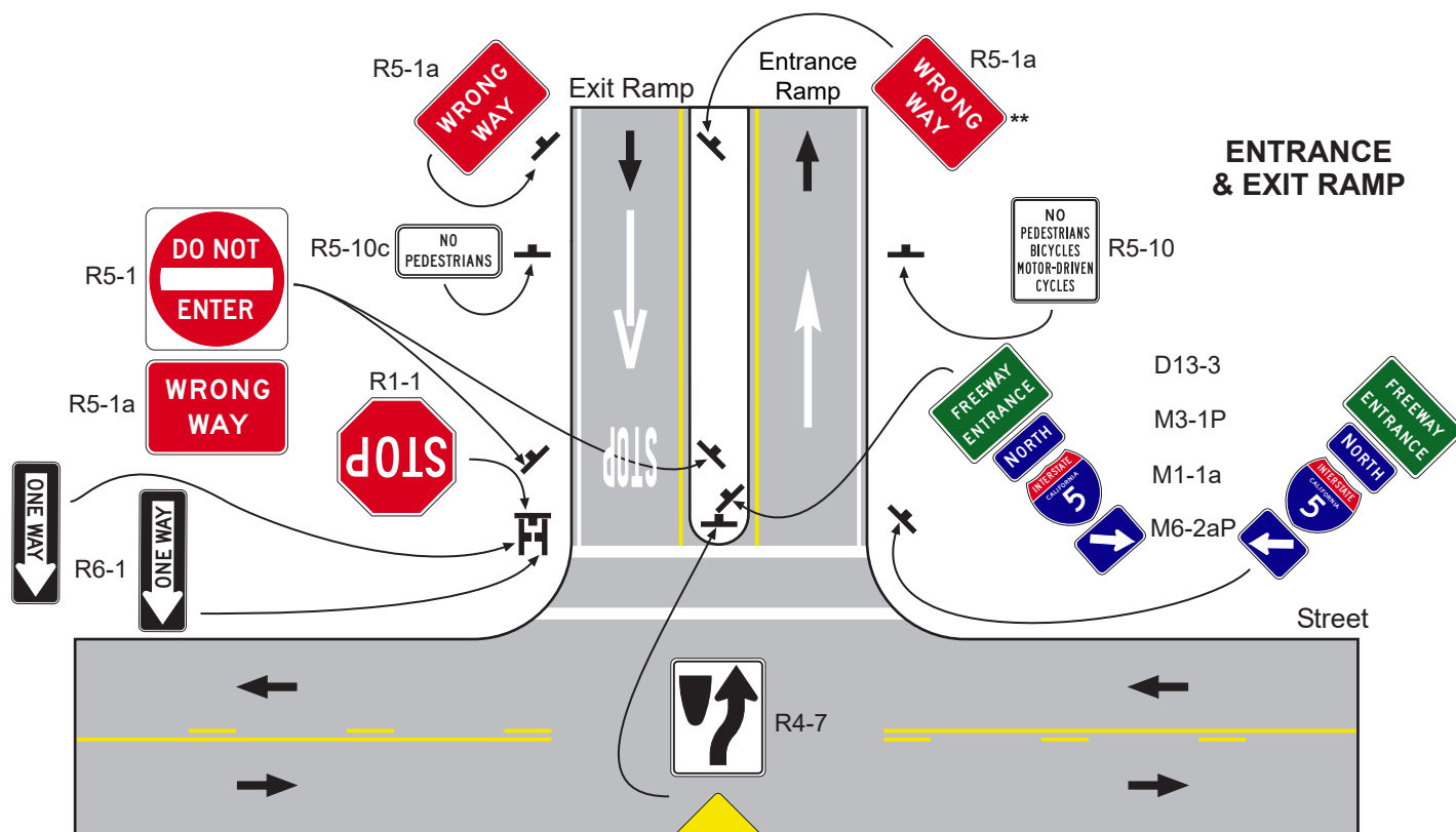
Figure 2B-15(CA). California Example of Application of Regulatory Signing and Pavement Markings at an Exit Ramp Termination to Deter Wrong-Way Entry (Sheet 4 of 5)
