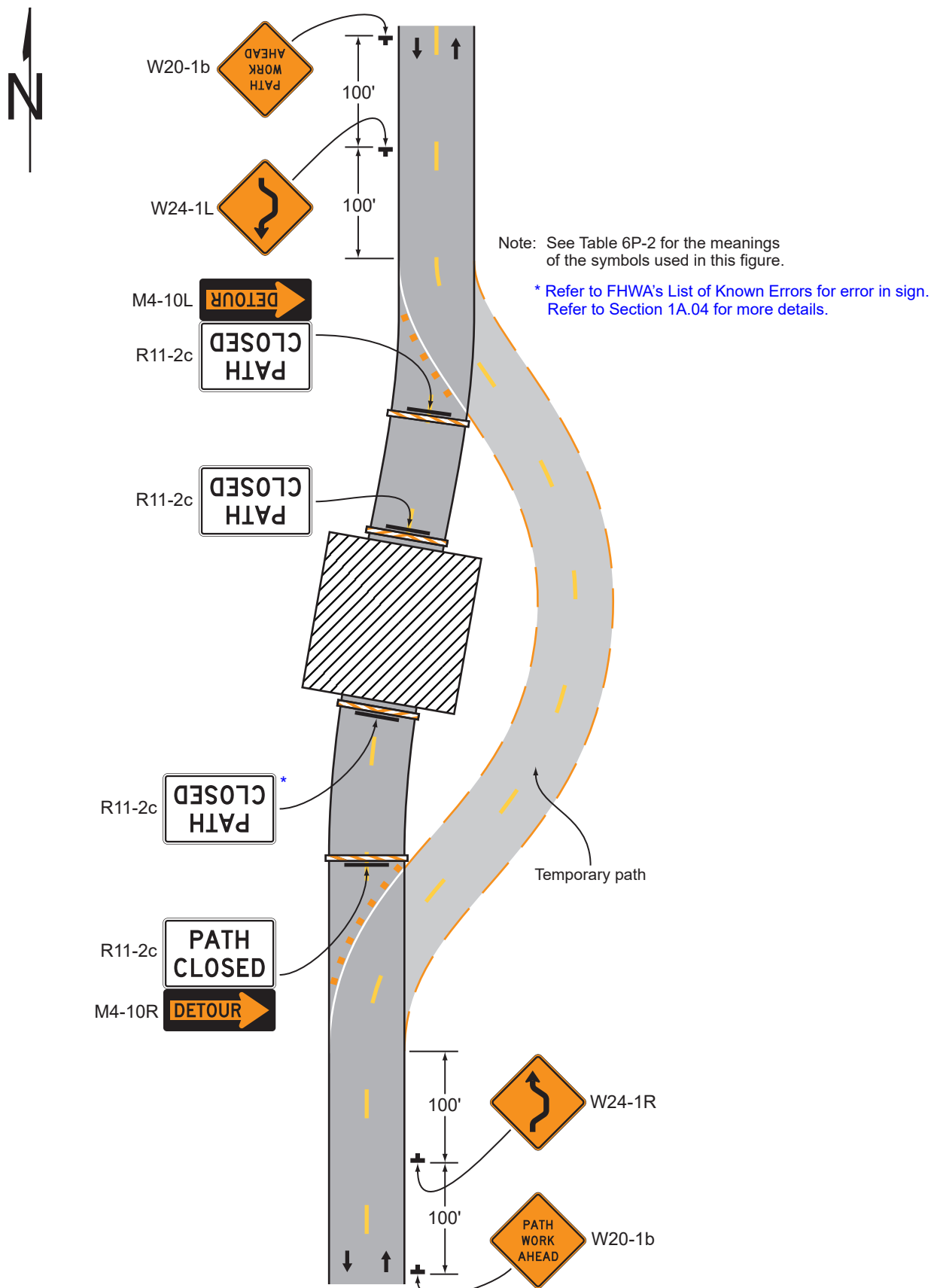
Typical Application 49
