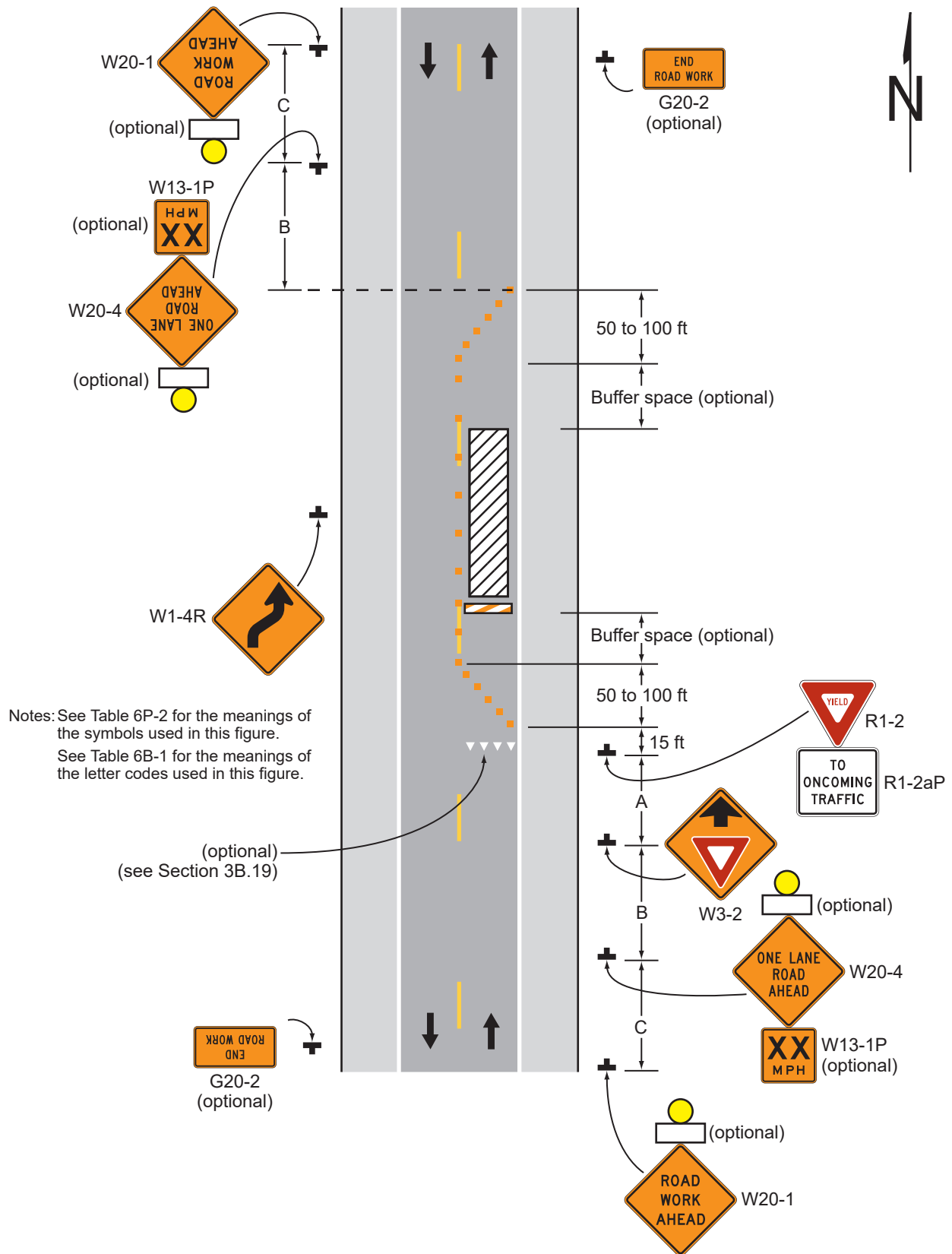
Typical Application 11
