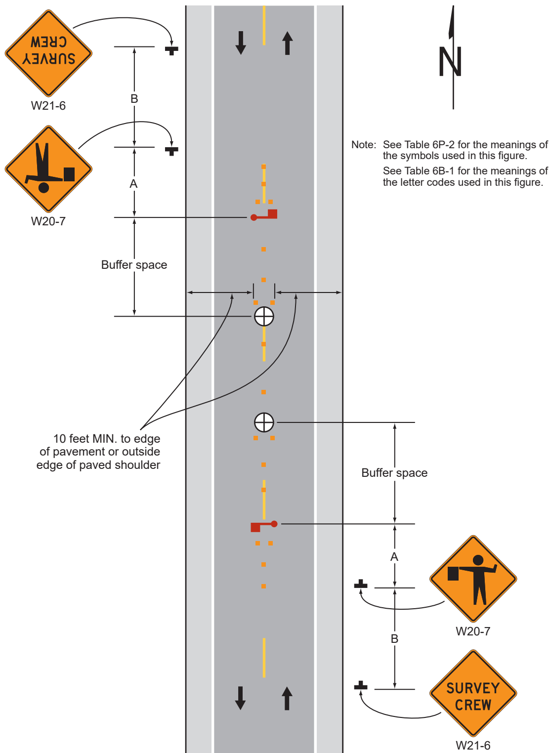
Typical Application 16
