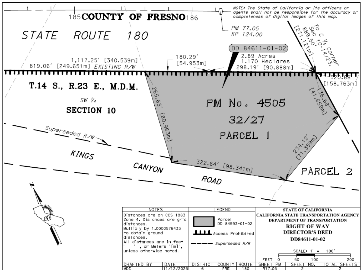
DD 84611-01-02 Detail Map
