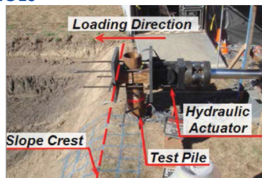
IMAGE 1: Test Setup
