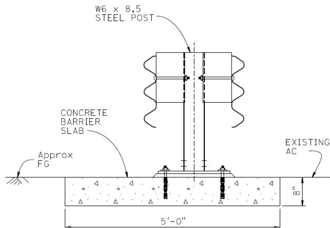
Image 4: Typical Section for Test Article
