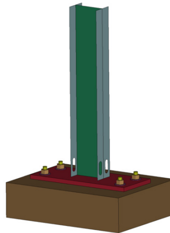
Image 1: Concrete Surface Mounted Median Post FEA Model
