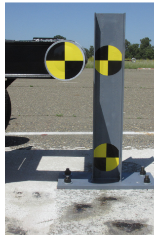
Image 2: Post Component Test Before Impact
