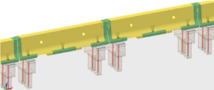
Image 2: Pooled Fund Example Project: Portable Temporary F Shape Concrete Barrier with vertical anchorage
