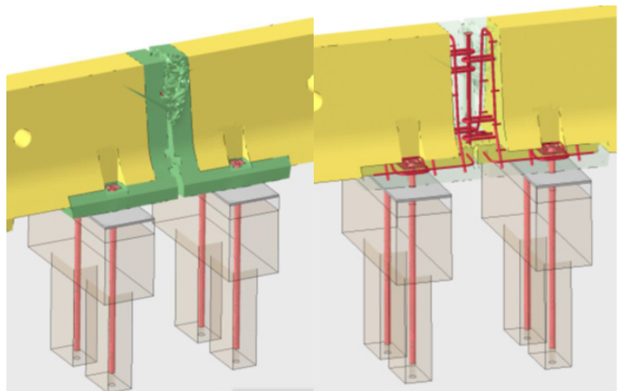
Image 5: Pooled Fund Example Project: Portable Temporary F Shape Concrete Barrier with vertical anchorage Finite Element Model and Simulation Results
