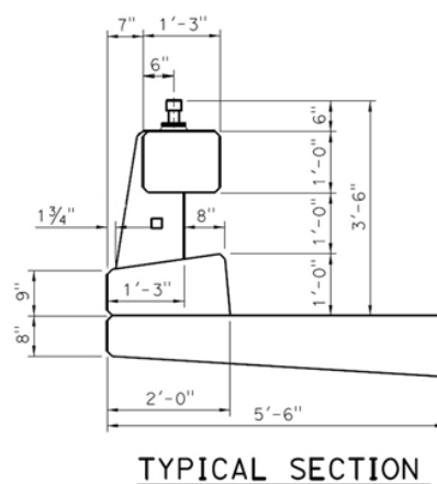
Image 1: Type 85 Bridge Rail Cross Section
