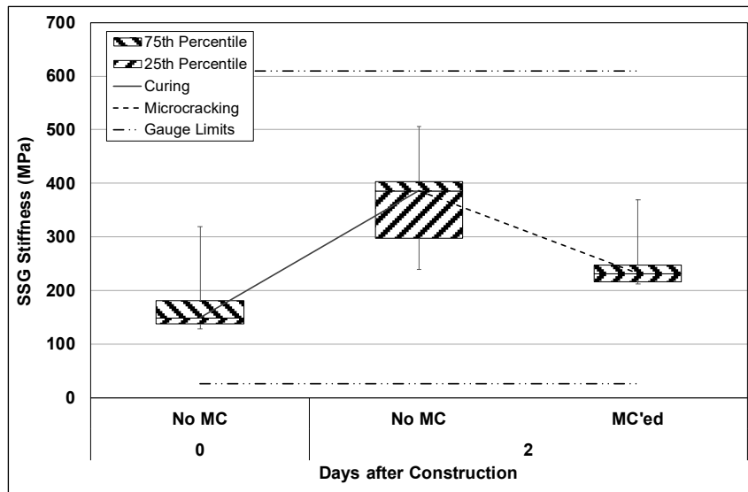
Figure B.230: Cell S31: SSG measured stiffness.
