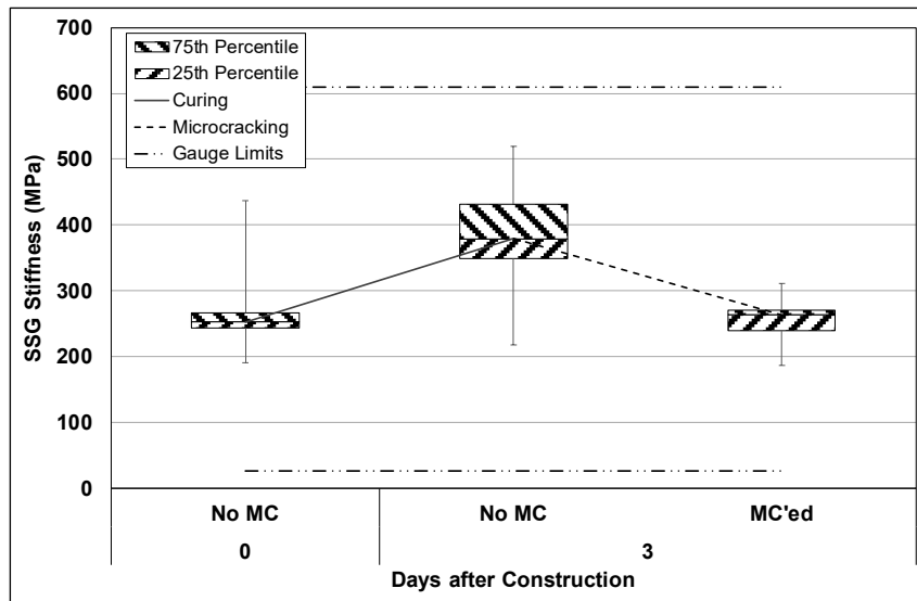
Figure B.83: Cell S11: SSG measured stiffness.
