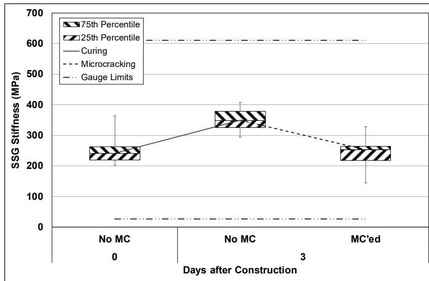
Figure B.140: Cell S18: SSG measured stiffness.
