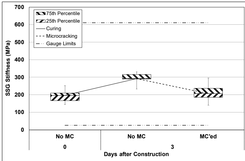
Figure B.215: Cell S29: SSG measured stiffness.
