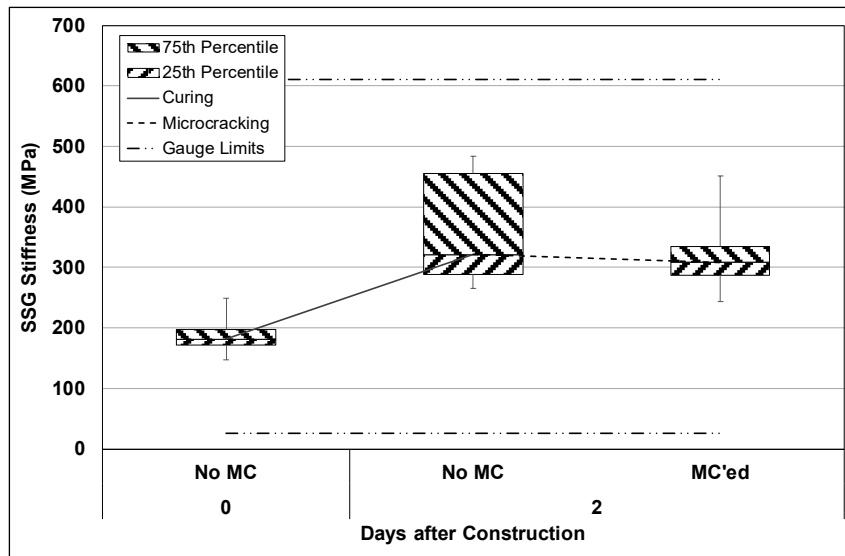
Figure B.92: Cell S12: SSG measured stiffness.
