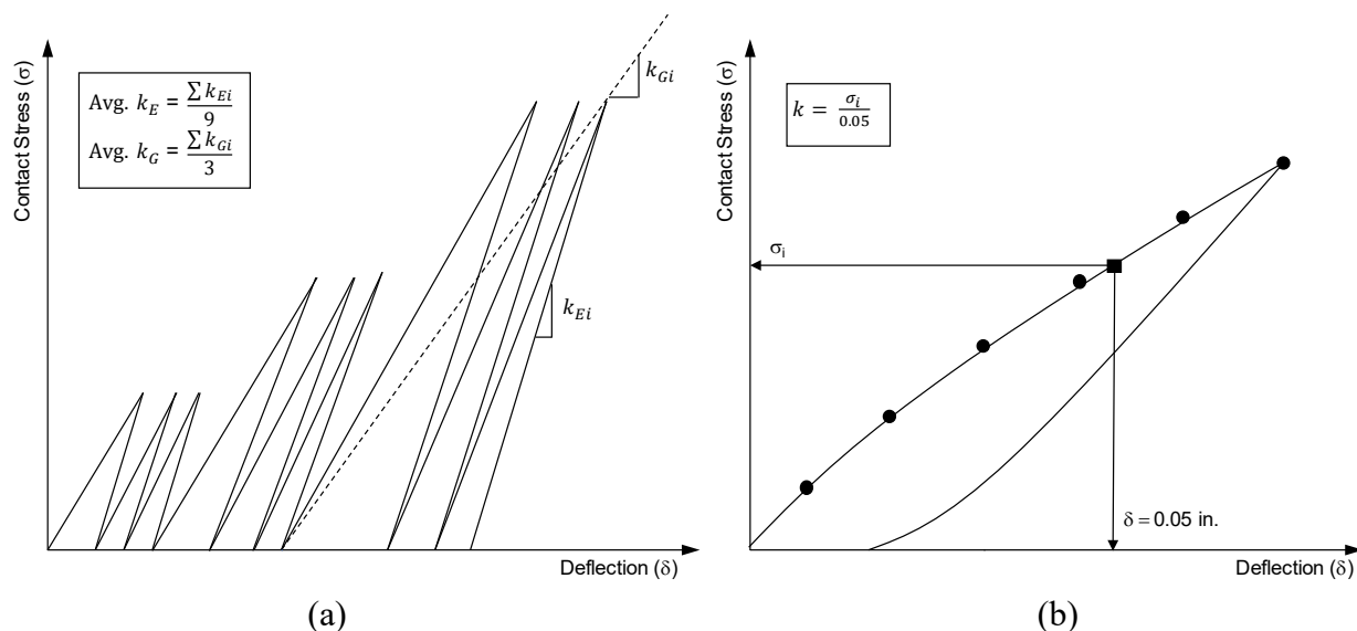
Figure 43. Interpretation of plate load testing results per (a) the AASHTO Road Test and AASHTO design procedures and (b) AASHTO and PCA design procedures
