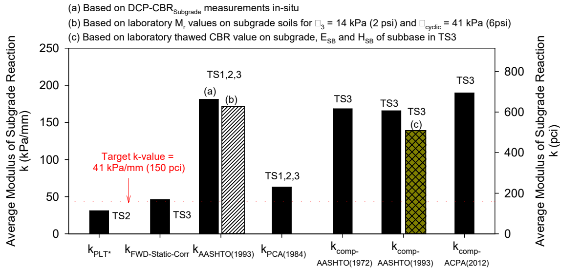
Figure 8. Which is the correct k value? Data compares the design target k value with measured and estimated k values from various field and laboratory measurements – Wisconsin US 10 construction project
