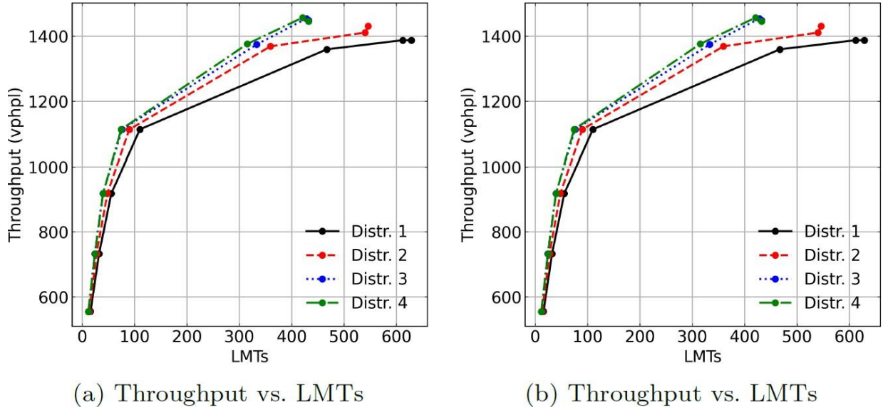
Figure 4.11: Throughput versus LMTs for different compliance distributions under MPR = 0%.
