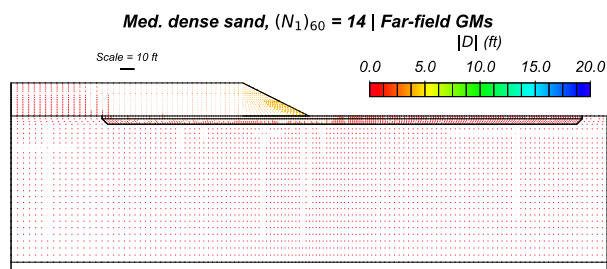
Figure 5: NDA results for Geometry 3 and Geometry 4: mean displacement magnitude.
