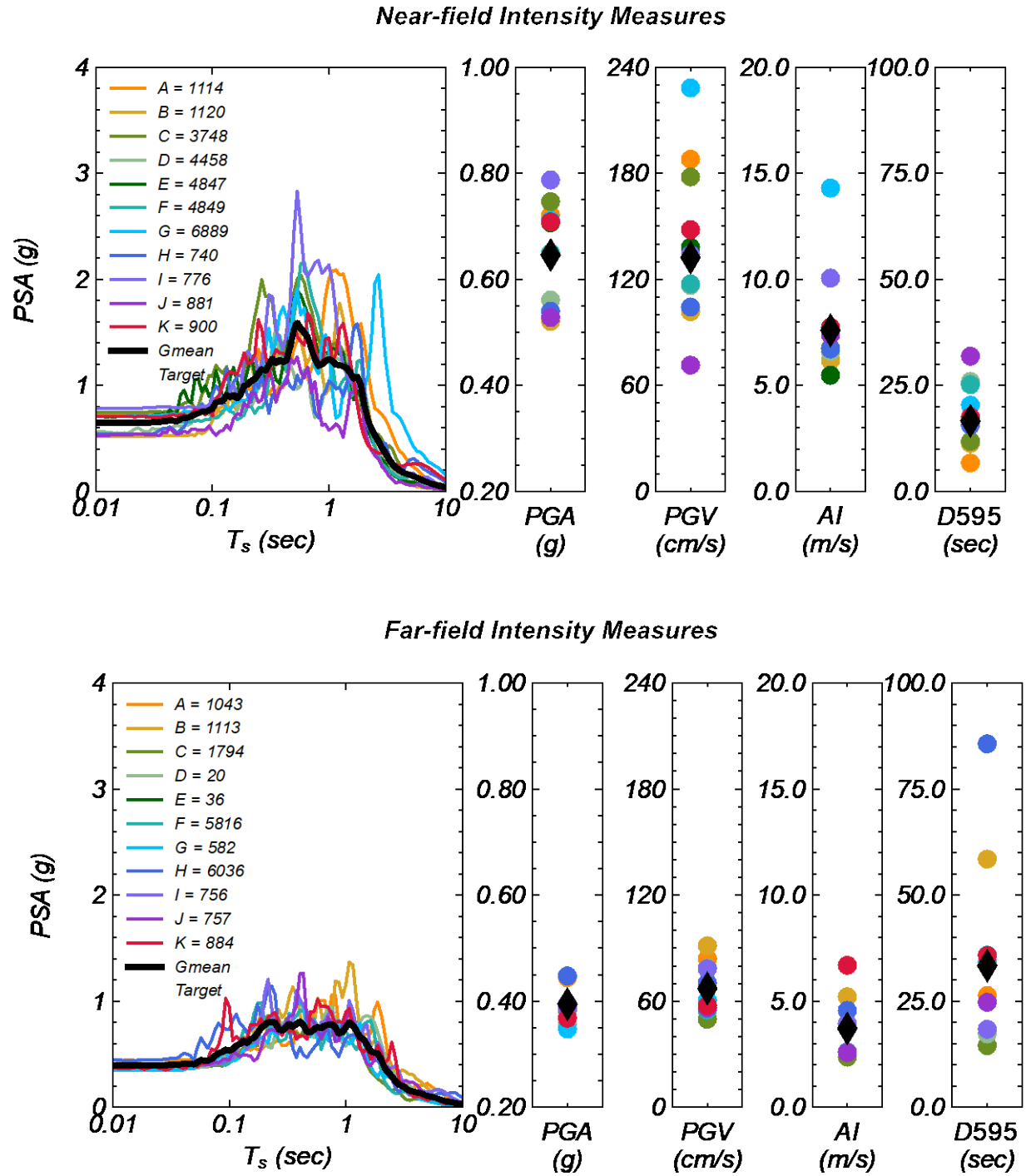
Figure 2: Intensity measures for near-field and far-field earthquake scenarios.
