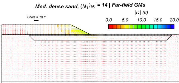
Figure 4: NDA results for Geometry 1 and Geometry 2: mean displacement magnitude.
