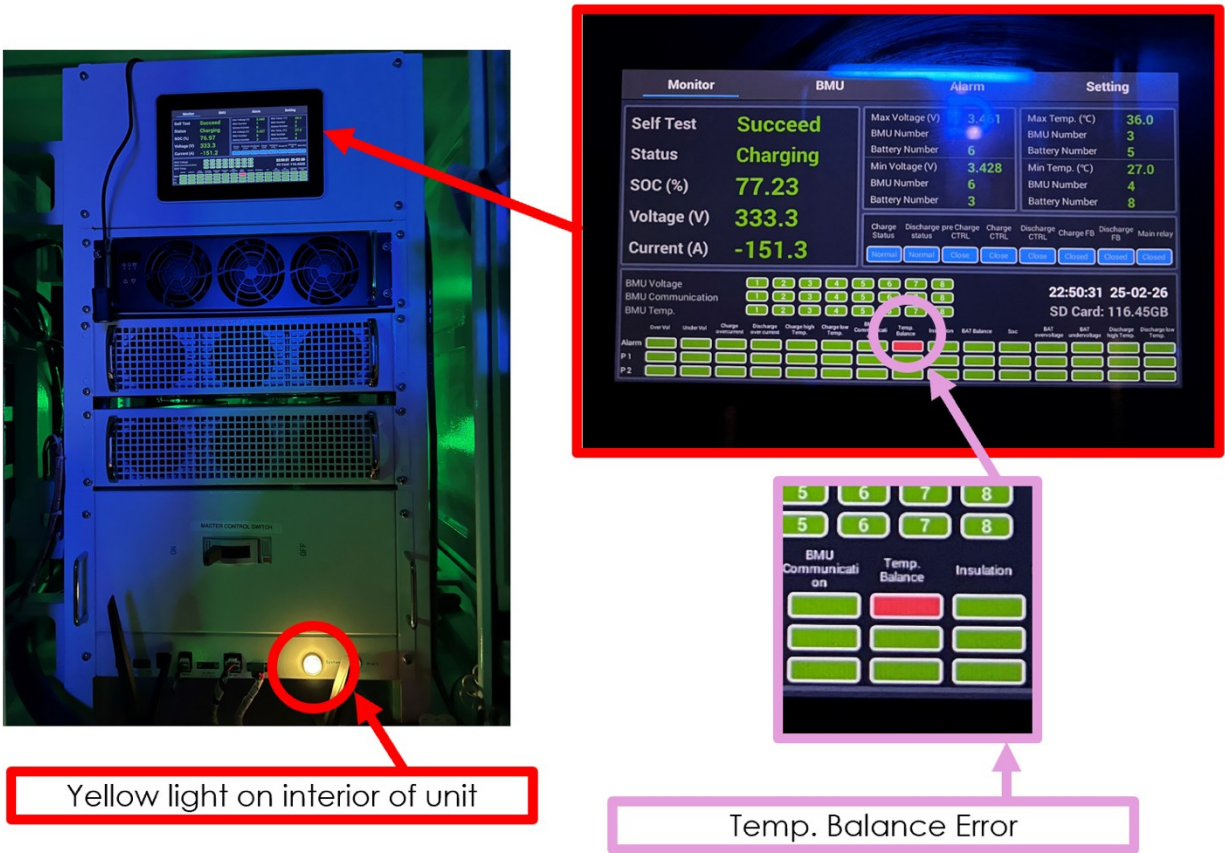
Figure 4.29: Temperature balance error seen on the EVES-6060-NA in cold conditions
