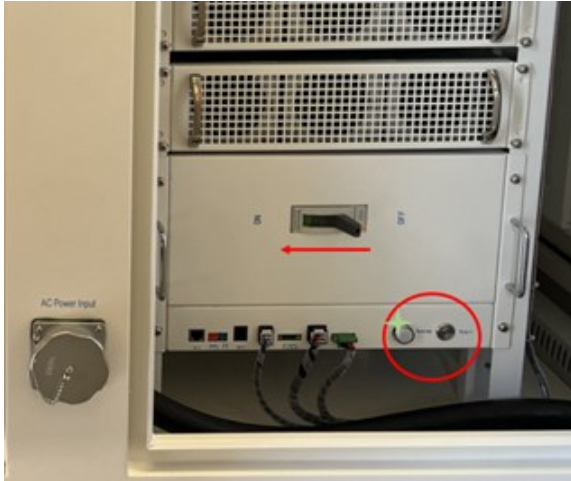
Figure B.8: START button activation and system status indicator for grid (AC) charging
