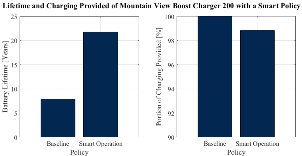
Figure 5.49: Battery expected lifetime assuming end-of-life at 20% capacity loss (left) and percentage of charging provided (right) based on the baseline and smart SOC policy used by the Mountain View FreeWire Boost Charger 200
