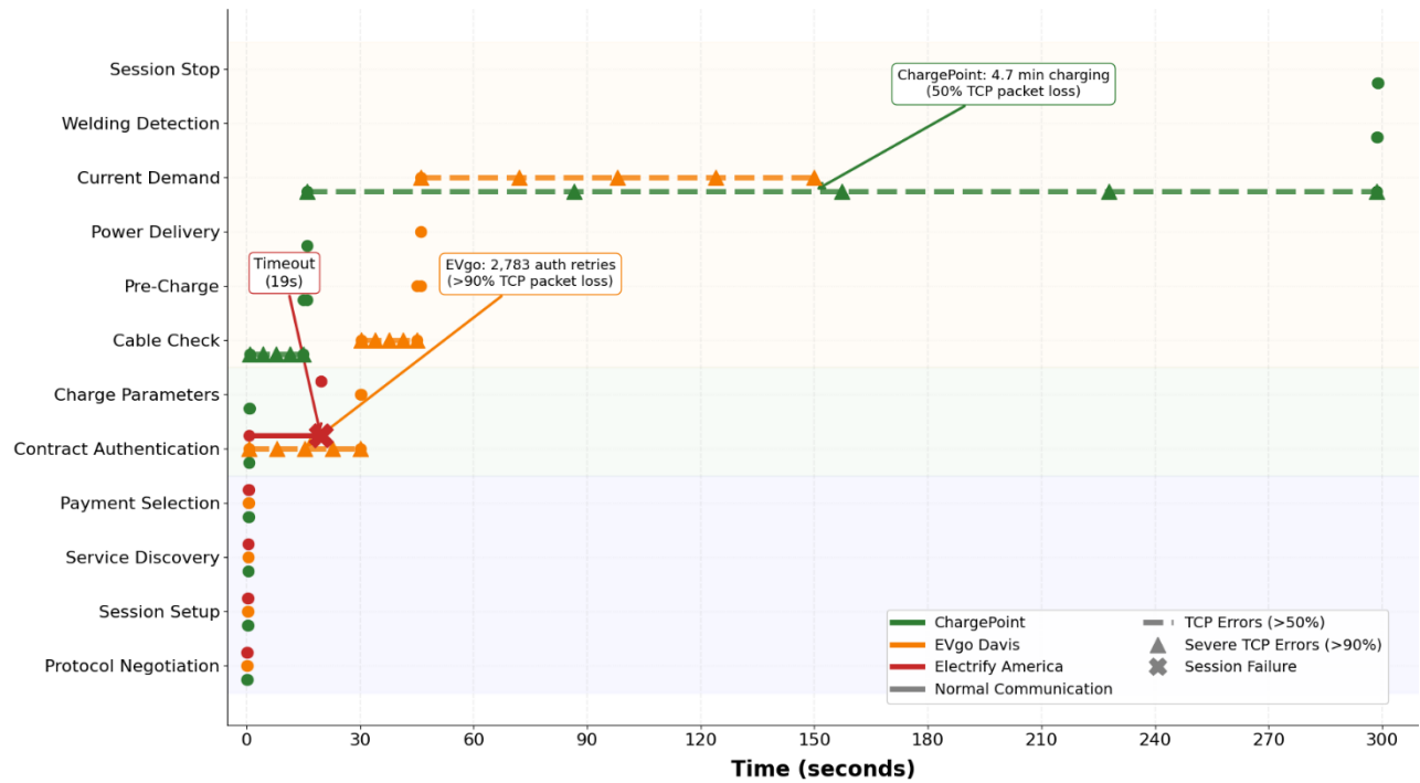
V2G Communication Phase Progression Comparison EVES-6060-NA at Different Charging Networks
