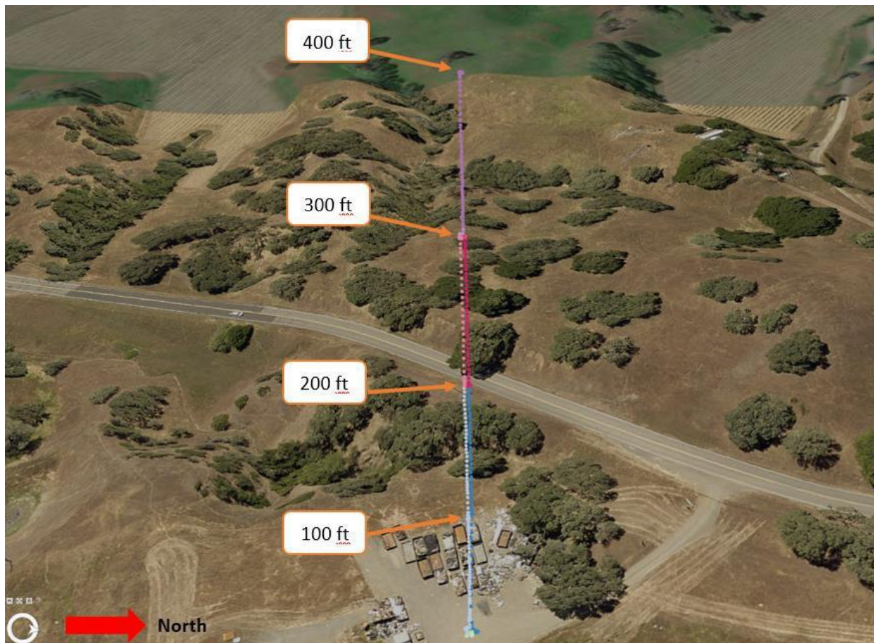
Figure 4.14: Flight path of UAS for Demo 5
