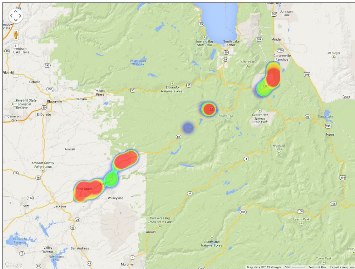
Figure E.6: SR88 ATT cellular service availability measurements (courtesy of AHMCT Research Center)
