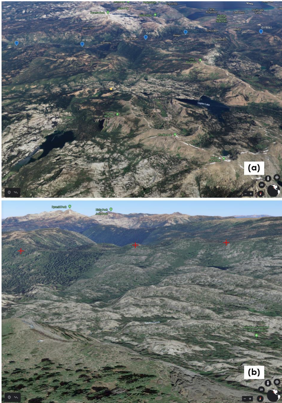
Figure E.5: SR88 3D map with select cellular tower and example site approximate locations near the Carson Spur (a) Verizon cellular tower and site locations, (b) view towards the cellular towers from the site (images courtesy Google Earth)
