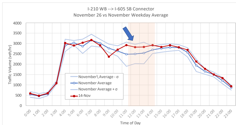
Figure 3-64 – Traffic Volume on the I-210 W to I-605 S Connector for the I-210 W November 26 Incident
