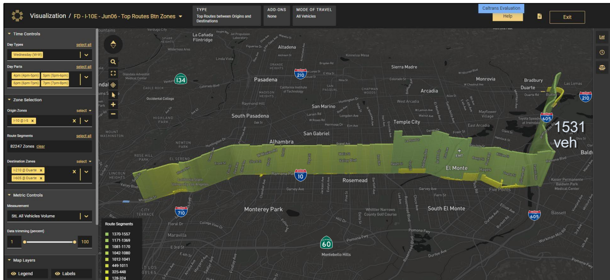
Figure 3-40 – Top routes between zones from I-10 E to I-210 E / I-605 N on Wednesday, June 5, 2019
