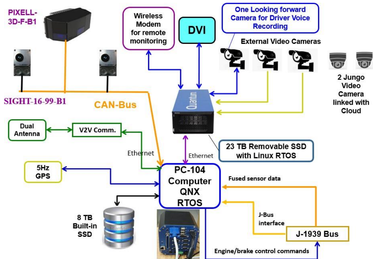
Figure 7. Data acquisition system installed on each truck: two large data drives are installed; one for CACC engineering data and one for extra sensor data
