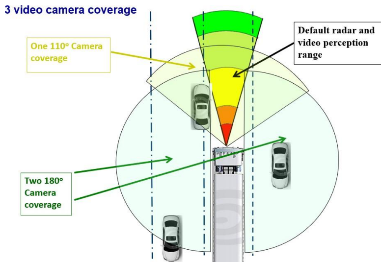
Figure 10. Three wide angle video camera coverage areas, mounted on the tractor only
