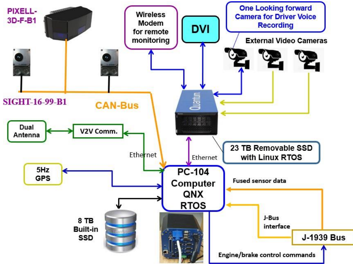
Figure 2. CACC Control System Architecture
