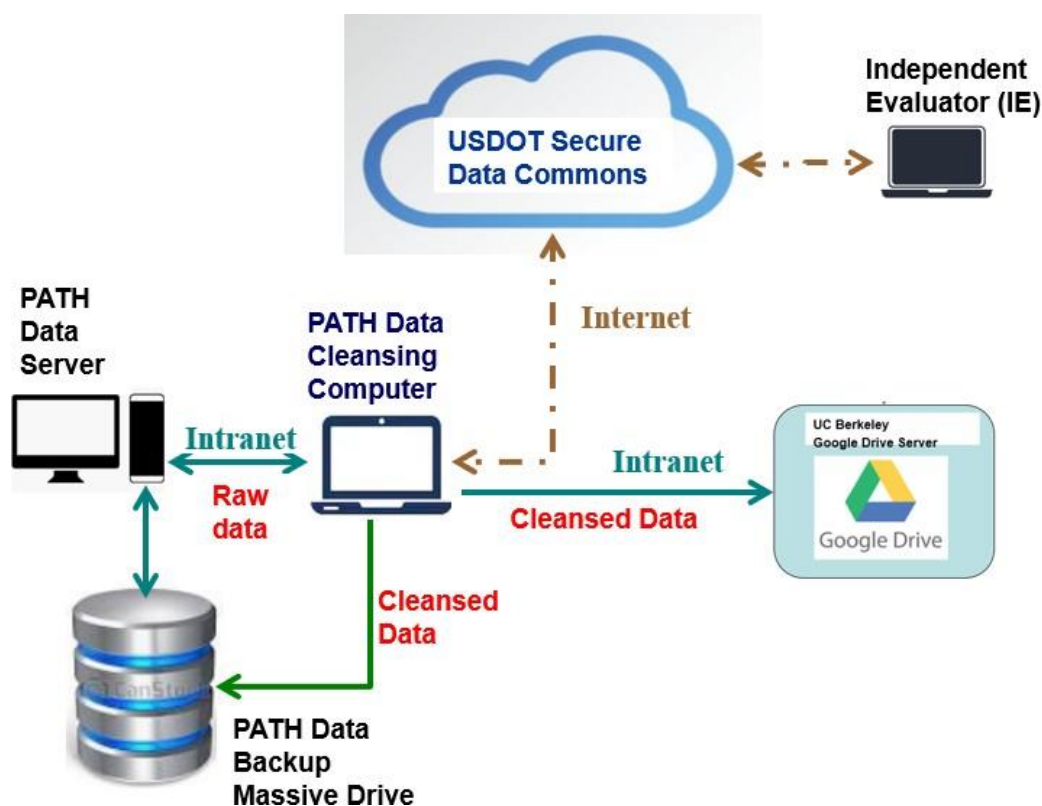
Figure 12. Scheme for Data Storage, Processing and Sharing with FHWA and IE
