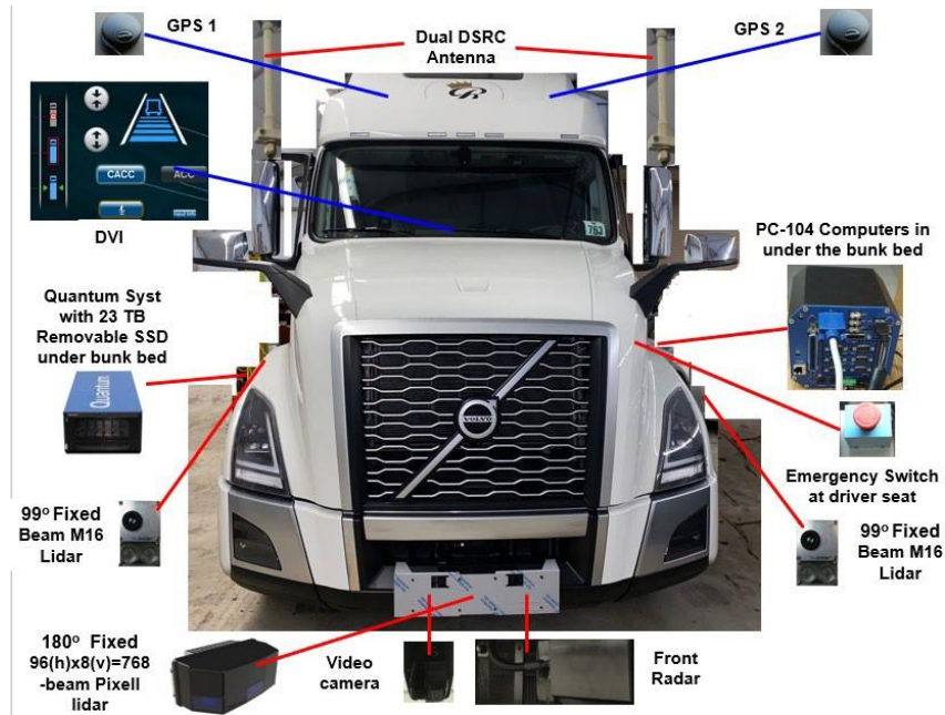
Figure 1. CACC Truck System Hardware
