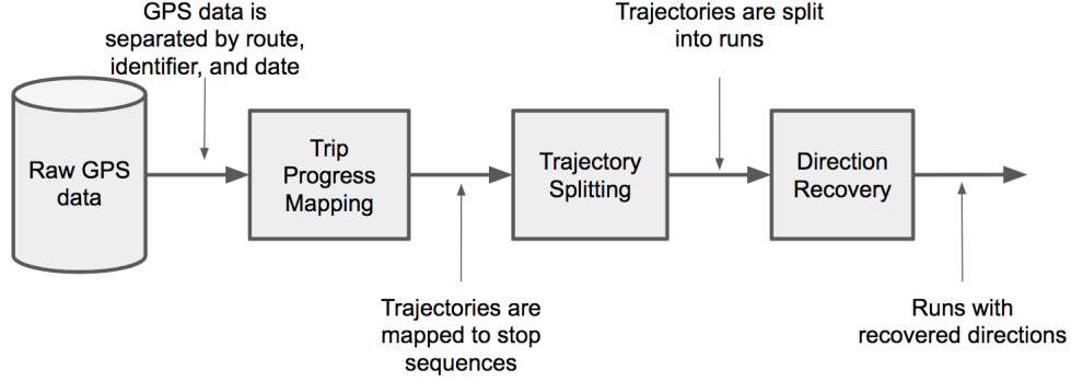
Figure 3: Pre-processing steps
